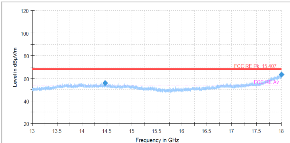
Lowest channel : 13 GHz to 18 GHz_Peak
