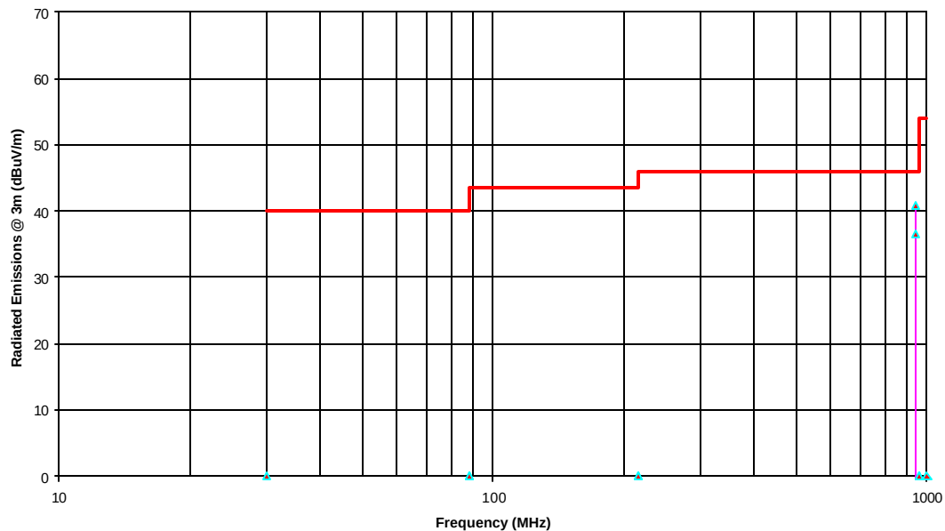
Radiated Emissions Measurements @ 3m OFTS FCC Part 15, Sub. B & ICES-003 - Class B Digital Devices Sanyo 900 MHz Cordless Phone, Model CTL-9935N
