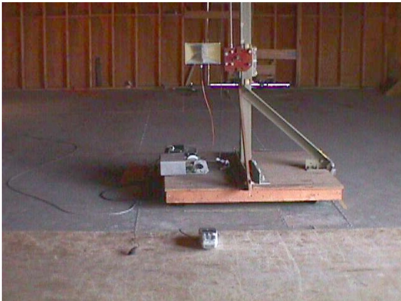
Radiated Emissions at 3 M Handset – Orthogonal Position #3
