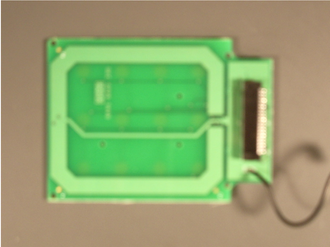
Antenna PCB – Antenna Side
