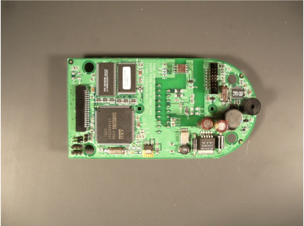
Main PCB – Top
