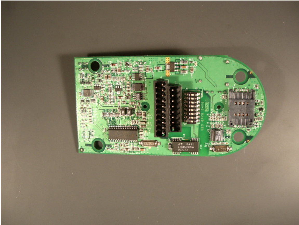
Main PCB – Bottom
