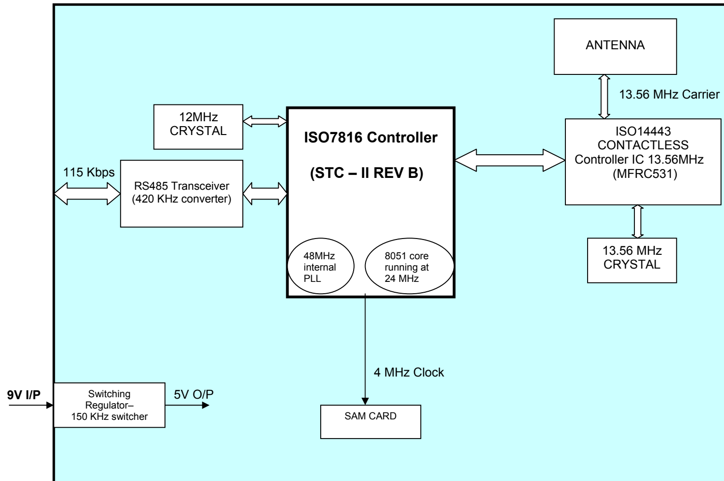
PAT 1221 Reader Block Diagram
