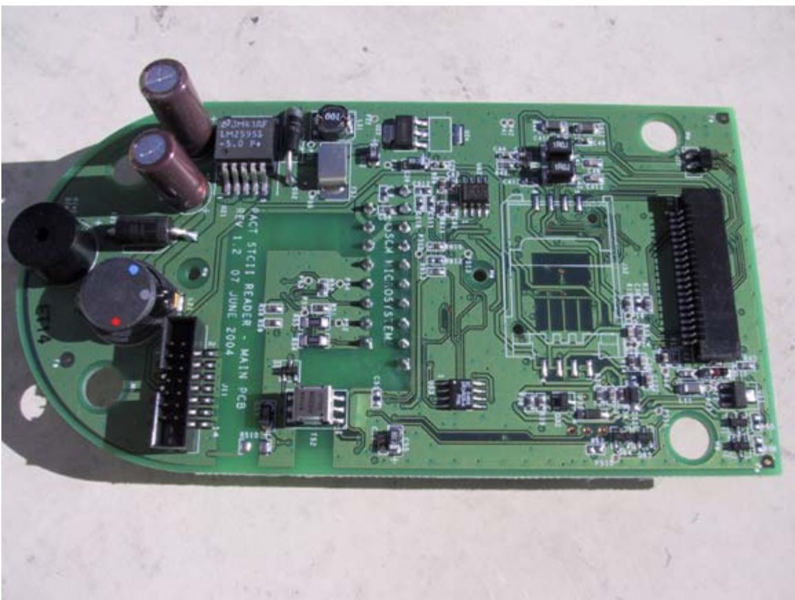
Photograph 6. EUT Internal Photo – Main PCB
