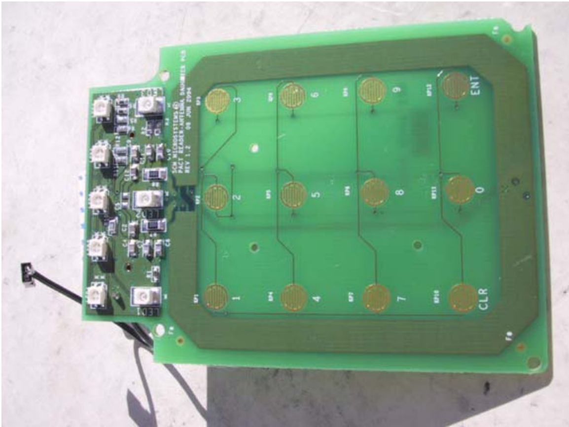
Photograph 2. EUT Internal Photo – Keypad PCB
