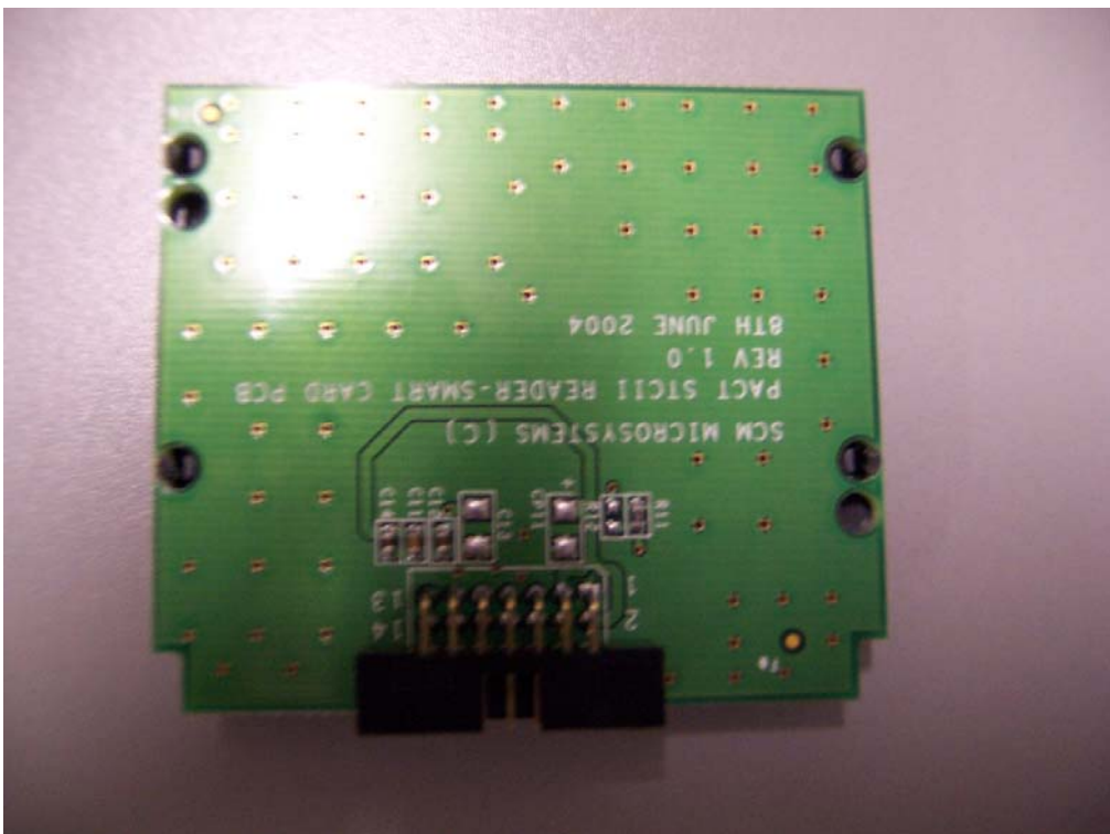
Photograph 4. EUT Internal Photo - Card Slot PCB
