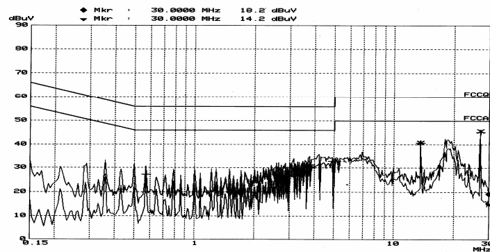
Line N Conducted Emission Graph
