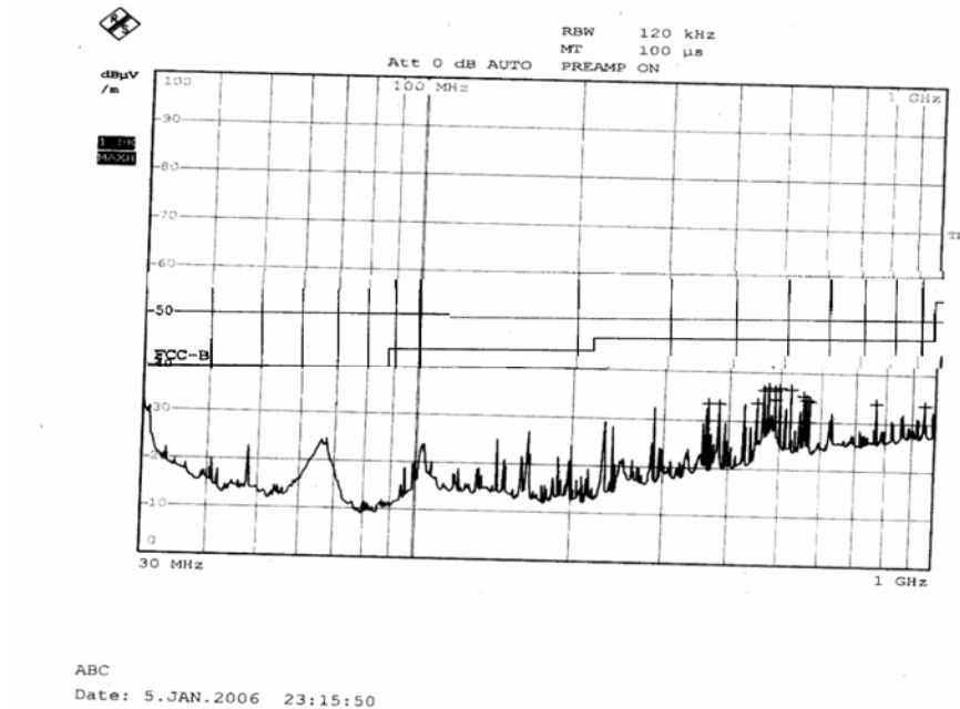
Horizontal Radiated Emission Plot
