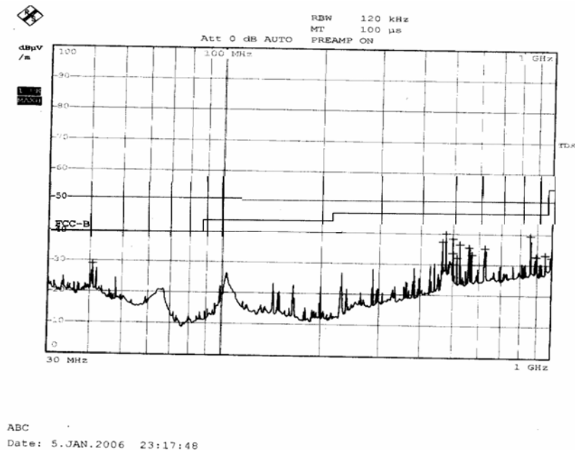
Vertical Radiated Emission Plot
