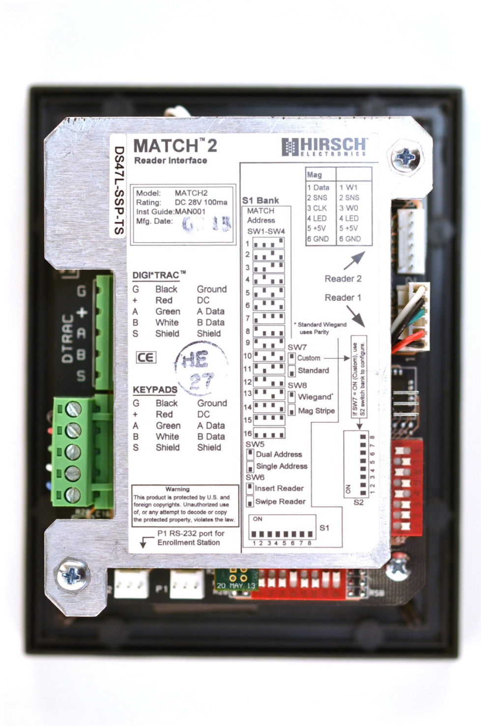
EUT Rear View
