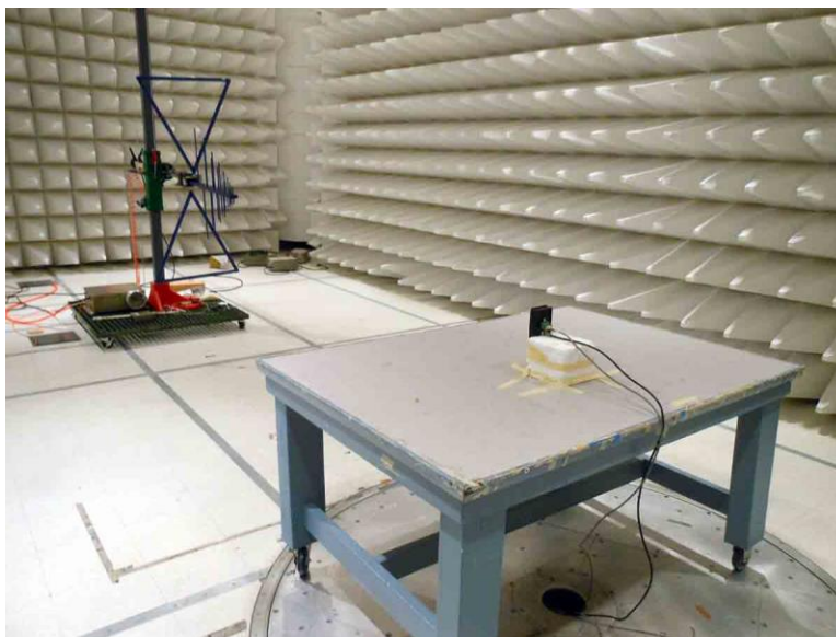
POE, 30MHz-1GHz
