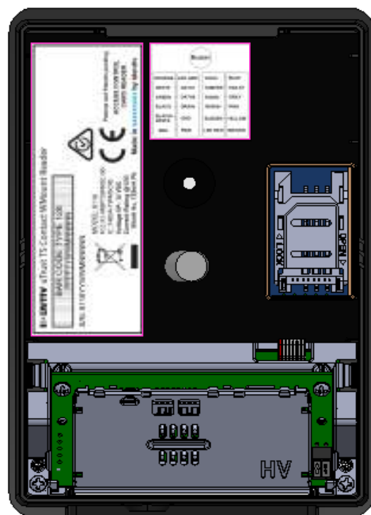
Reader with Pigtail cable
