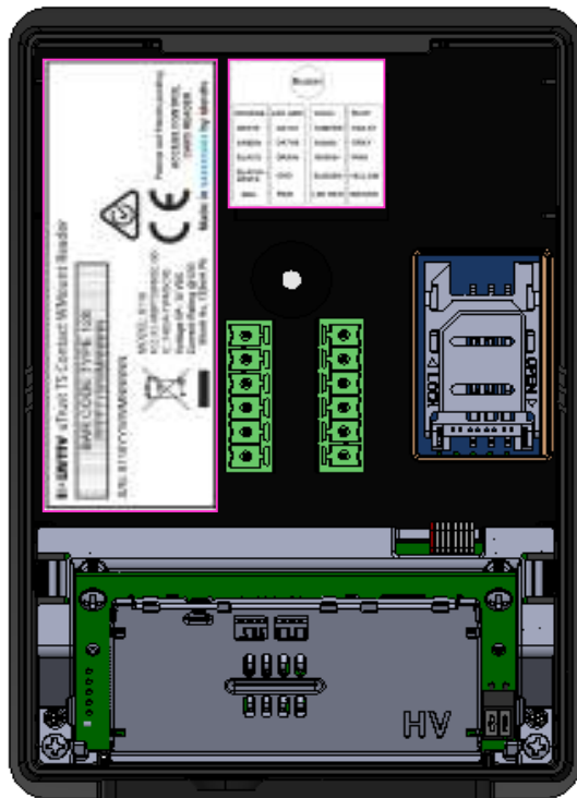
Reader with Terminal connector
