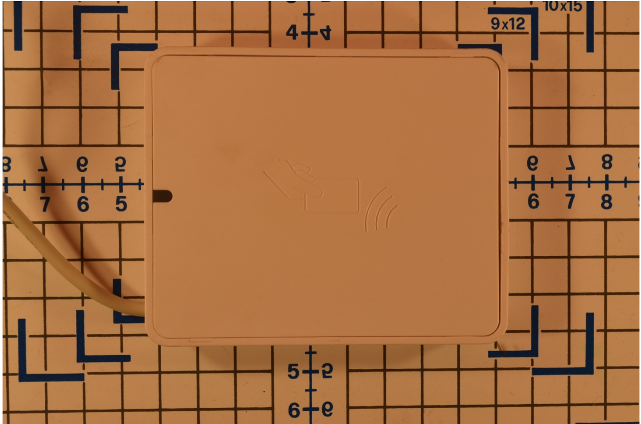
EUT Bottom View
