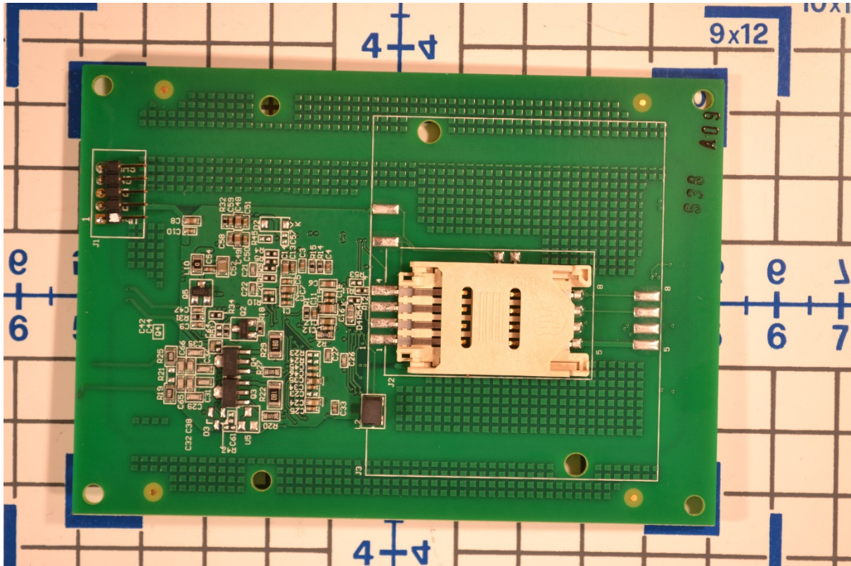
PCB: Top View
