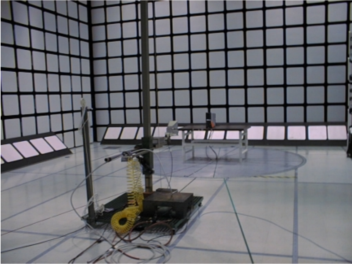
MPE and Radiated Spurious Emissions
