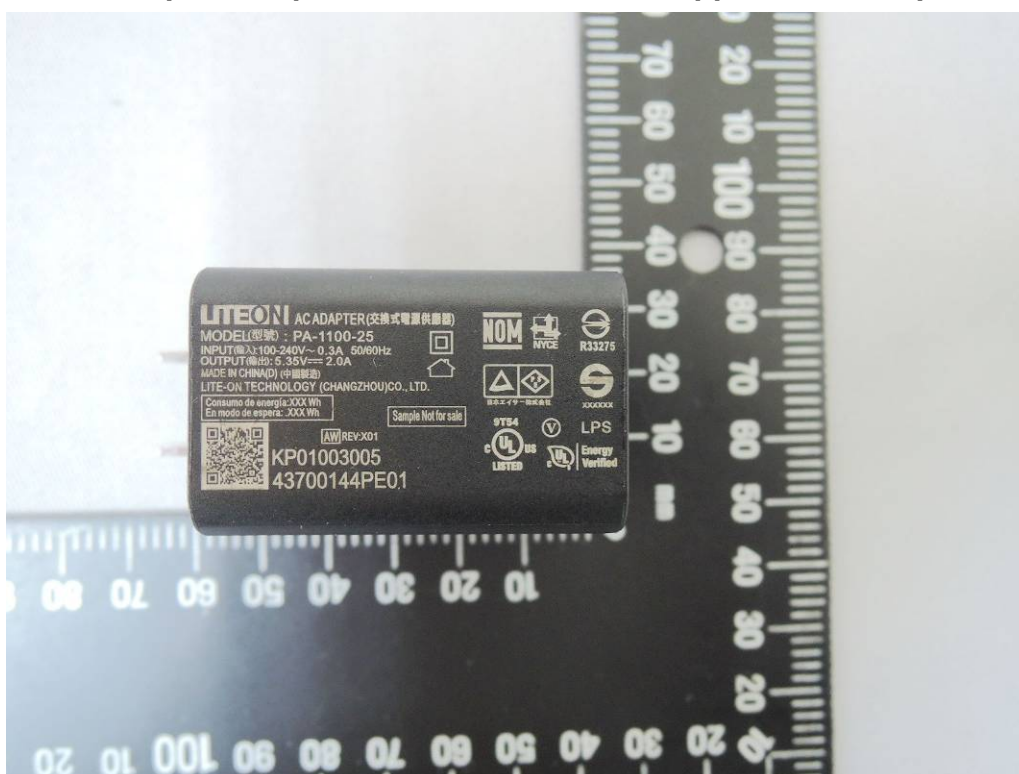
Adapter – 1 (Model No.: PA-1100-25, Supplier: LITEON)
