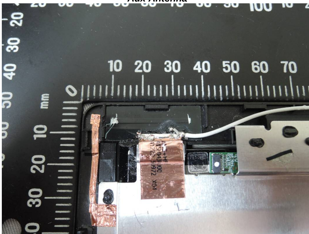
Aux Antenna
