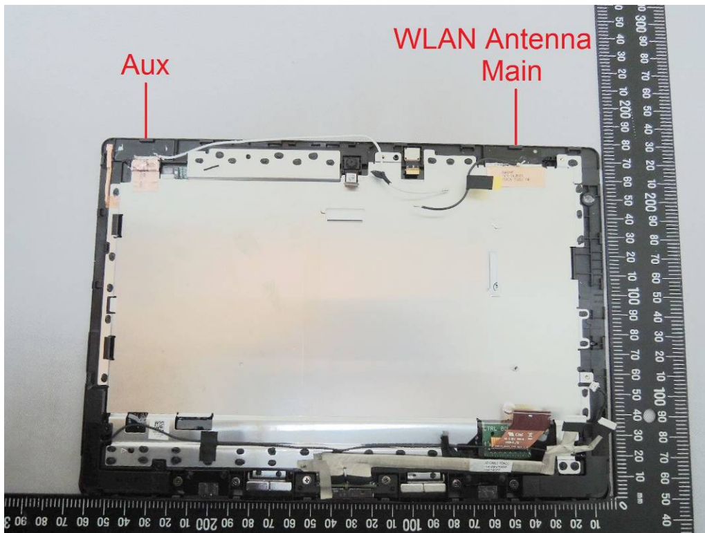
BT/WLAN Antenna
