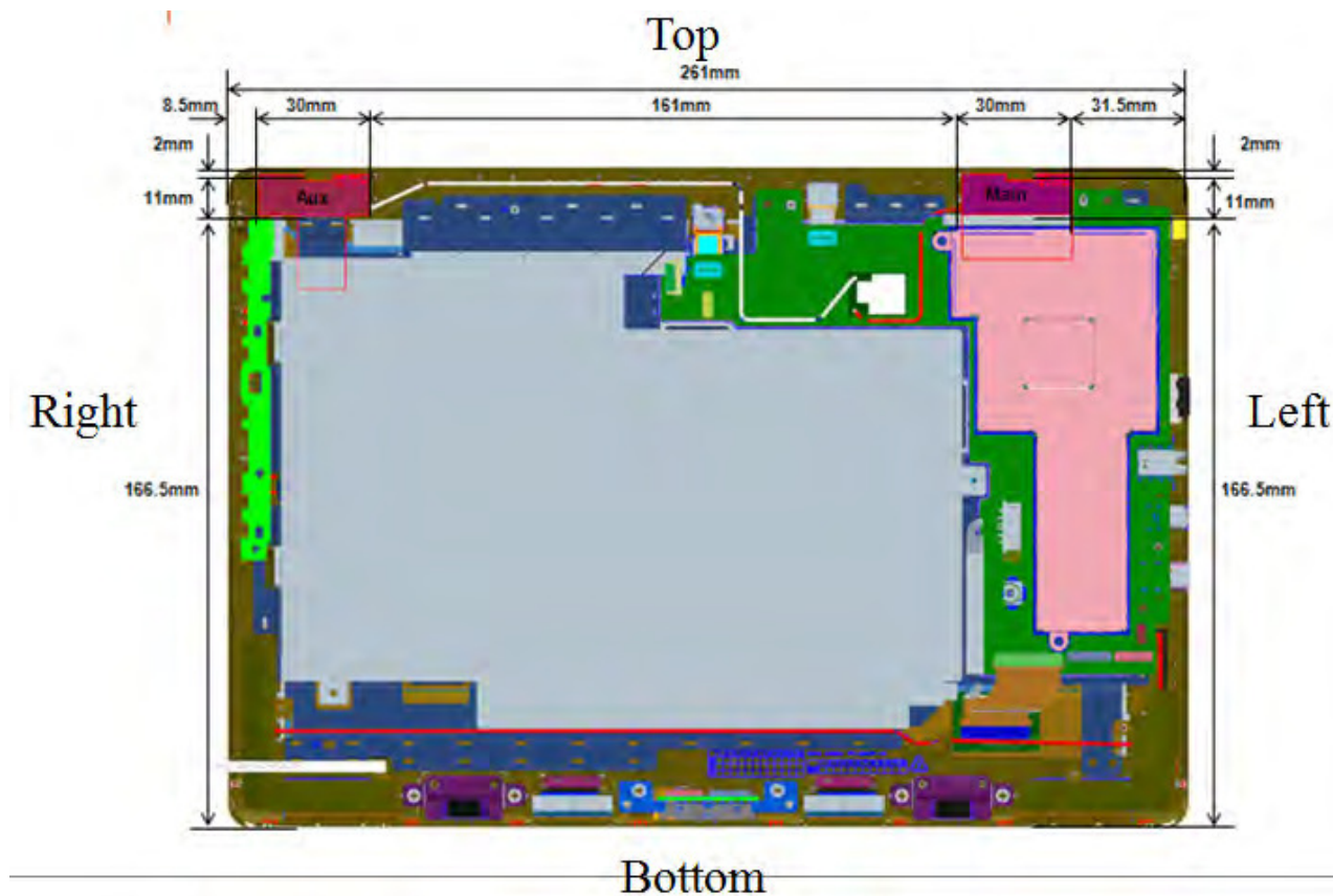
Fig.8 Antenna position of EUT (Back view)
