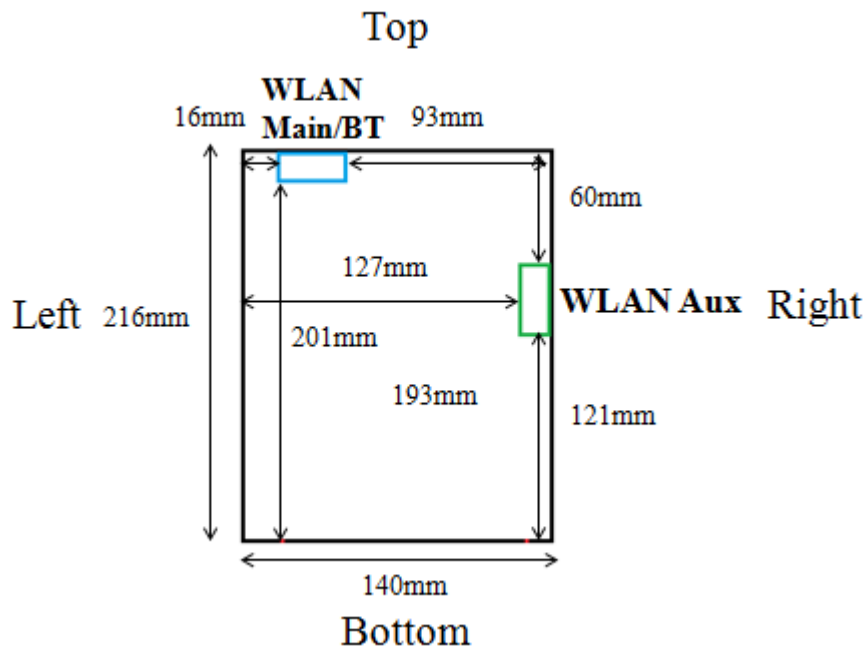
Fig.10 Antenna position of EUT (Front view)
