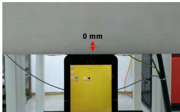
Fig.6 EUT Right side to flat phantom
