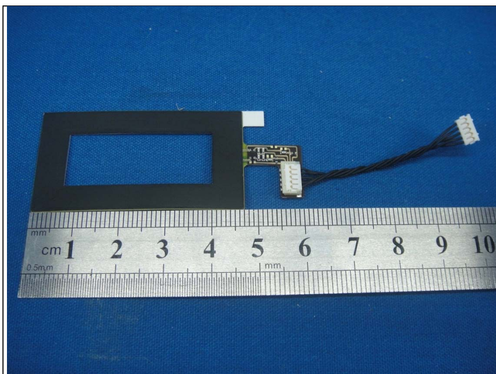
Antenna 5 (Model: LX7828-12-000-C)
