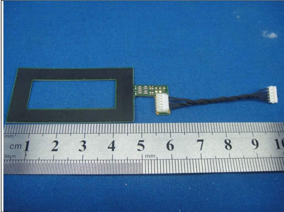
Antenna 2 (Model: ANT-MO41A)
