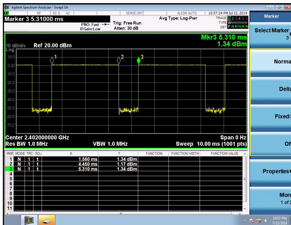
Time-domain plot for Bluetooth transmission signal
