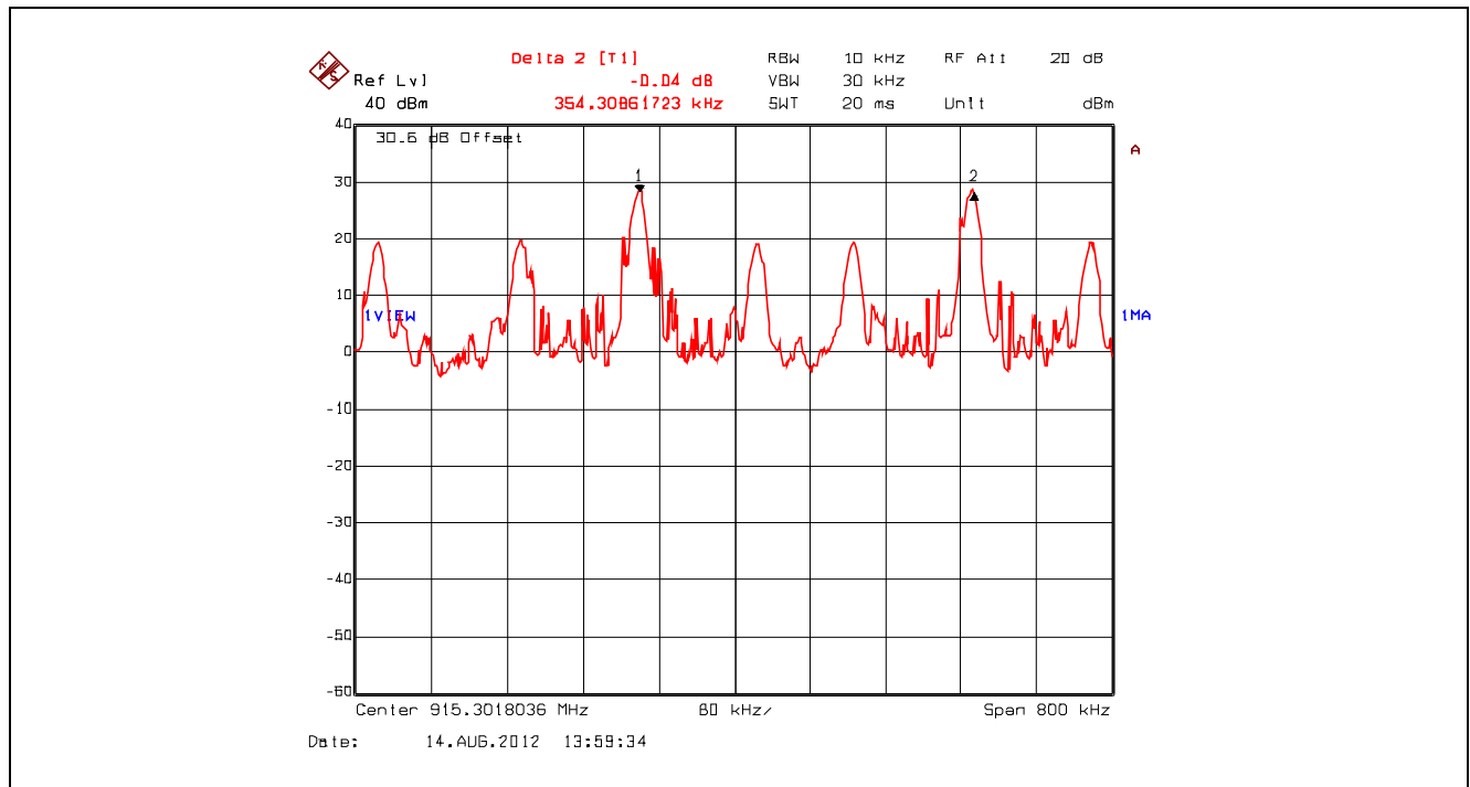
Plot 5.3.4.8. Carrier Frequency Separation, GFSK, 125 kbps
