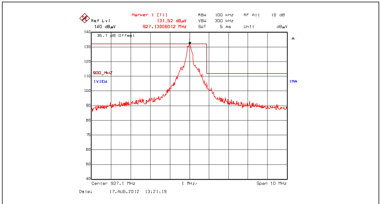
Plot 5.7.4.4.2.7. Radiated Band-Edge, High End of Frequency Band, Single Frequency Mode, High Power, Vertical
