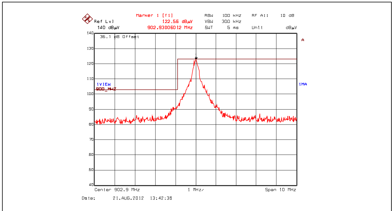
Plot 5.7.4.2.2.3. Radiated Band-Edge, Low End of Frequency Band, Single Frequency Mode, High Power, Vertical
