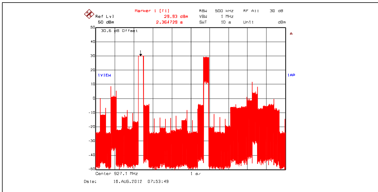
Plot 5.3.4.26. Time of Occupancy, 927.1 MHz, FSK 10 kbps, Dwell Time @ 927.1 MHz = 285.561122 ms
