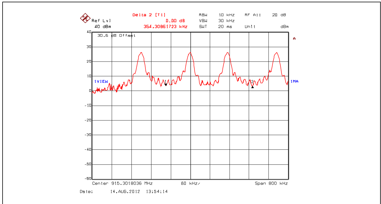
Plot 5.3.4.7. Carrier Frequency Separation, FSK, 10 kbps
