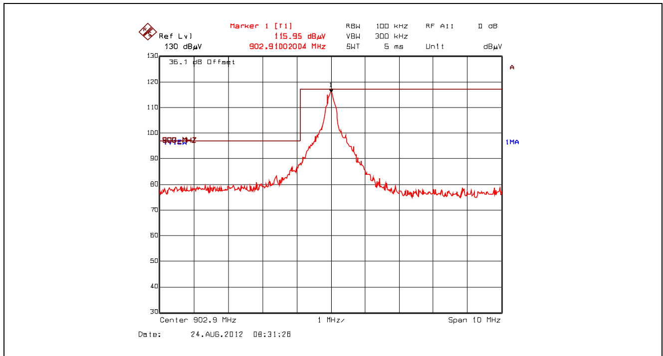
Plot 5.7.4.1.2.3. Radiated Band-Edge, Low End of Frequency Band, Single Frequency Mode, 100 mW, Vertical
