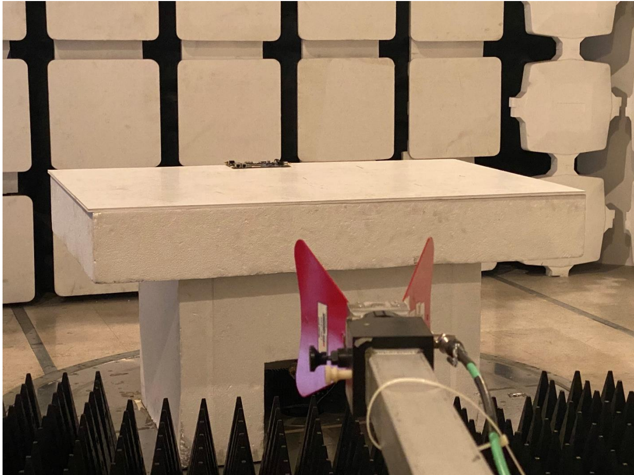
Radiated Emissions 1-6GHz
