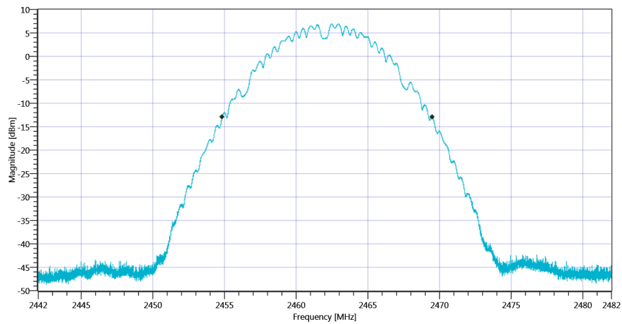
Plot_FCC Part 15.247 Bandwidth 99PCT-20dB ~ WLAN2G4 b-mode_14102020_105859.png
