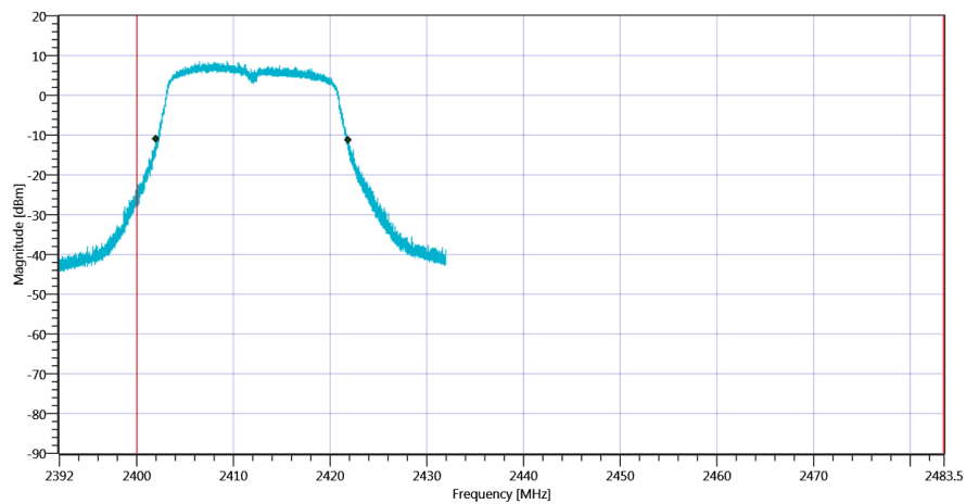
Plot_FCC Part 15.247 Bandwidth 99PCT-20dB ~ WLAN2G4 nHT20-mode_15102020_084230.png
