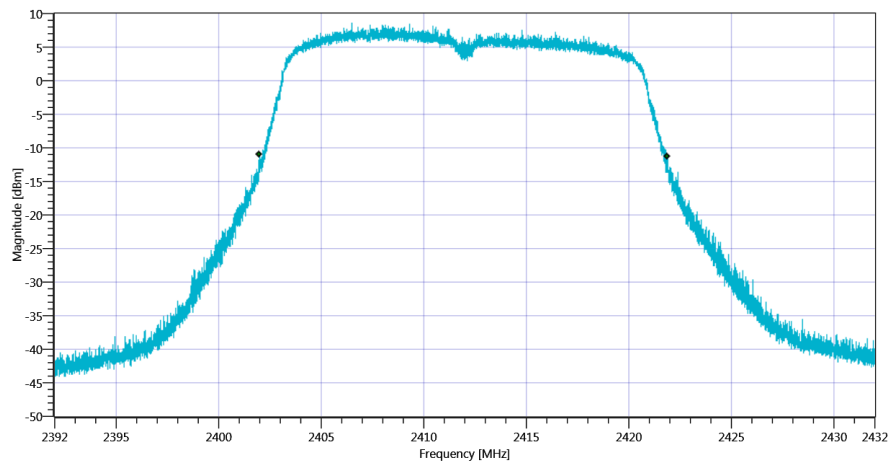
Plot_FCC Part 15.247 Bandwidth 99PCT-20dB ~ WLAN2G4 nHT20-mode 20dB_15102020_084226.png
