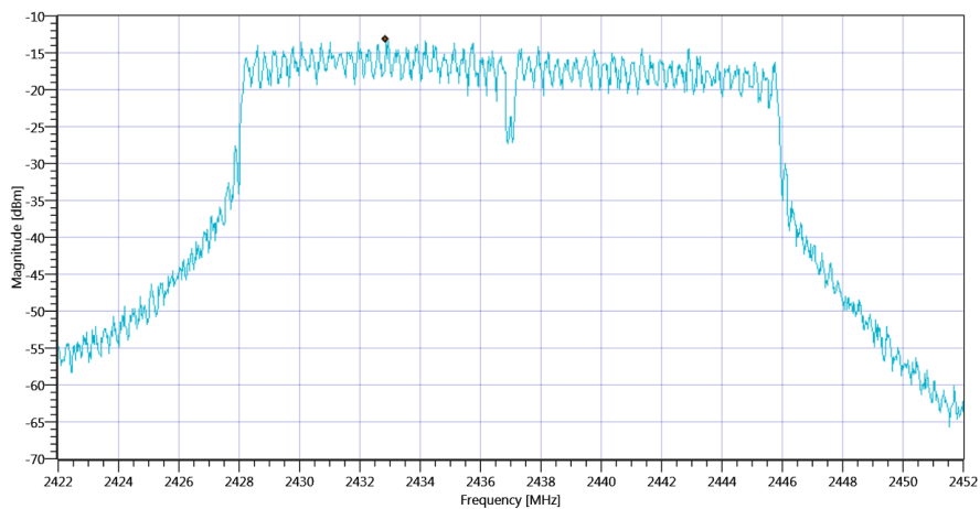
Plot_FCC Part 15.247 Peak Power Spectral Density DTS ~ WLAN2G4 nHT20-mode_15102020_085056.png
