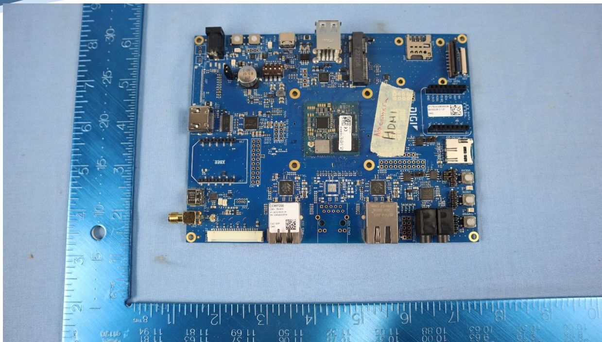
CCMP25 Front
