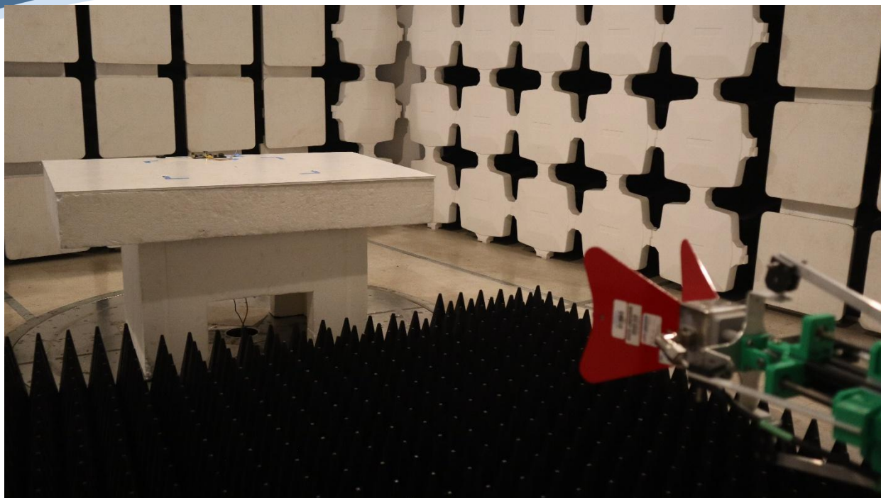
Radiated emissions above 1GHz Test Setup
