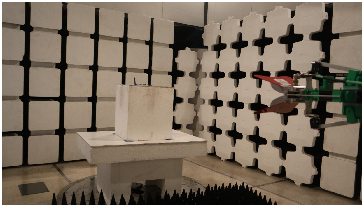
Test Setup 1GHz-18GHz GW.49.A153
