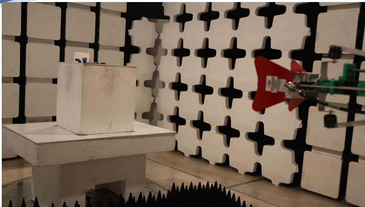
Test Setup 1GHz-18GHz H2B1WD1A3B0200
