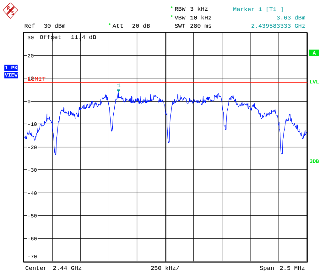
Plot 5.6.4.2. Power Spectral Density, Channel 18, 2440 MHz, QPSK Modulation, Power Setting -7 Mode 3
