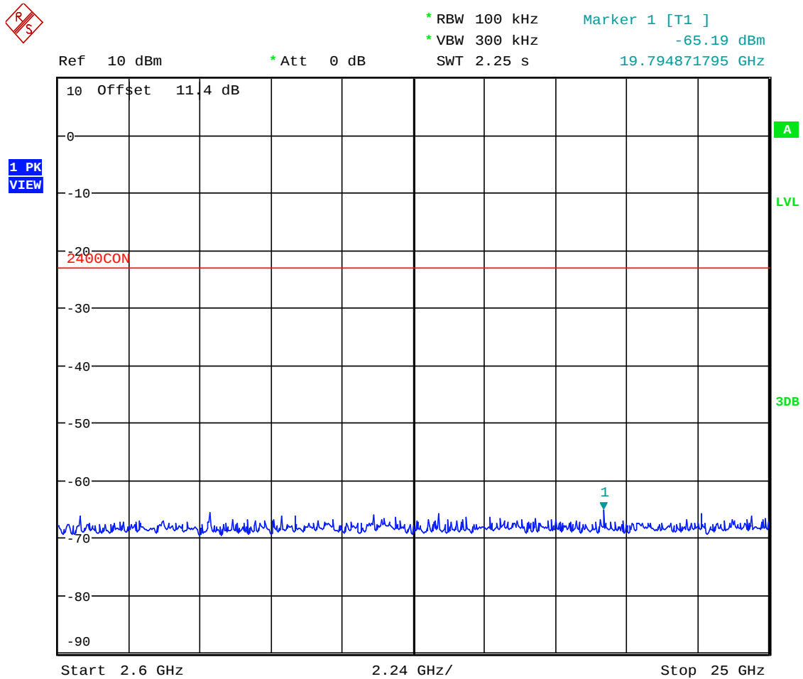
Plot 5.4.4.2.8. Conducted Spurious Emissions Channel 11, 2405 MHz, QPSK Modulation, Power Setting -26 Mode 3, 2.6 GHz – 25 GHz
