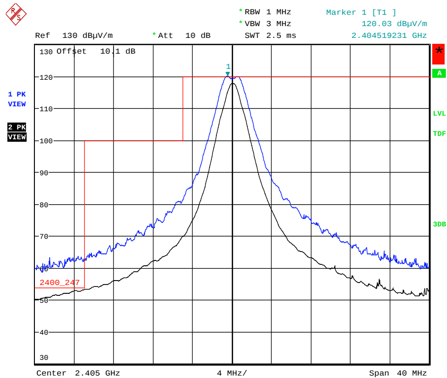
Plot 5.5.4.1.2.4. Band-Edge RF Radiated Emissions at 3 m, Vertical Polarization Low End of Frequency Band, QPSK Modulation, Power -7 Mode 3
