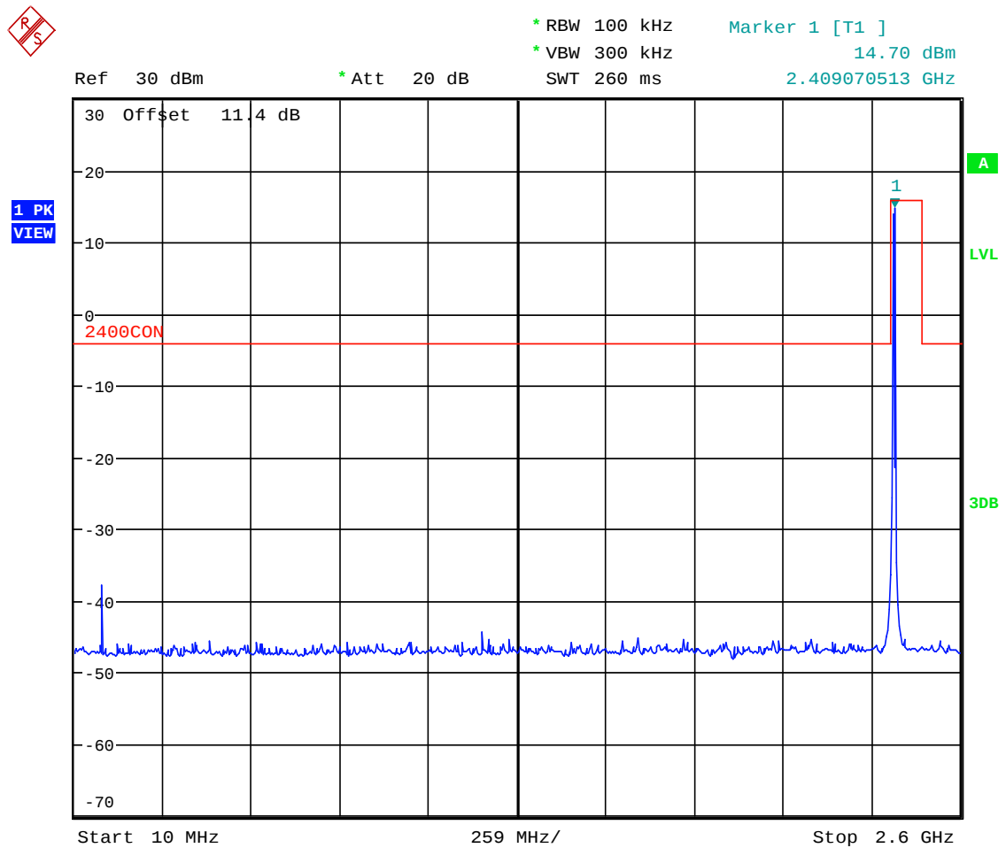
Plot 5.4.4.2.1. Conducted Spurious Emissions Channel 11, 2405 MHz, QPSK Modulation, Power Setting -7 Mode 3, 10 MHz – 2.6 GHz
