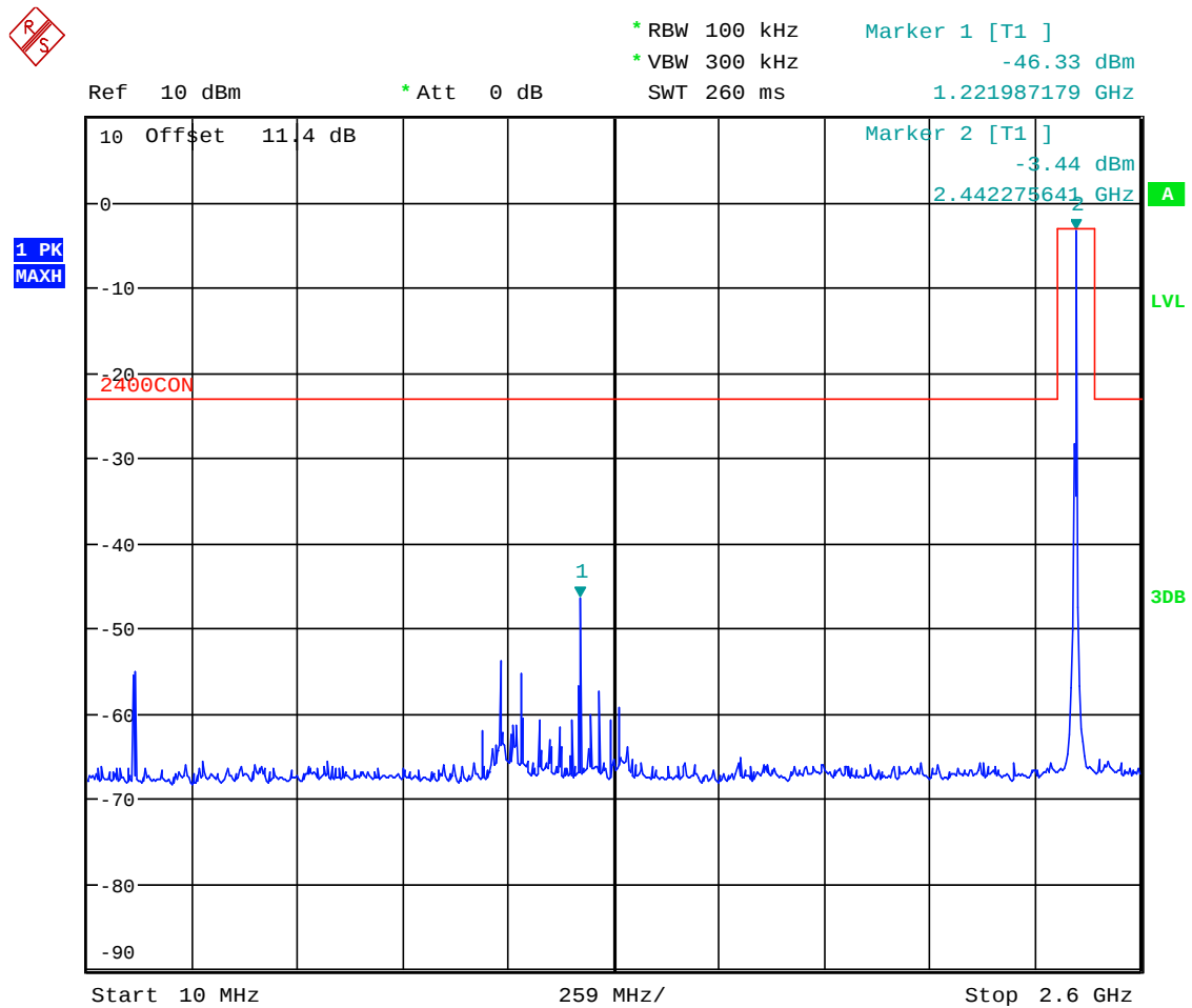
Plot 5.4.4.2.9. Conducted Spurious Emissions Channel 18, 2440 MHz, QPSK Modulation, Power Setting -26 Mode 3, 10 MHz – 2.6 GHz
