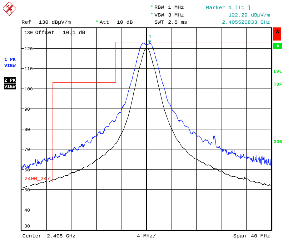
Plot 5.5.4.3.2.1. Band-Edge RF Radiated Emissions at 3 m, Horizontal Polarization Low End of Frequency Band, QPSK Modulation, Power -7 Mode 3
