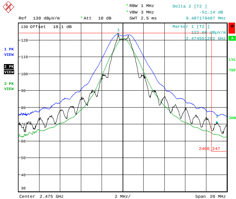
Plot 5.5.4.2.6. Band-Edge RF Radiated Emissions at 3 m, Vertical Polarization High End of Frequency Band, QPSK Modulation, Power -7 Mode 3
