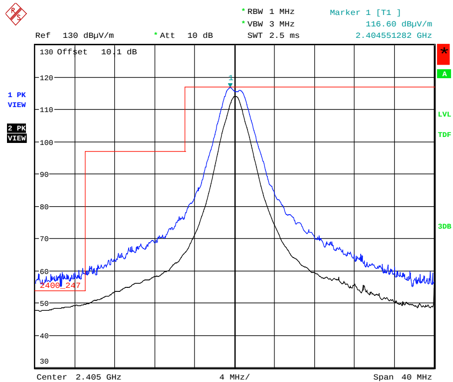
Plot 5.5.4.5.2.1. Band-Edge RF Radiated Emissions at 3 m, Horizontal Polarization Low End of Frequency Band, QPSK Modulation, Power -7 Mode 3
