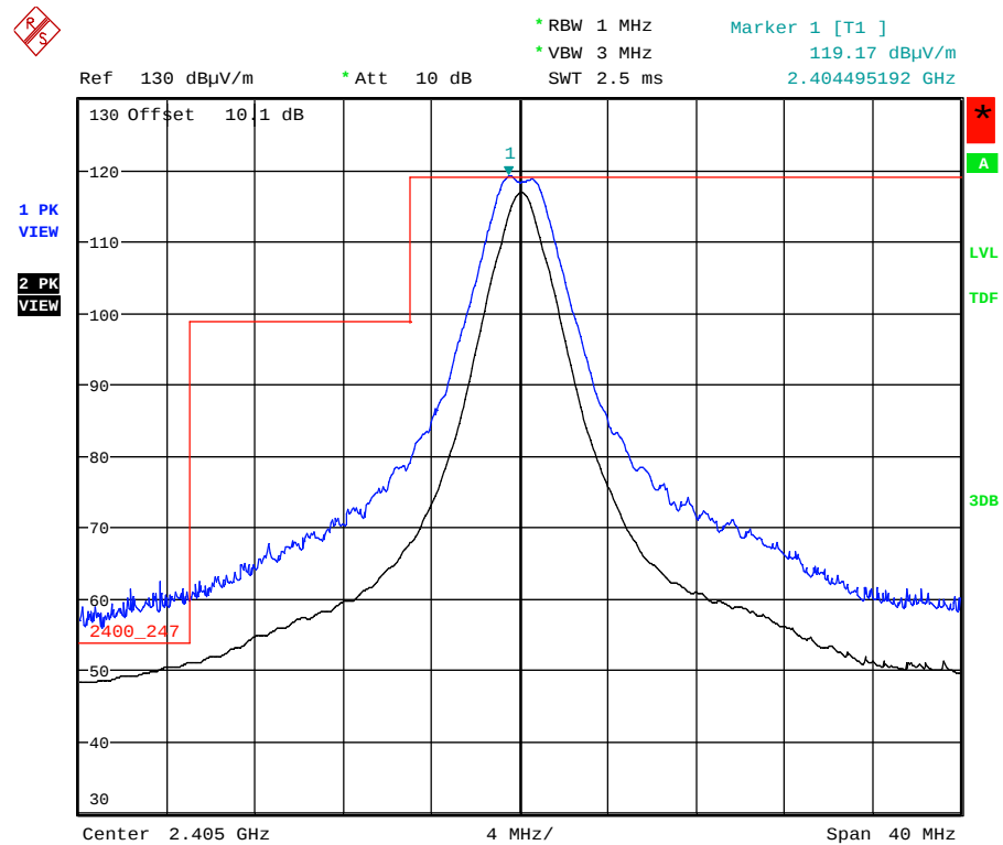
Plot 5.5.4.4.2.3. Band-Edge RF Radiated Emissions at 3 m, Vertical Polarization Low End of Frequency Band, QPSK Modulation, Power -7 Mode 3
