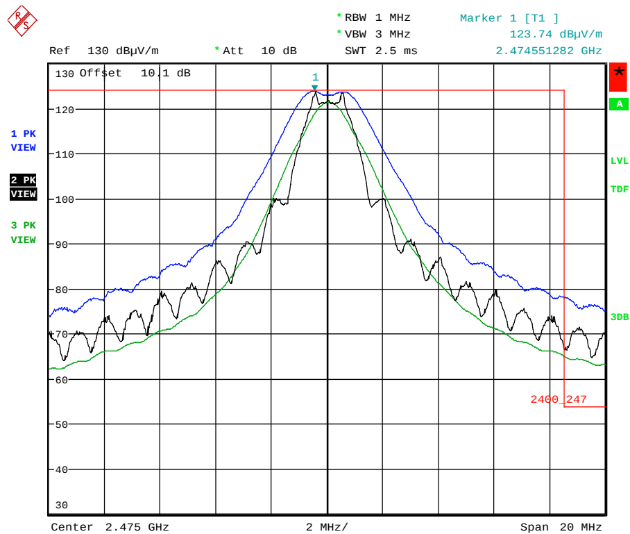
Plot 5.5.4.3.2.2. Band-Edge RF Radiated Emissions at 3 m, Horizontal Polarization High End of Frequency Band, QPSK Modulation, Power -7 Mode 3
