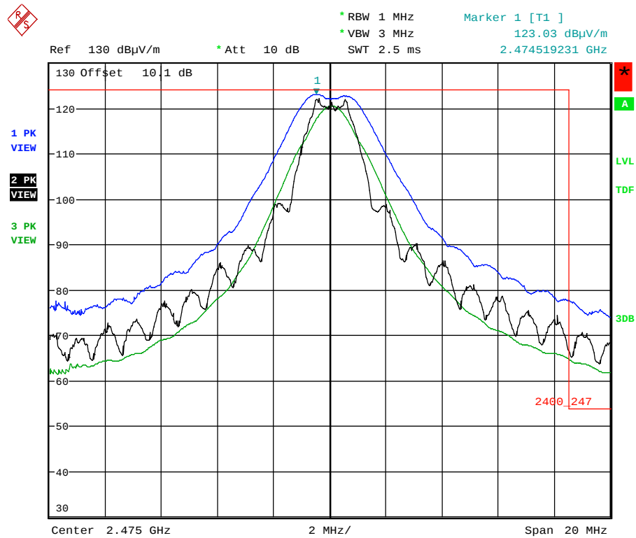
Plot 5.5.4.1.2.5. Band-Edge RF Radiated Emissions at 3 m, Vertical Polarization High End of Frequency Band, QPSK Modulation, Power -7 Mode 3
