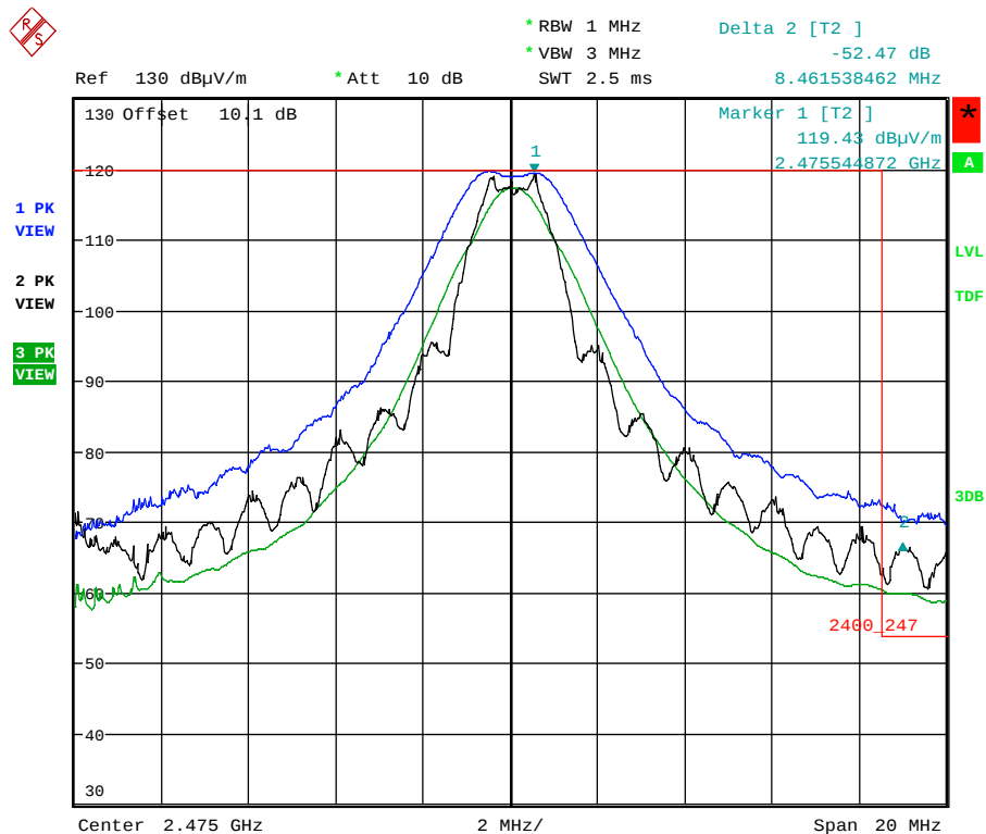
Plot 5.5.4.5.2.3. Band-Edge RF Radiated Emissions at 3 m, Horizontal Polarization High End of Frequency Band, QPSK Modulation, Power -7 Mode 3
