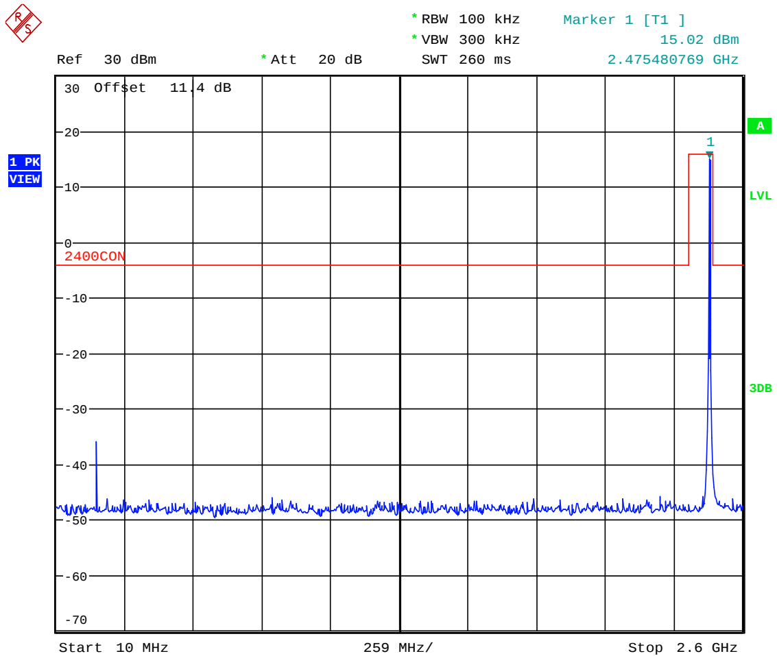
Plot 5.4.4.2.5. Conducted Spurious Emissions Channel 25, 2475 MHz, QPSK Modulation, Power Setting -7 Mode 3, 10 MHz – 2.6 GHz
