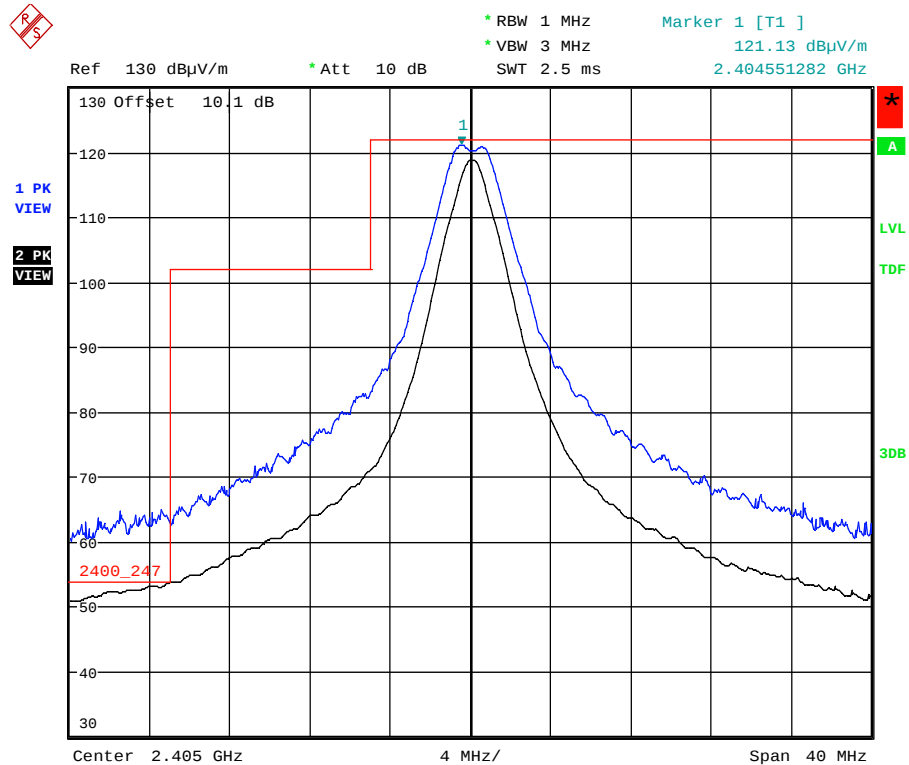
Plot 5.5.4.2.2.1. Band-Edge RF Radiated Emissions at 3 m, Horizontal Polarization Low End of Frequency Band, QPSK Modulation, Power -7 Mode 3
