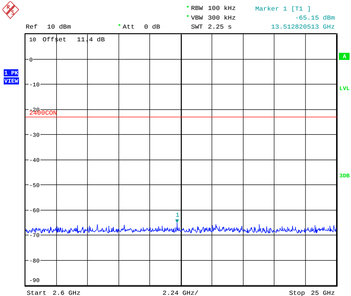
Plot 5.4.4.2.10. Conducted Spurious Emissions Channel 18, 2440 MHz, QPSK Modulation, Power Setting -26 Mode 3, 2.6 GHz – 25 GHz
