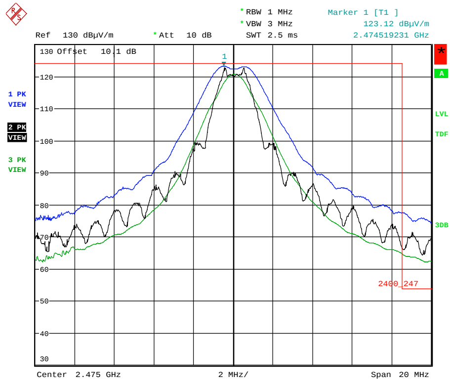
Plot 5.5.4.2.2.5. Band-Edge RF Radiated Emissions at 3 m, Vertical Polarization High End of Frequency Band, QPSK Modulation, Power -7 Mode 3
