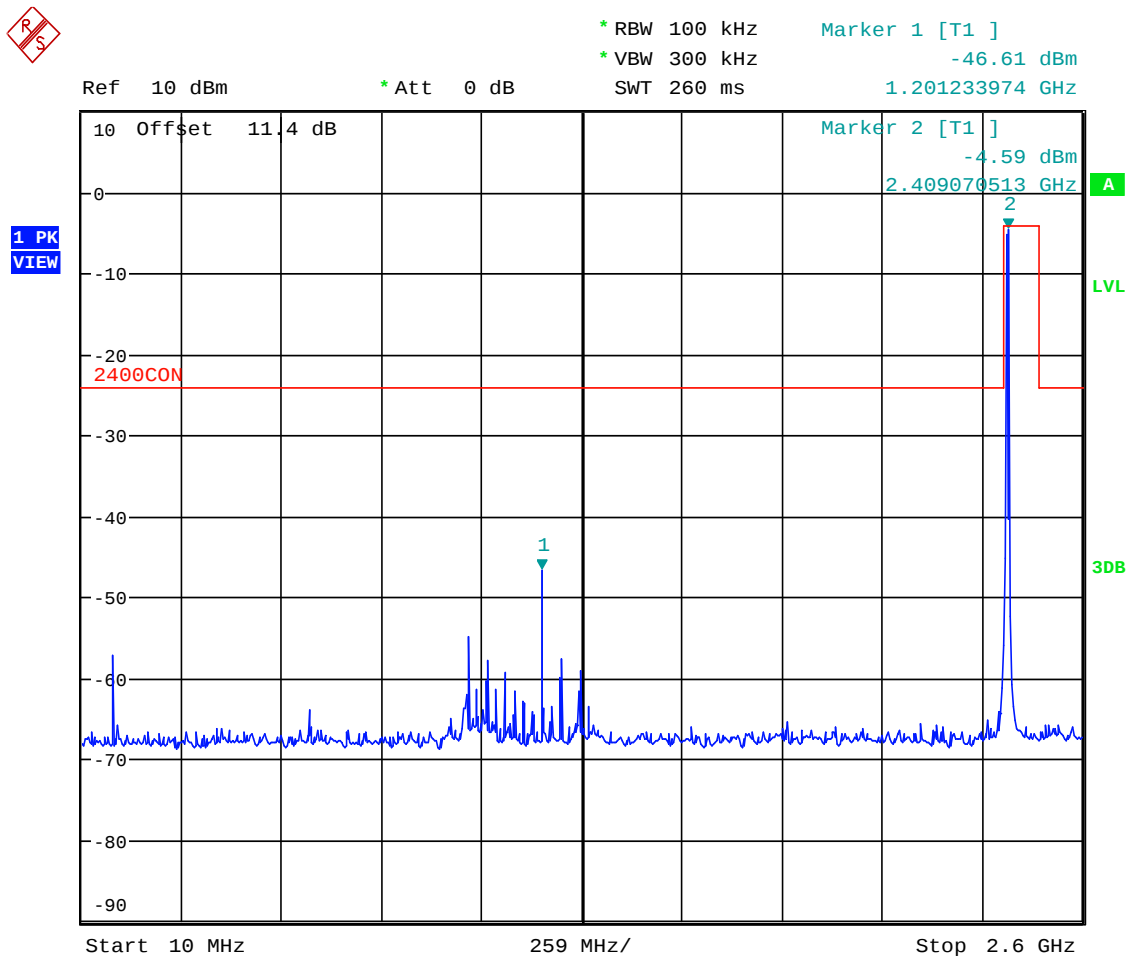
Plot 5.4.4.2.7. Conducted Spurious Emissions Channel 11, 2405 MHz, QPSK Modulation, Power Setting -26 Mode 3, 10 MHz – 2.6 GHz
