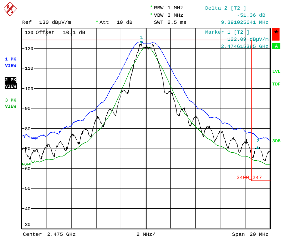
Plot 5.5.4.1.2.6. Band-Edge RF Radiated Emissions at 3 m, Vertical Polarization High End of Frequency Band, QPSK Modulation, Power -7 Mode 3
