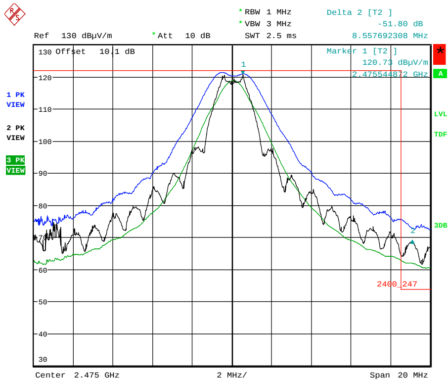
Plot 5.5.4.1.2.3. Band-Edge RF Radiated Emissions at 3 m, Horizontal Polarization High End of Frequency Band, QPSK Modulation, Power -7 Mode 3
