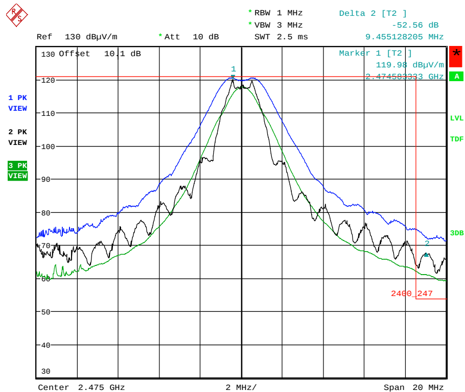
Plot 5.5.4.5.2.6. Band-Edge RF Radiated Emissions at 3 m, Vertical Polarization High End of Frequency Band, QPSK Modulation, Power -7 Mode 3
