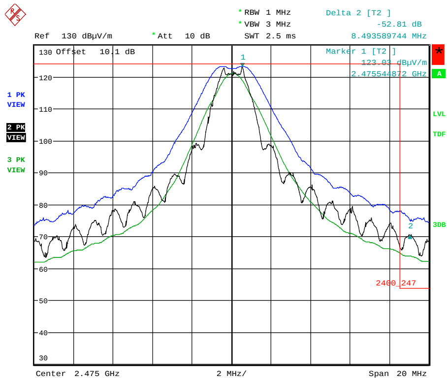
Plot 5.5.4.2.2.3. Band-Edge RF Radiated Emissions at 3 m, Horizontal Polarization High End of Frequency Band, QPSK Modulation, Power -7 Mode 3
