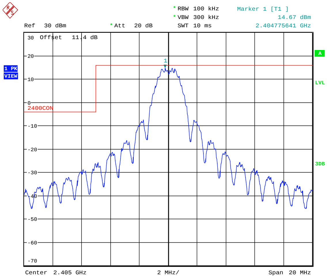
Plot 5.4.4.1.1. Band-Edge RF Conducted Emissions Lower Band-edge, Channel 11, 2405 MHz, QPSK Modulation, Power Setting -7 Mode 3
