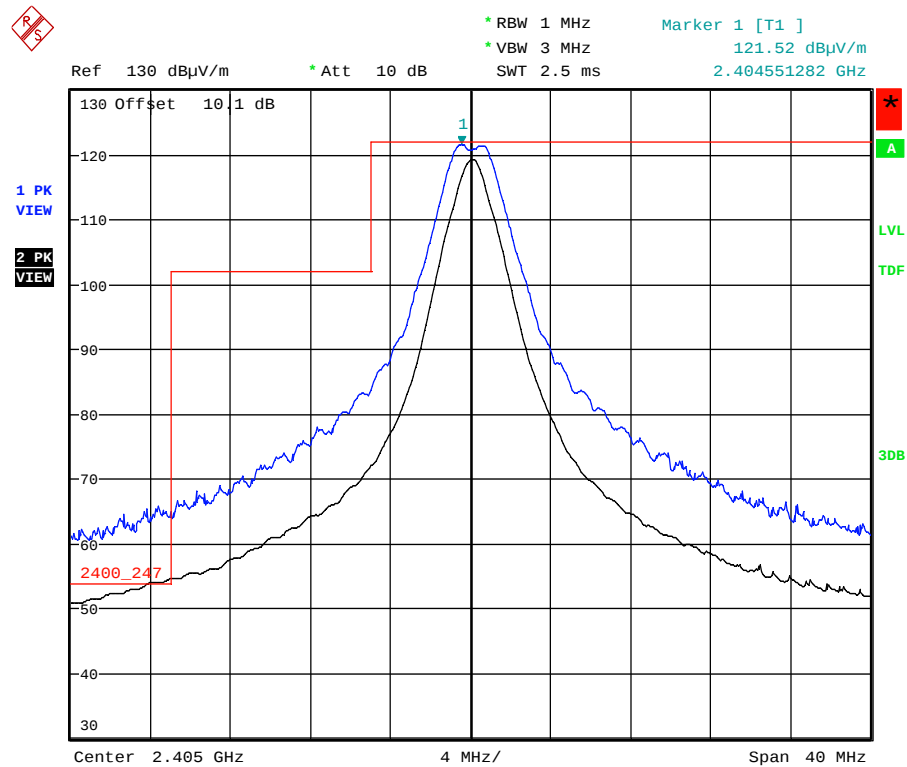
Plot 5.5.4.2.2.4. Band-Edge RF Radiated Emissions at 3 m, Vertical Polarization Low End of Frequency Band, QPSK Modulation, Power -7 Mode 3
