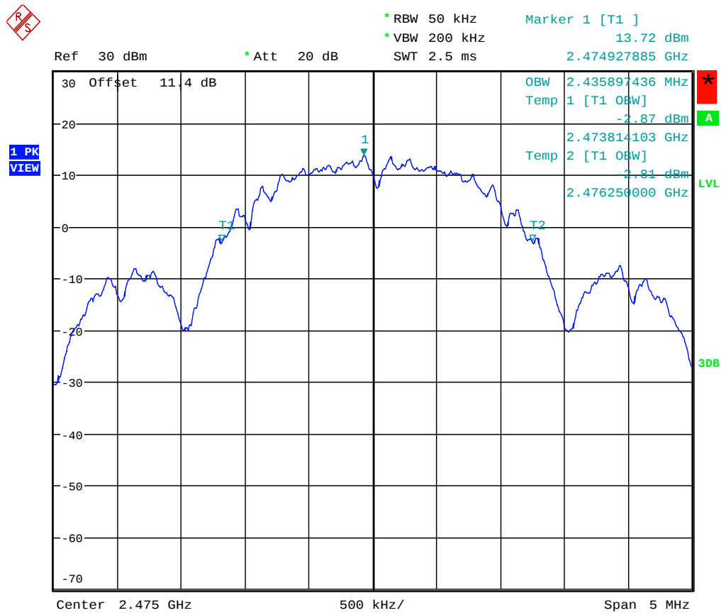
Plot 5.2.4.6. 99% Occupied Bandwidth, Channel 25, 2475 MHz, QPSK Modulation, Power Setting -7 Mode 3
