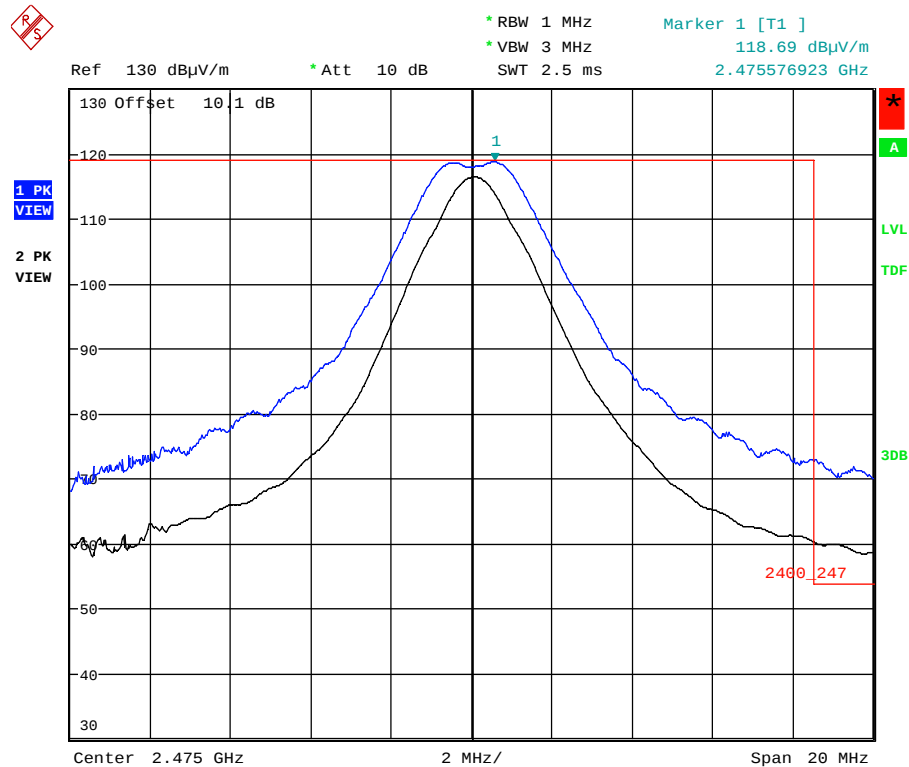
Plot 5.5.4.4.2.4. Band-Edge RF Radiated Emissions at 3 m, Vertical Polarization High End of Frequency Band, QPSK Modulation, Power -7 Mode 3
