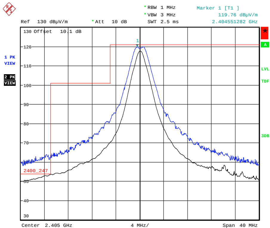
Plot 5.5.4.5.2.4. Band-Edge RF Radiated Emissions at 3 m, Vertical Polarization Low End of Frequency Band, QPSK Modulation, Power -7 Mode 3
