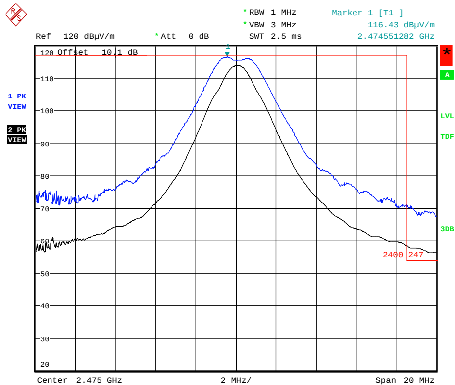
Plot 5.5.4.4.2.2. Band-Edge RF Radiated Emissions at 3 m, Horizontal Polarization High End of Frequency Band, QPSK Modulation, Power -7 Mode 3
