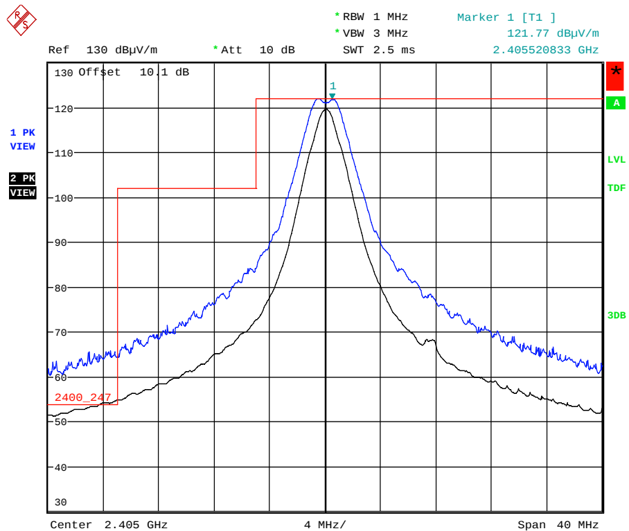
Plot 5.5.4.3.2.4. Band-Edge RF Radiated Emissions at 3 m, Vertical Polarization Low End of Frequency Band, QPSK Modulation, Power -7 Mode 3
