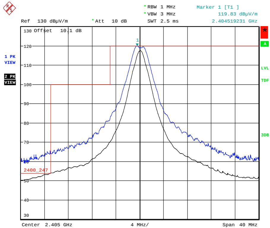
Plot 5.5.4.1.2.1. Band-Edge RF Radiated Emissions at 3 m, Horizontal Polarization Low End of Frequency Band, QPSK Modulation, Power -7 Mode 3
