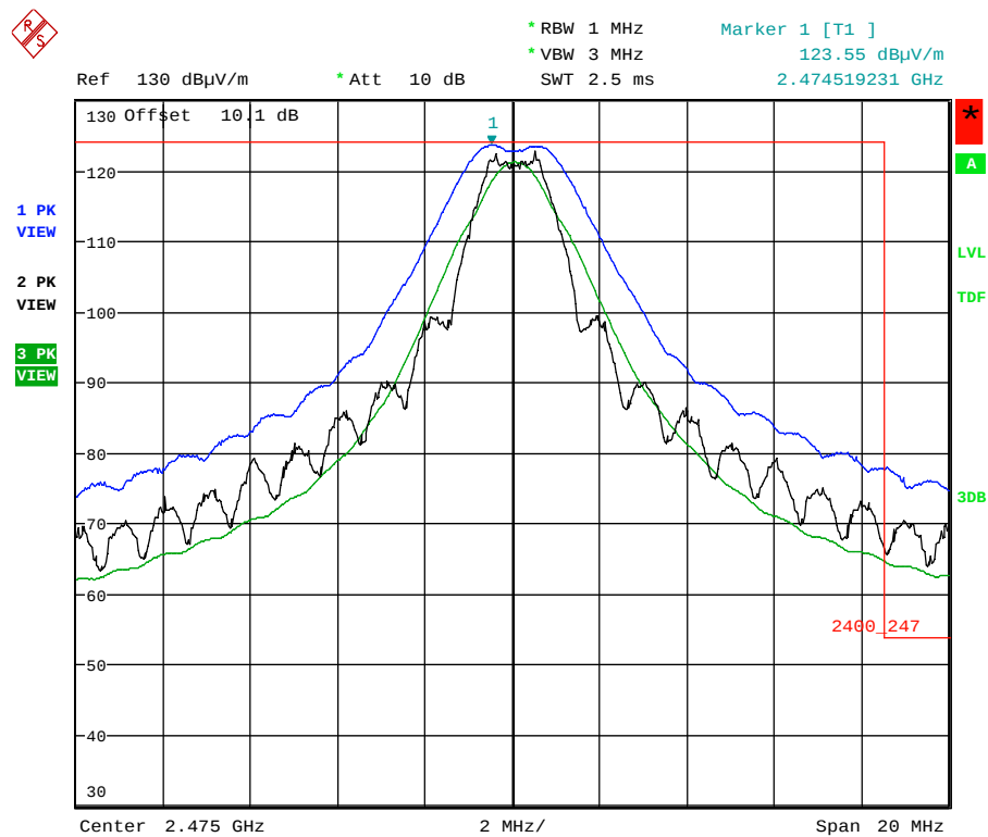
Plot 5.5.4.3.2.5. Band-Edge RF Radiated Emissions at 3 m, Vertical Polarization High End of Frequency Band, QPSK Modulation, Power -7 Mode 3
