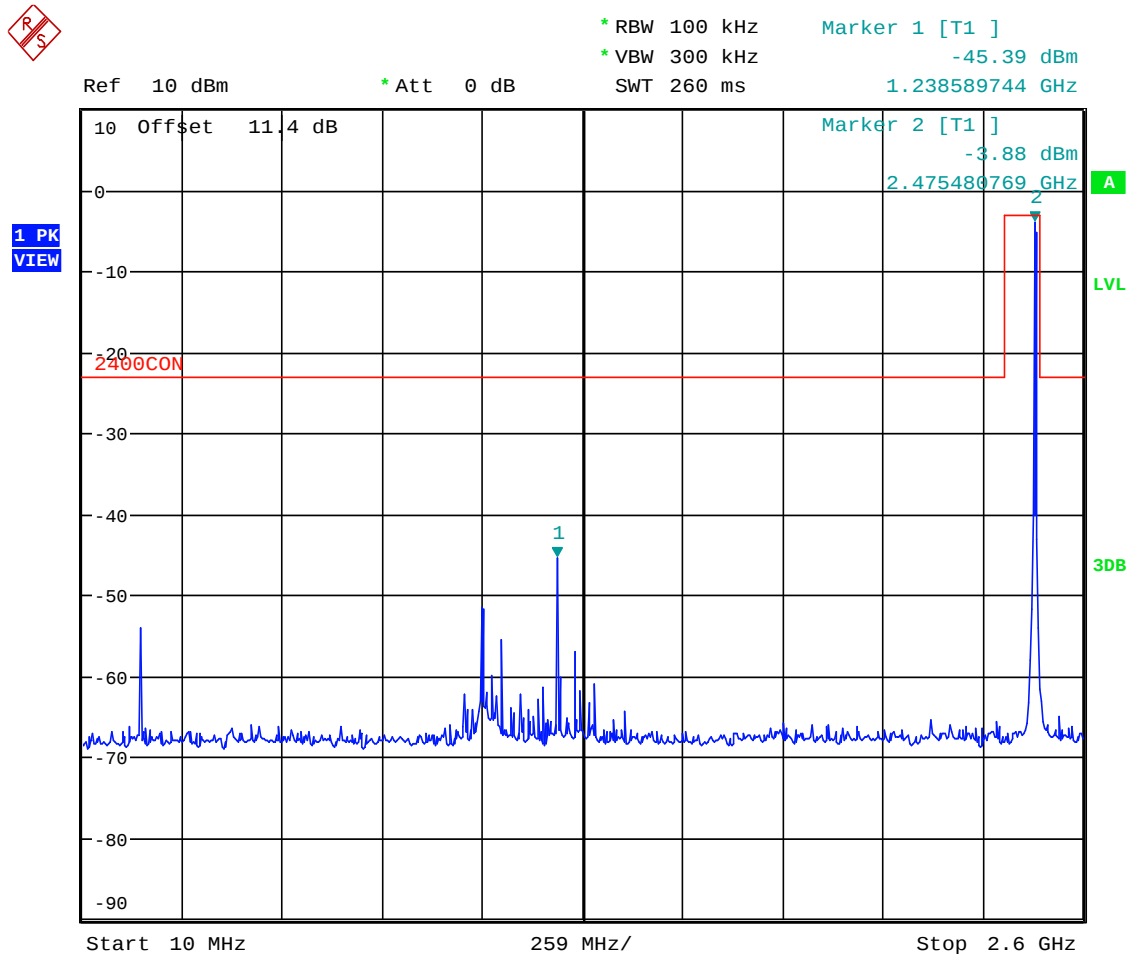
Plot 5.4.4.2.11. Conducted Spurious Emissions Channel 25, 2475 MHz, QPSK Modulation, Power Setting -26 Mode 3, 10 MHz – 2.6 GHz
