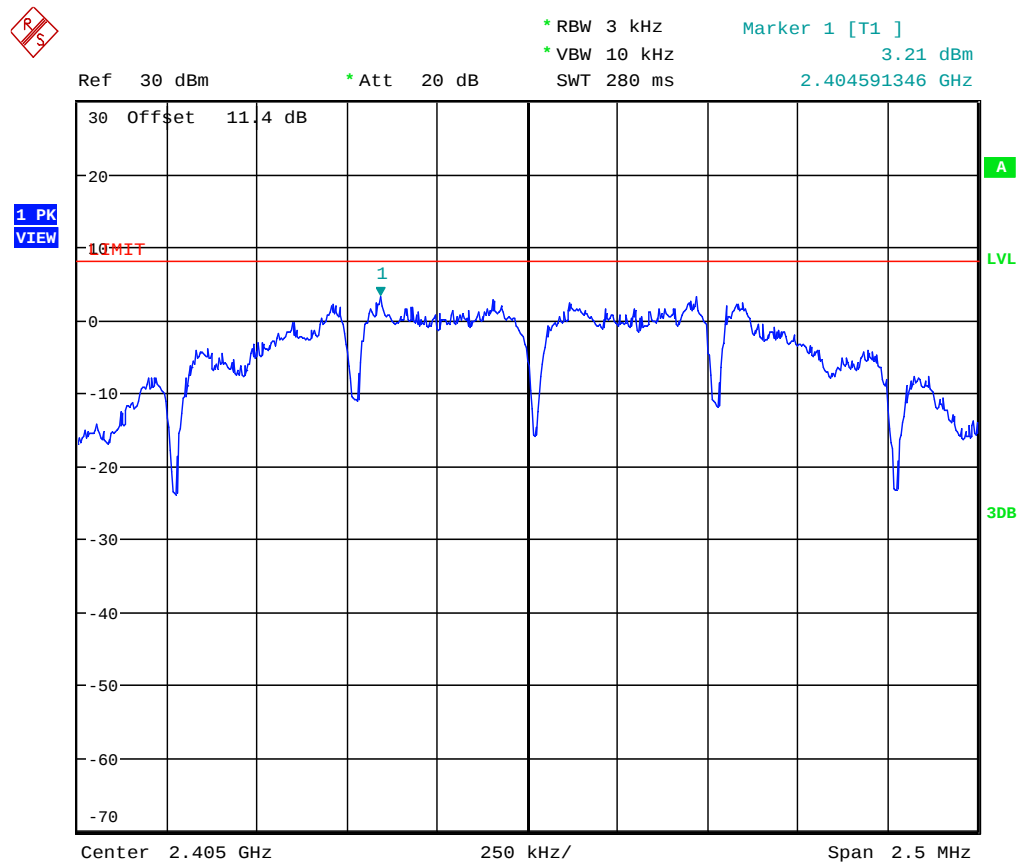
Plot 5.6.4.1. Power Spectral Density, Channel 11, 2405 MHz, QPSK Modulation, Power Setting -7 Mode 3
