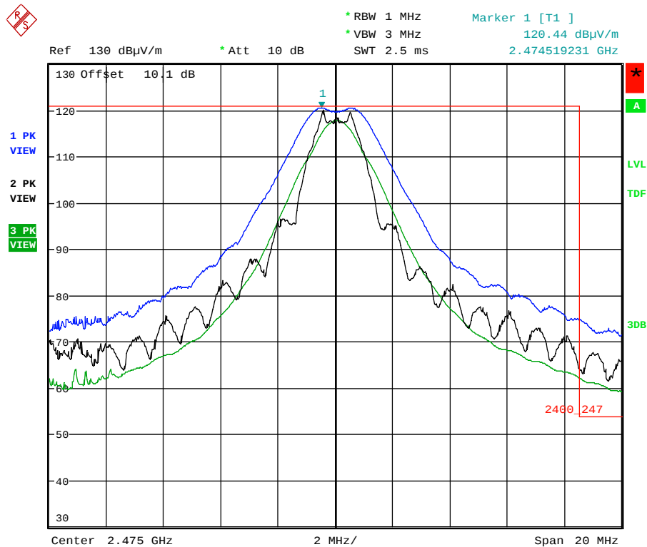
Plot 5.5.4.5.2.5. Band-Edge RF Radiated Emissions at 3 m, Vertical Polarization High End of Frequency Band, QPSK Modulation, Power -7 Mode 3
