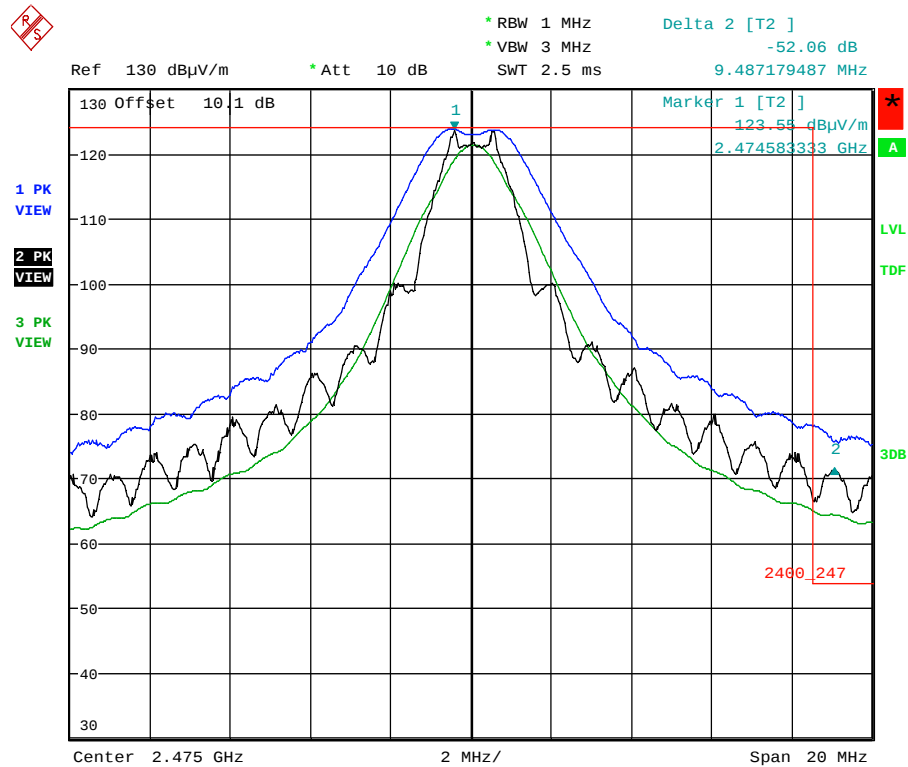
Plot 5.5.4.3.2.3. Band-Edge RF Radiated Emissions at 3 m, Horizontal Polarization High End of Frequency Band, QPSK Modulation, Power -7 Mode 3
