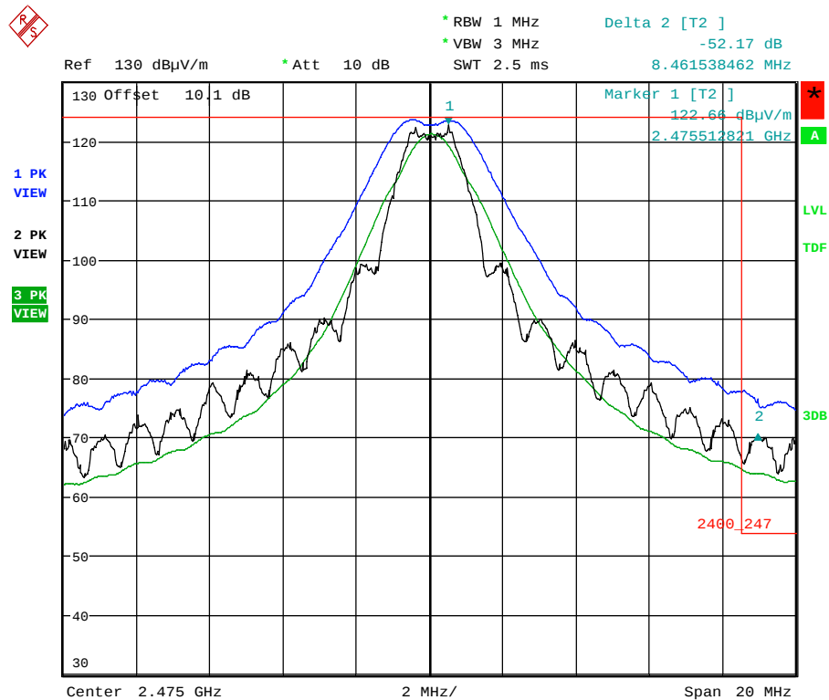
Plot 5.5.4.3.2.6. Band-Edge RF Radiated Emissions at 3 m, Vertical Polarization High End of Frequency Band, QPSK Modulation, Power -7 Mode 3
