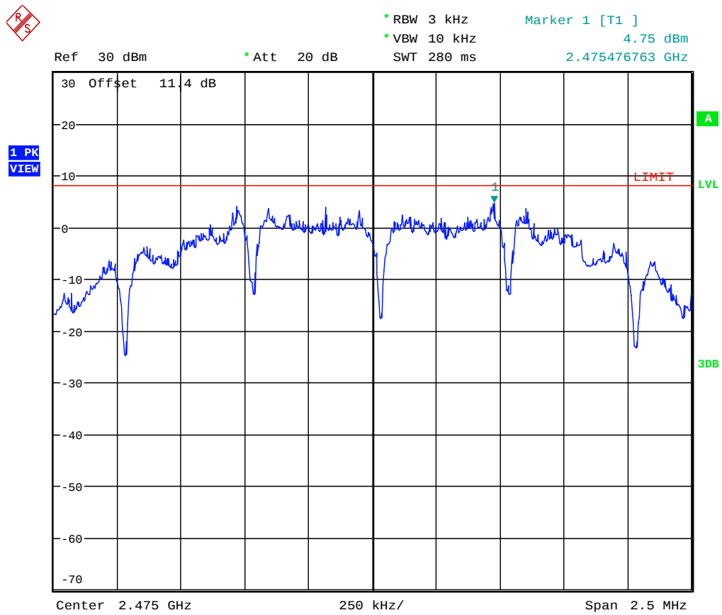
Plot 5.6.4.3. Power Spectral Density, Channel 25, 2475 MHz, QPSK Modulation, Power Setting -7 Mode 3
