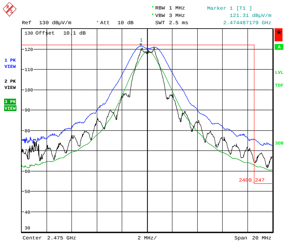
Plot 5.5.4.1.2.2. Band-Edge RF Radiated Emissions at 3 m, Horizontal Polarization High End of Frequency Band, QPSK Modulation, Power -7 Mode 3
