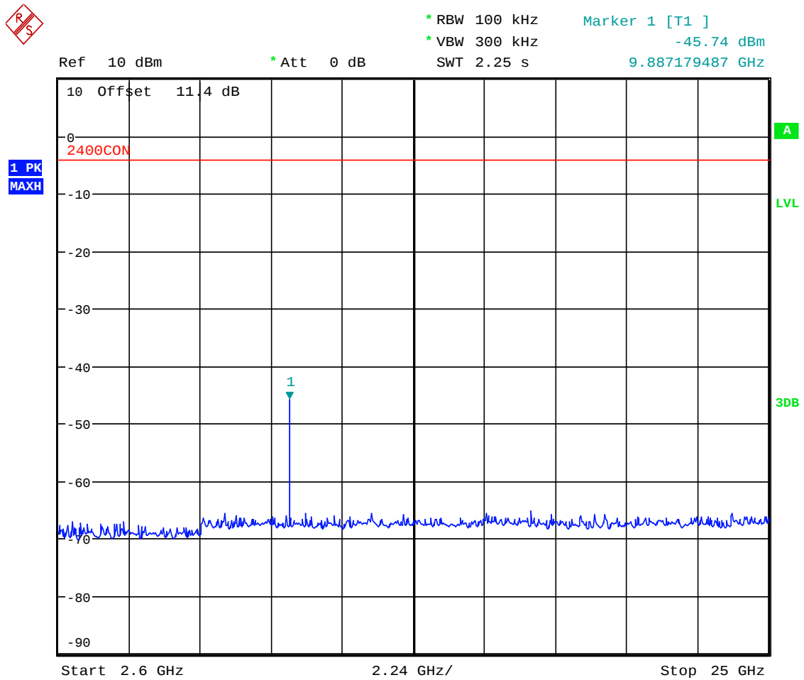
Plot 5.4.4.2.6. Conducted Spurious Emissions Channel 25, 2475 MHz, QPSK Modulation, Power Setting -7 Mode 3, 2.6 GHz – 25 GHz
