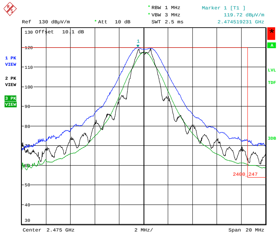
Plot 5.5.4.5.2.2. Band-Edge RF Radiated Emissions at 3 m, Horizontal Polarization High End of Frequency Band, QPSK Modulation, Power -7 Mode 3
