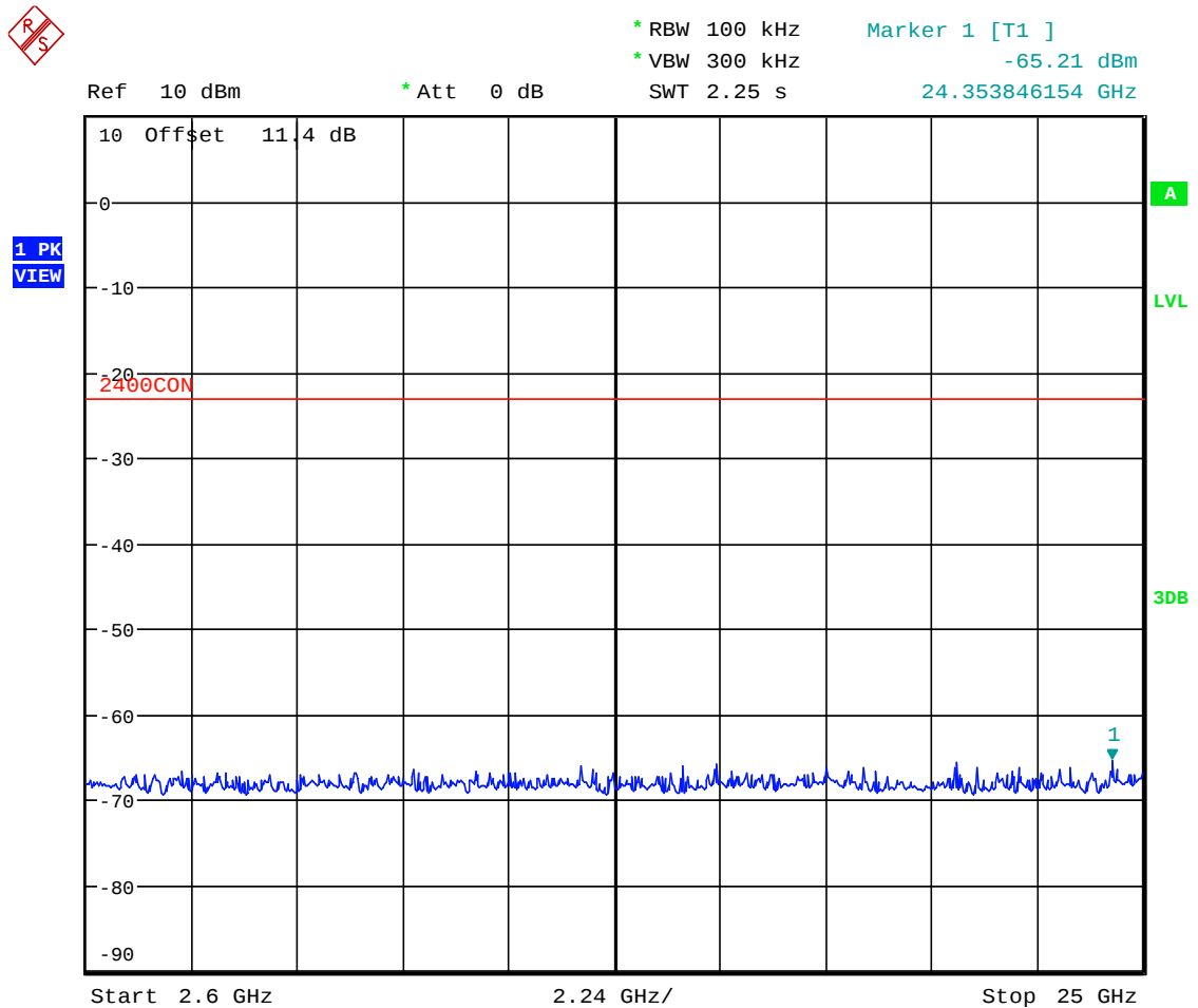
Plot 5.4.4.2.12. Conducted Spurious Emissions Channel 25, 2475 MHz, QPSK Modulation, Power Setting -26 Mode 3, 2.6 GHz – 25 GHz
