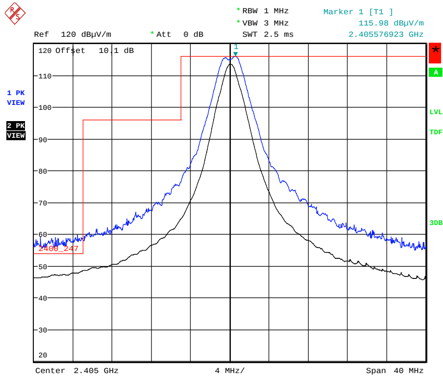
Plot 5.5.4.4.2.1. Band-Edge RF Radiated Emissions at 3 m, Horizontal Polarization Low End of Frequency Band, QPSK Modulation, Power -7 Mode 3
