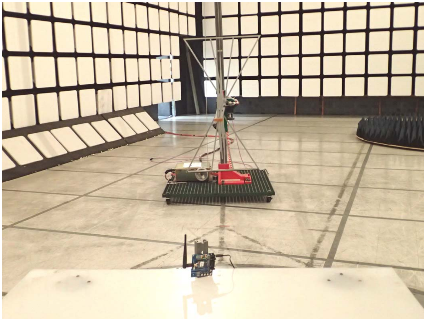
Radiated Emissions @ 3 m, Orthogonal Position 2 EUT with 2.1 dBi Dipole Antenna
