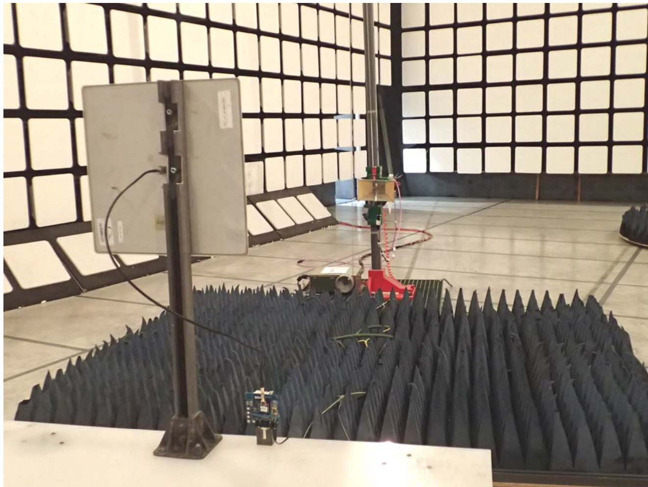
Radiated Emissions @ 3 m, Orthogonal Position 3 EUT with 19.0 dBi Flat Panel Antenna
