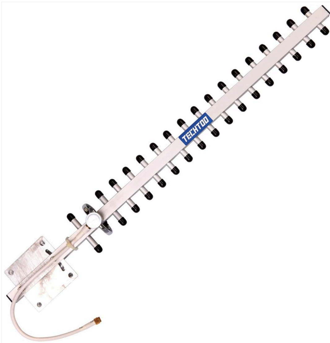
Figure 1: TECHTOO 2.4GHz 18dBi Yagi Directional WiFi Antenna.
