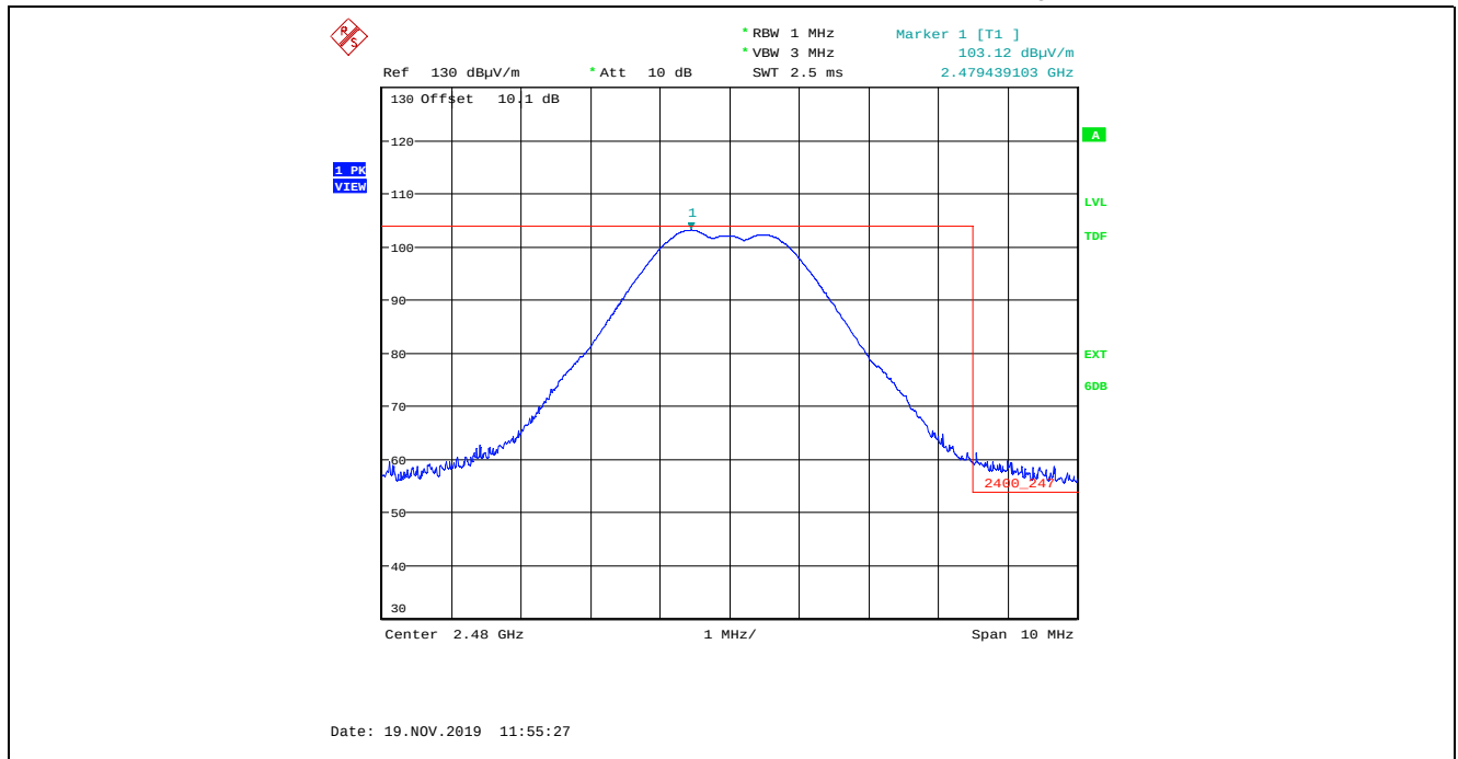
Plot 5.2.4.2.9. Band-Edge Radiated Emissions, Higher Band-edge, Peak Detector Rx Antenna in Vertical Polarization, QPSK Modulation, Power Setting 13, 2480 MHz
