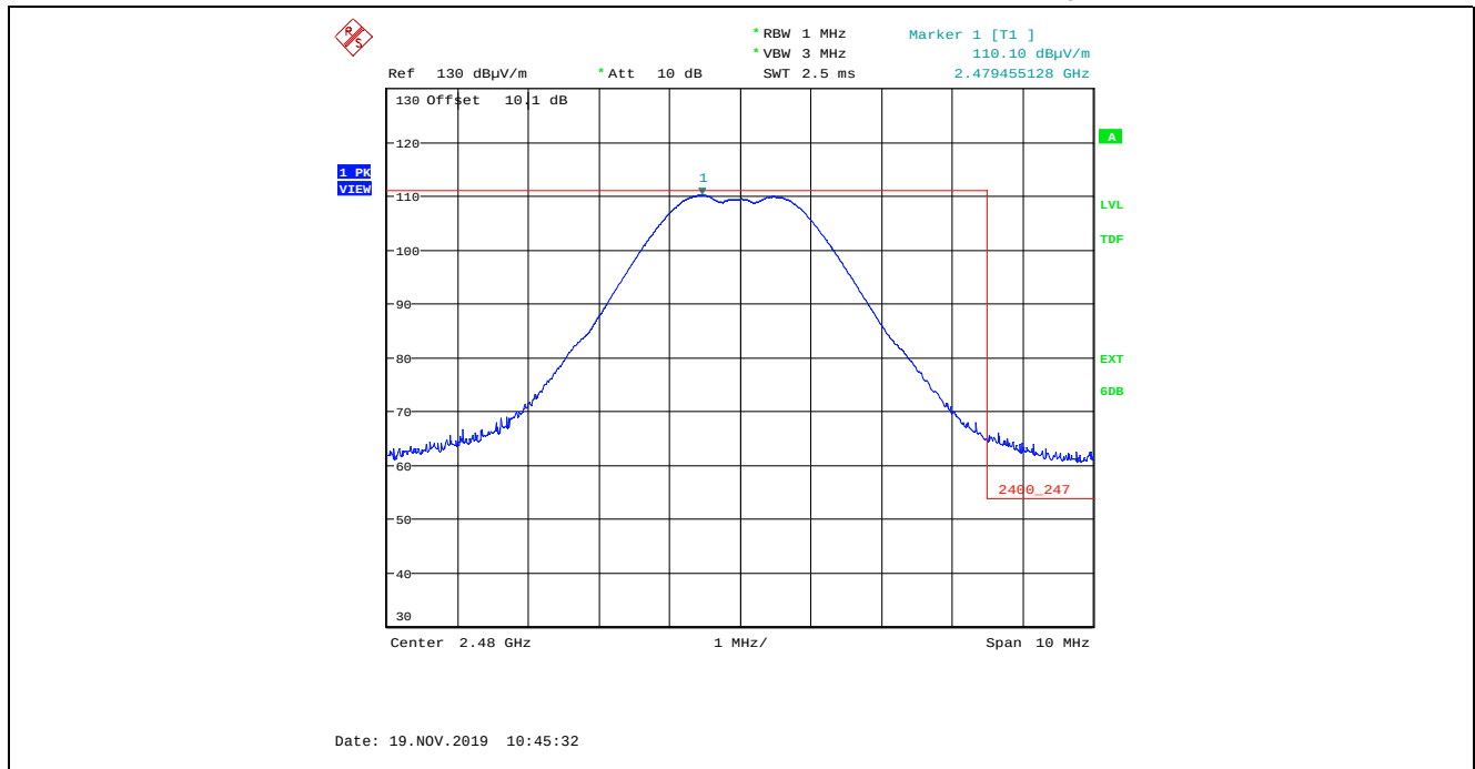
Plot 5.2.4.2.11. Band-Edge Radiated Emissions, Higher Band-edge, Peak Detector Rx Antenna in Horizontal Polarization, QPSK Modulation, Power Setting 13, 2480 MHz
