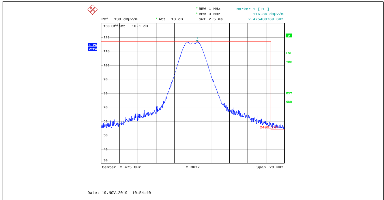
Plot 5.2.4.2.7. Band-Edge Radiated Emissions, Higher Band-edge, Peak Detector Rx Antenna in Horizontal Polarization, QPSK Modulation, Power Setting 20, 2475 MHz
