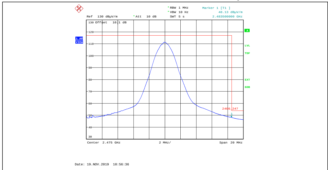
Plot 5.2.4.2.8. Band-Edge Radiated Emissions, Higher Band-edge, Average Detector Rx Antenna in Horizontal Polarization, QPSK Modulation, Power Setting 20, 2475 MHz
