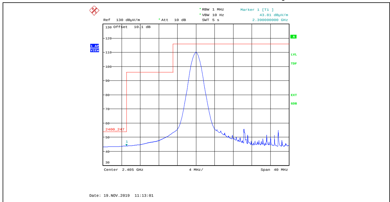
Plot 5.2.4.2.4. Band-Edge Radiated Emissions, Lower Band-edge, Average Detector Rx Antenna in Horizontal Polarization, QPSK Modulation, Power Setting 20, 2405 MHz
