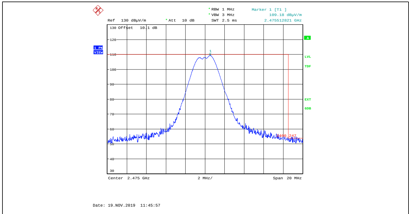
Plot 5.2.4.2.5. Band-Edge Radiated Emissions, Higher Band-edge, Peak Detector Rx Antenna in Vertical Polarization, QPSK Modulation, Power Setting 20, 2475 MHz
