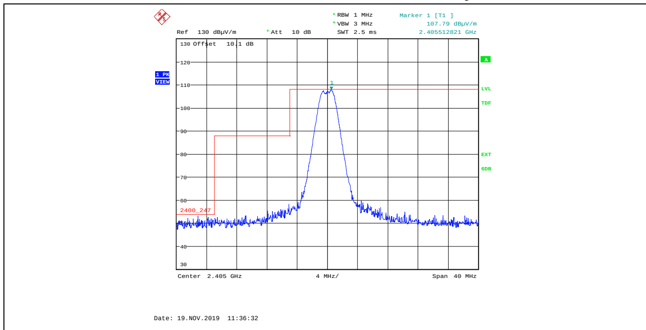
Plot 5.2.4.2.1. Band-Edge Radiated Emissions, Lower Band-edge, Peak Detector Rx Antenna in Vertical Polarization, QPSK Modulation, Power Setting 20, 2405 MHz
