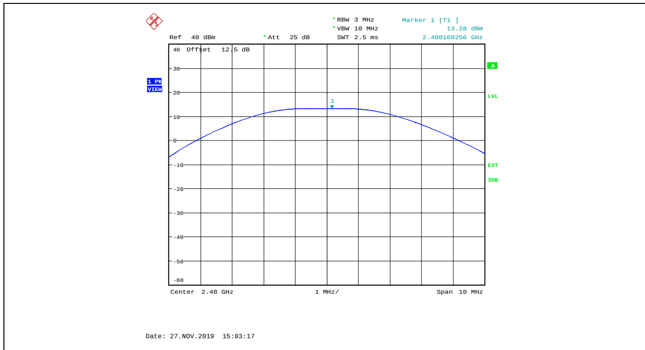
Plot 5.1.4.4. Maximum Peak Conducted Output Power, QPSK Modulation, Power Setting 13, Ch 26, 2480 MHz
