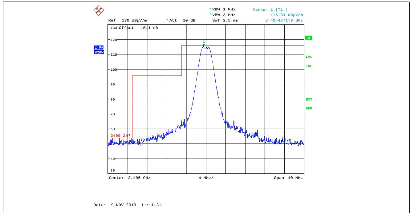
Plot 5.2.4.2.3. Band-Edge Radiated Emissions, Lower Band-edge, Peak Detector Rx Antenna in Horizontal Polarization, QPSK Modulation, Power Setting 20, 2405 MHz
