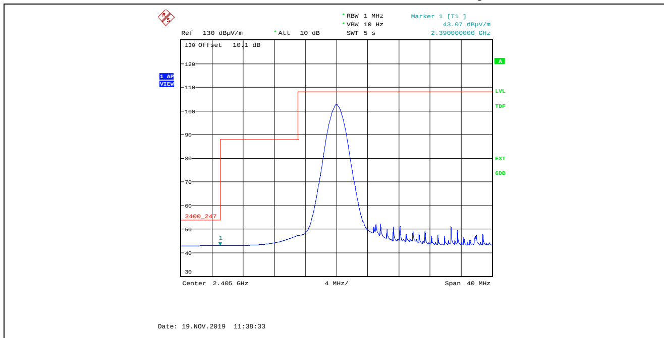
Plot 5.2.4.2.2. Band-Edge Radiated Emissions, Lower Band-edge, Average Detector Rx Antenna in Vertical Polarization, QPSK Modulation, Power Setting 20, 2405 MHz
