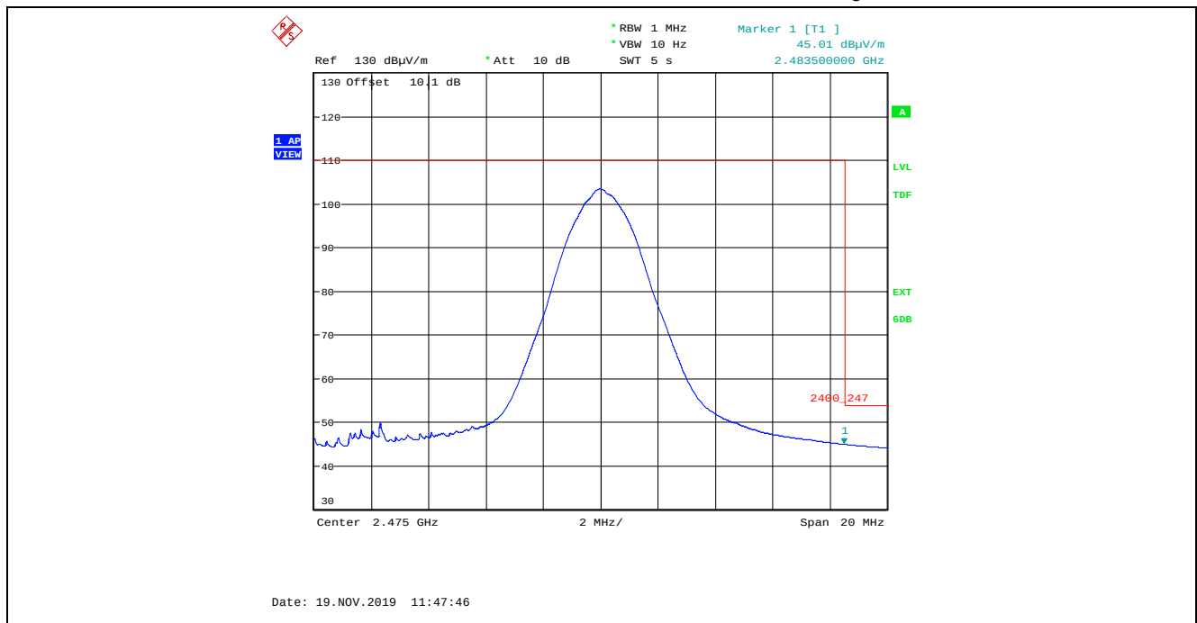
Plot 5.2.4.2.6. Band-Edge Radiated Emissions, Higher Band-edge, Average Detector Rx Antenna in Vertical Polarization, QPSK Modulation, Power Setting 20, 2475 MHz
