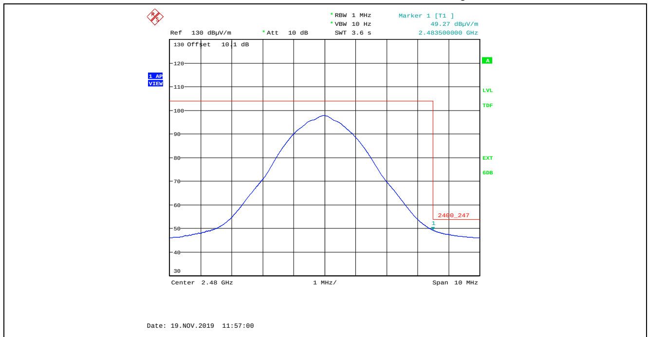
Plot 5.2.4.2.10. Band-Edge Radiated Emissions, Higher Band-edge, Average Detector Rx Antenna in Vertical Polarization, QPSK Modulation, Power Setting 13, 2480 MHz
