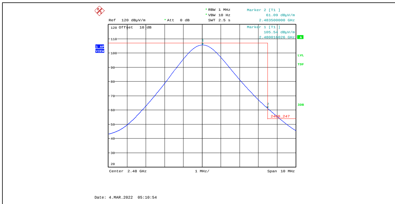
Plot 5.4.4.1.2.8. Band-Edge RF Radiated Emissions at 3 m, Vertical Polarization, Average High End of Frequency Band, 2480 MHz, 8 dBm Power Setting, 1 Mbps Marker 2: 61.09 dBμV/m – 33.36 dB Duty Cycle Factor = 27.73 dBμV/m (Limit 54 dBμV/m)
