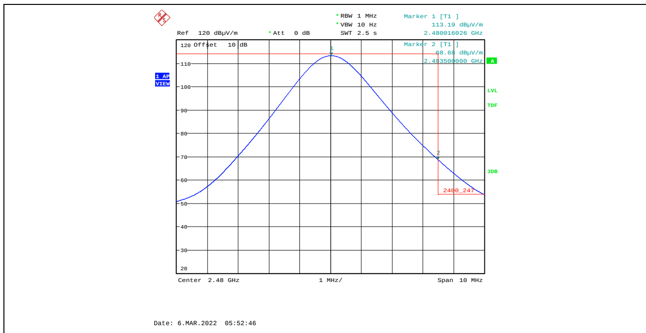
Plot 5.4.4.2.2.6. Band-Edge RF Radiated Emissions at 3 m, Horizontal Polarization, Average High End of Frequency Band, 2480 MHz, 8 dBm Power Setting, 1 Mbps Marker 2: 68.68 dBμV/m – 33.36 dB Duty Cycle Factor = 35.32 dBμV/m (Limit 54 dBμV/m)
