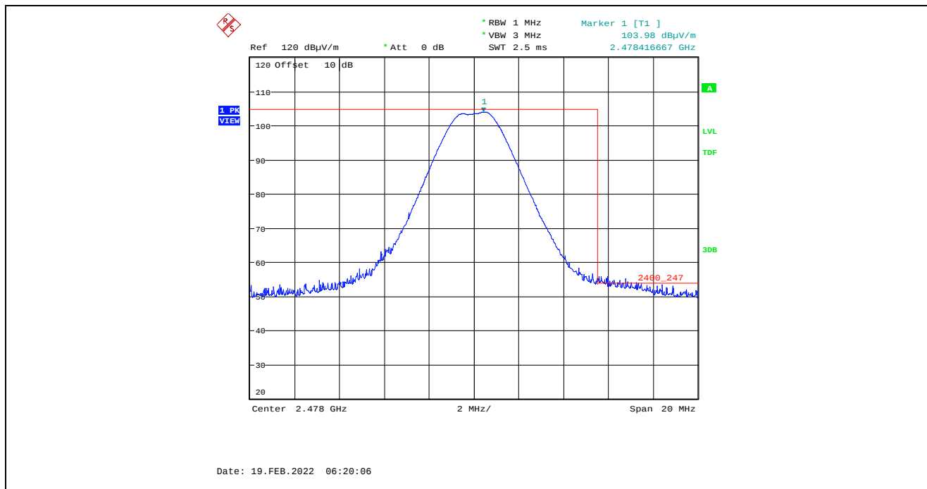
Plot 5.4.4.5.2.5. Band-Edge RF Radiated Emissions at 3 m, Horizontal Polarization, Peak High End of Frequency Band, 2478 MHz, 8 dBm Power Setting, 2 Mbps
