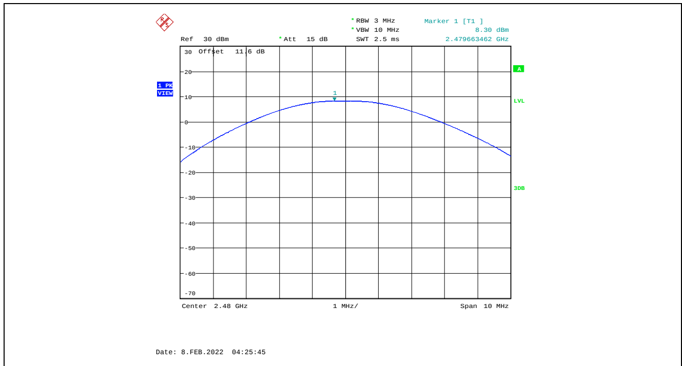
Plot 5.3.4.3. Maximum Peak Conducted Output Power, GFSK Modulation, 1 Mbps, 8 dBm Power Setting, 2480 MHz
