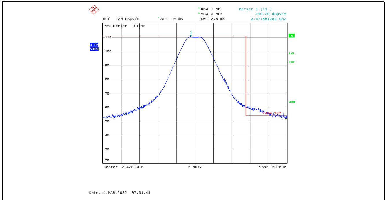
Plot 5.4.4.7.2.7. Band-Edge RF Radiated Emissions at 3 m, Vertical Polarization, Peak High End of Frequency Band, 2478 MHz, 8 dBm Power Setting, 2 Mbps
