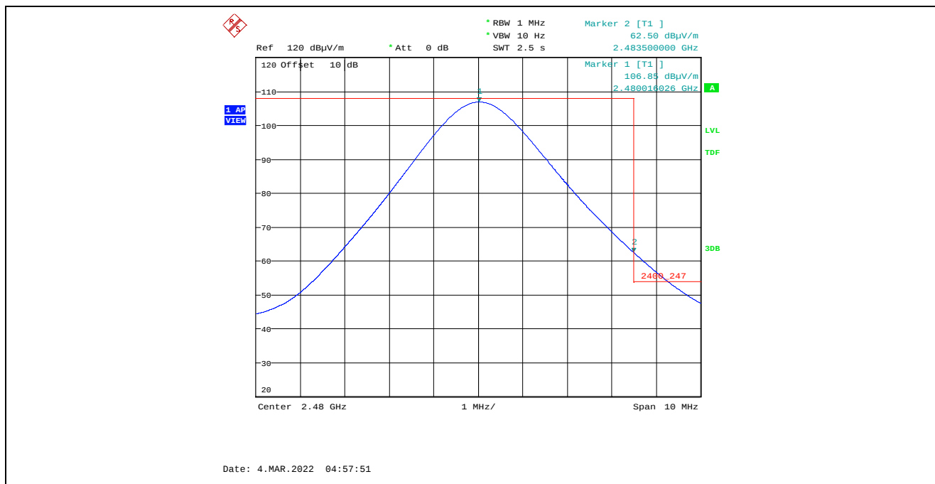
Plot 5.4.4.1.2.6. Band-Edge RF Radiated Emissions at 3 m, Horizontal Polarization, Average High End of Frequency Band, 2480 MHz, 8 dBm Power Setting, 1 Mbps Marker 2: 62.50 dBμV/m – 33.36 dB Duty Cycle Factor = 29.14 dBμV/m (Limit 54 dBμV/m)
