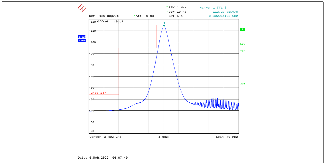
Plot 5.4.4.2.2.2. Band-Edge RF Radiated Emissions at 3 m, Horizontal Polarization, Average Low End of Frequency Band, 2402 MHz, 8 dBm Power Setting, 1 Mbps
