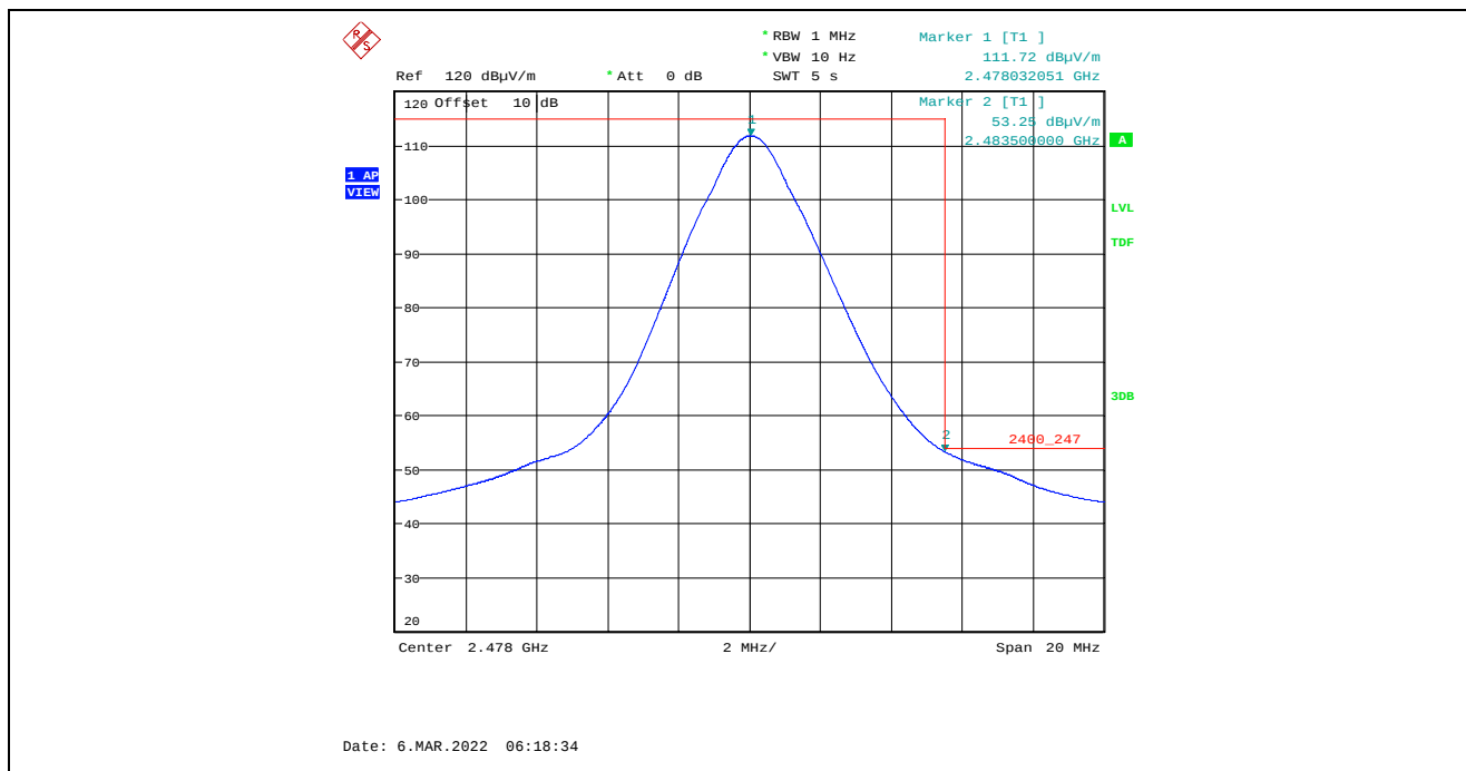
Plot 5.4.4.6.2.6. Band-Edge RF Radiated Emissions at 3 m, Horizontal Polarization, Average High End of Frequency Band, 2478 MHz, 8 dBm Power Setting, 2 Mbps
