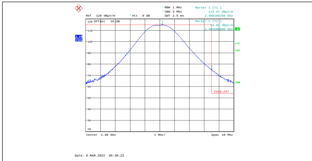
Plot 5.4.4.2.7. Band-Edge RF Radiated Emissions at 3 m, Vertical Polarization, Peak High End of Frequency Band, 2480 MHz, 8 dBm Power Setting, 1 Mbps
