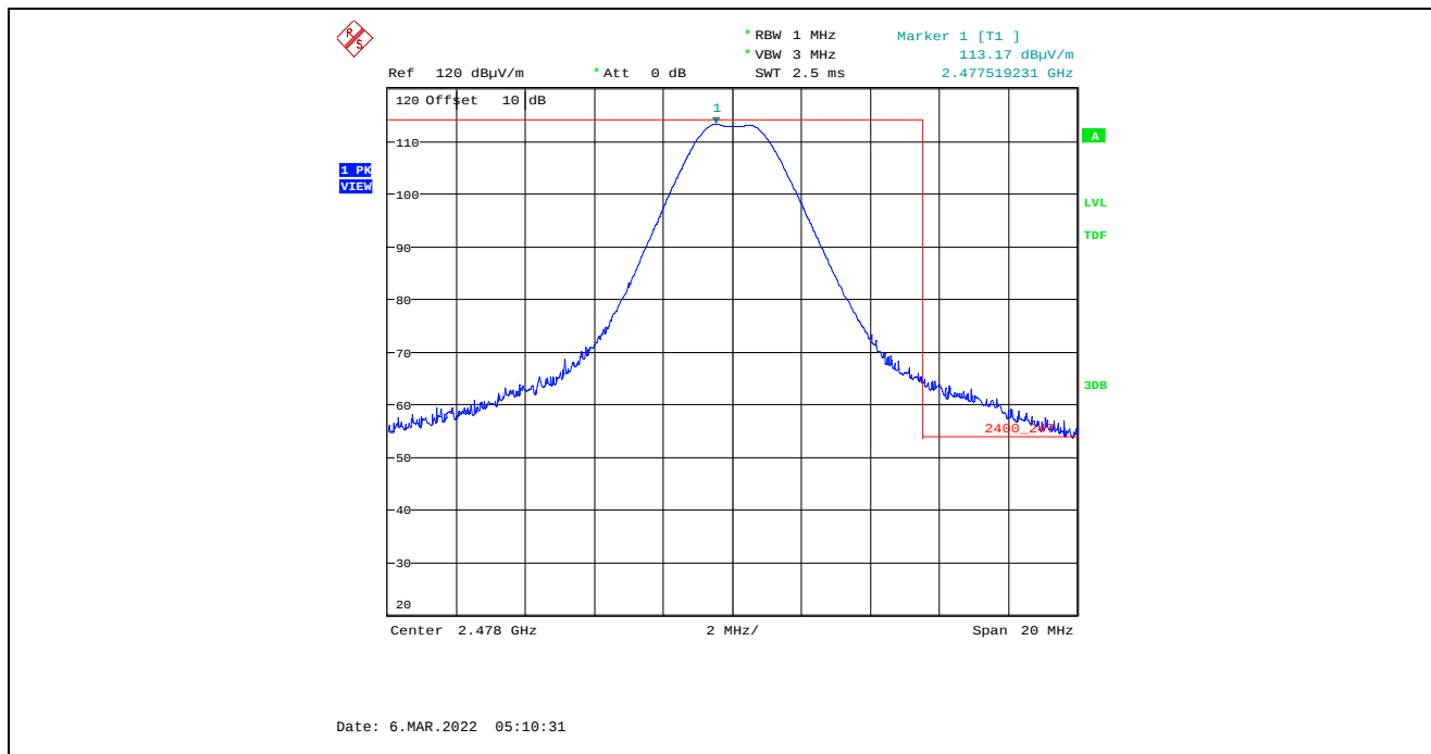
Plot 5.4.4.6.2.7. Band-Edge RF Radiated Emissions at 3 m, Vertical Polarization, Peak High End of Frequency Band, 2478 MHz, 8 dBm Power Setting, 2 Mbps
