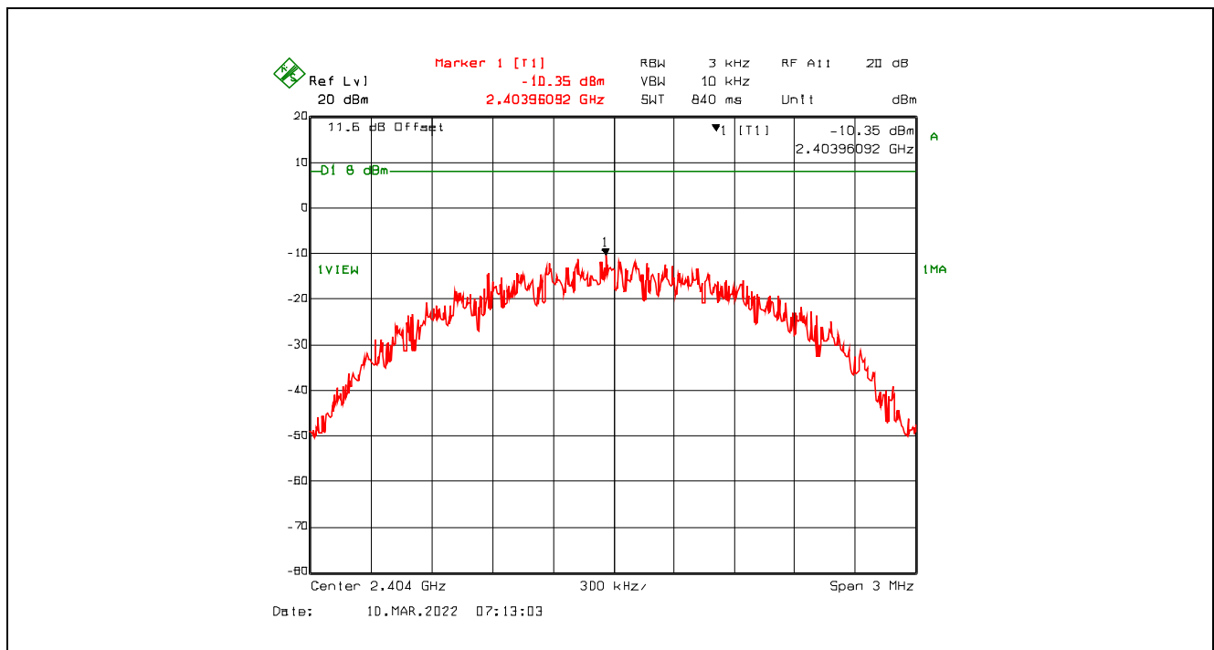
Plot 5.5.4.4. Power Spectral Density, GFSK Modulation, 2 Mbps, 8 dBm Power Setting, 2404 MHz
