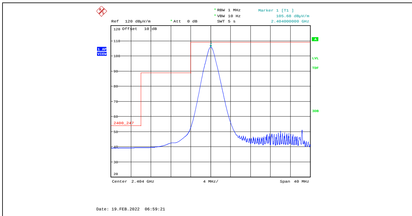
Plot 5.4.4.5.2.4. Band-Edge RF Radiated Emissions at 3 m, Vertical Polarization, Average Low End of Frequency Band, 2404 MHz, 8 dBm Power Setting, 2 Mbps
