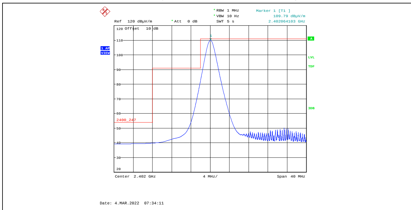
Plot 5.4.4.3.2.2. Band-Edge RF Radiated Emissions at 3 m, Horizontal Polarization, Average Low End of Frequency Band, 2402 MHz, 8 dBm Power Setting, 1 Mbps
