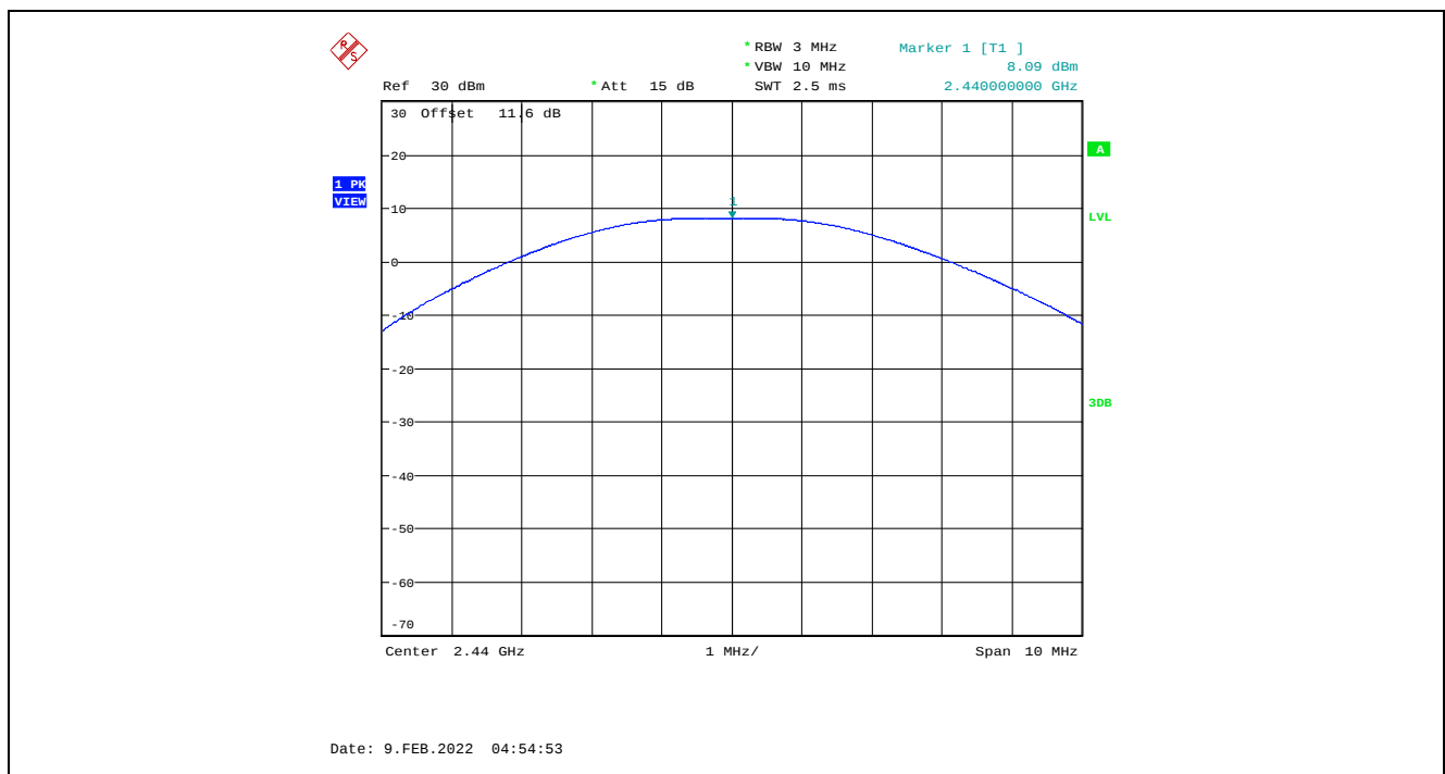
Plot 5.3.4.8. Maximum Peak Conducted Output Power, GFSK Modulation, 2 Mbps, 8 dBm Power Setting, 2440 MHz
