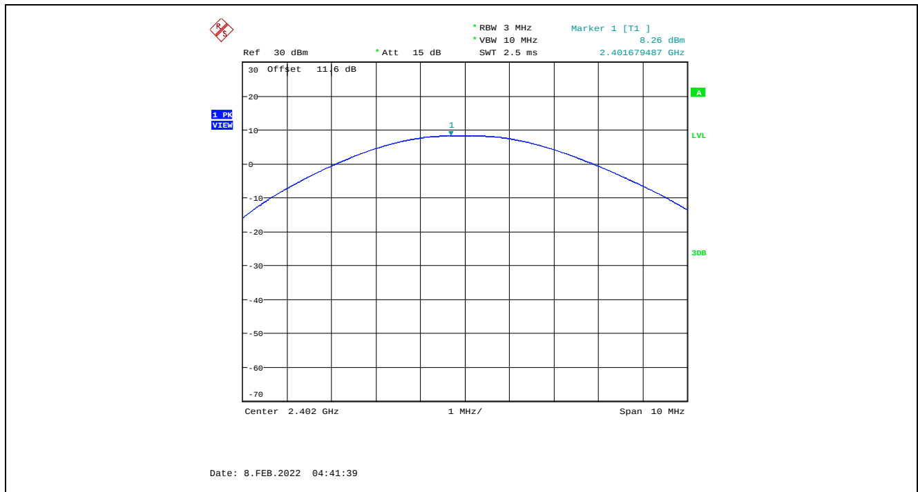
Plot 5.3.4.1. Maximum Peak Conducted Output Power, GFSK Modulation, 1 Mbps, 8 dBm Power Setting, 2402 MHz
