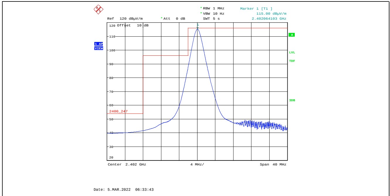
Plot 5.4.4.4.2.2. Band-Edge RF Radiated Emissions at 3 m, Horizontal Polarization, Average Low End of Frequency Band, 2402 MHz, 8 dBm Power Setting, 1 Mbps
