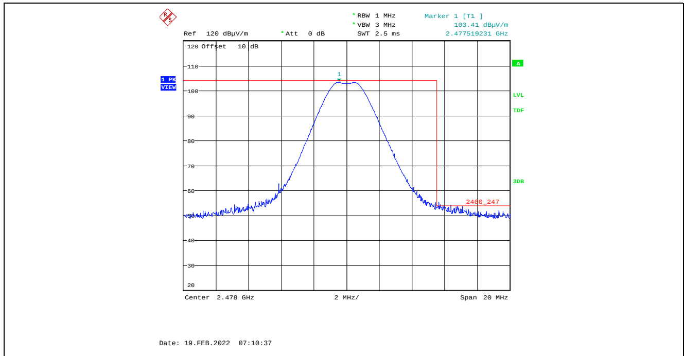
Plot 5.4.4.5.2.7. Band-Edge RF Radiated Emissions at 3 m, Vertical Polarization, Peak High End of Frequency Band, 2478 MHz, 8 dBm Power Setting, 2 Mbps
