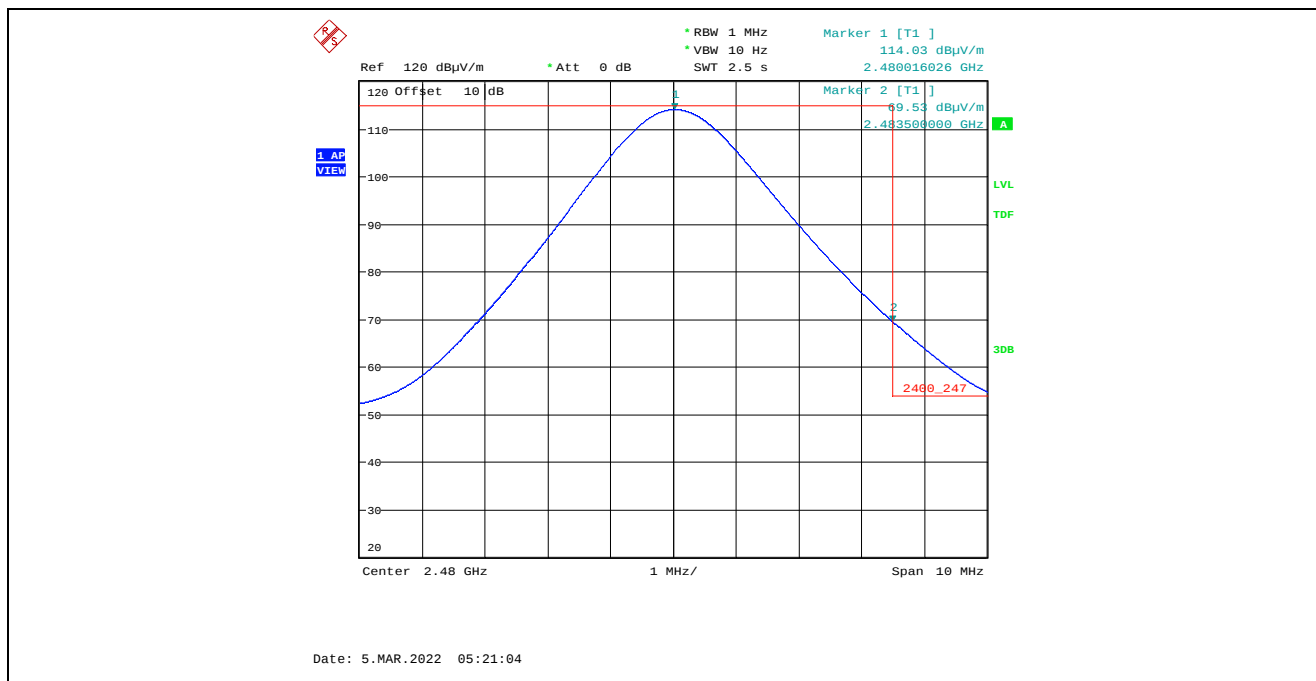
Plot 5.4.4.4.2.8. Band-Edge RF Radiated Emissions at 3 m, Vertical Polarization, Average High End of Frequency Band, 2480 MHz, 8 dBm Power Setting, 1 Mbps Marker 2: 69.53 dBμV/m – 33.36 dB Duty Cycle Factor = 36.17 dBμV/m (Limit 54 dBμV/m)
