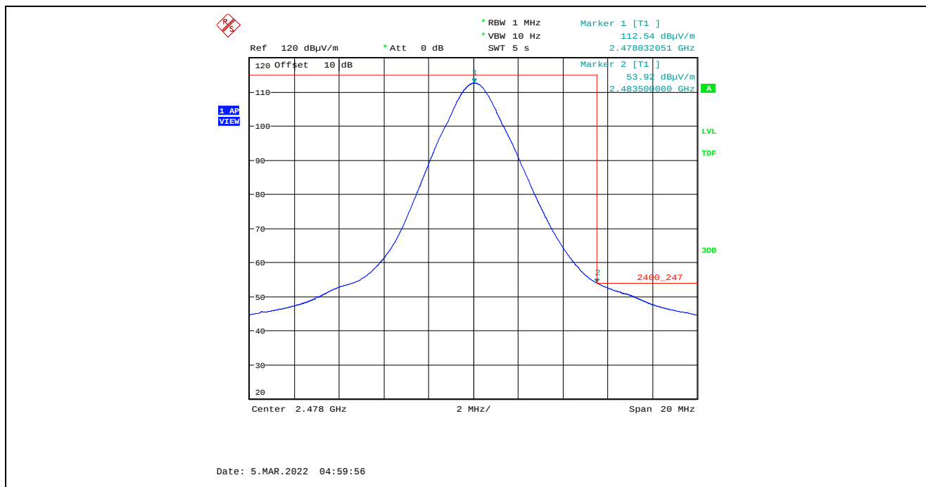
Plot 5.4.4.8.2.8. Band-Edge RF Radiated Emissions at 3 m, Vertical Polarization, Average High End of Frequency Band, 2478 MHz, 8 dBm Power Setting, 2 Mbps
