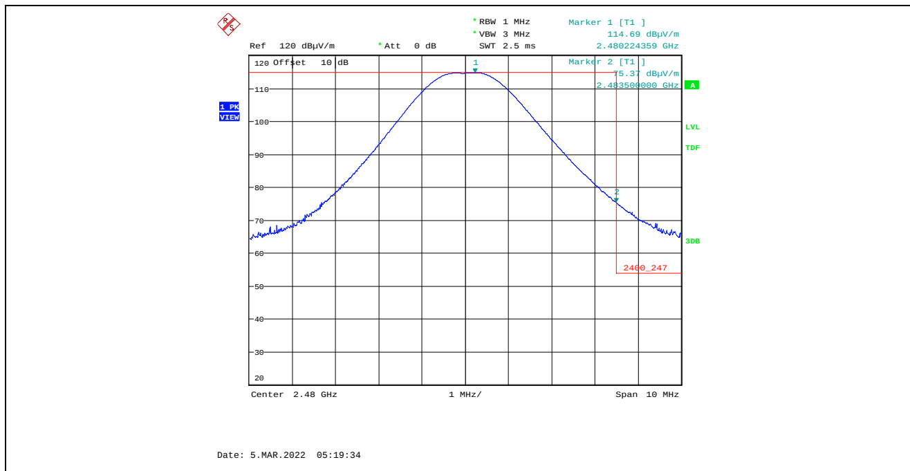
Plot 5.4.4.4.2.7. Band-Edge RF Radiated Emissions at 3 m, Vertical Polarization, Peak High End of Frequency Band, 2480 MHz, 8 dBm Power Setting, 1 Mbps
