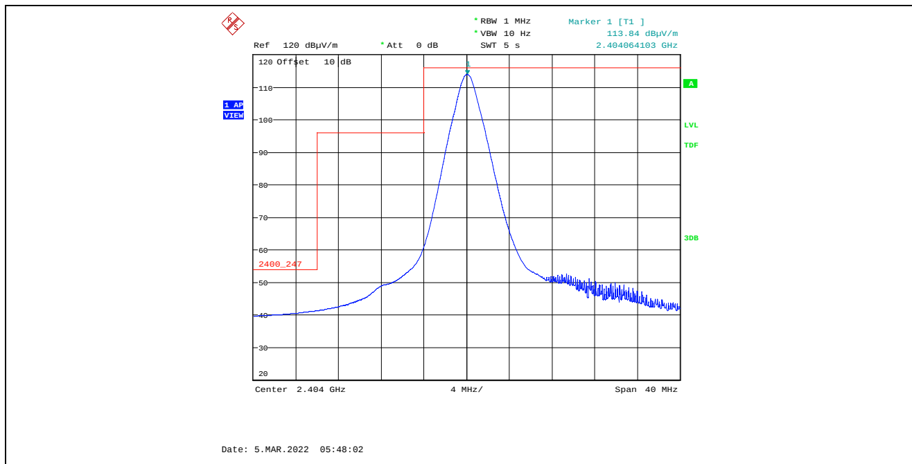
Plot 5.4.4.8.2.2. Band-Edge RF Radiated Emissions at 3 m, Horizontal Polarization, Average Low End of Frequency Band, 2404 MHz, 8 dBm Power Setting, 2 Mbps
