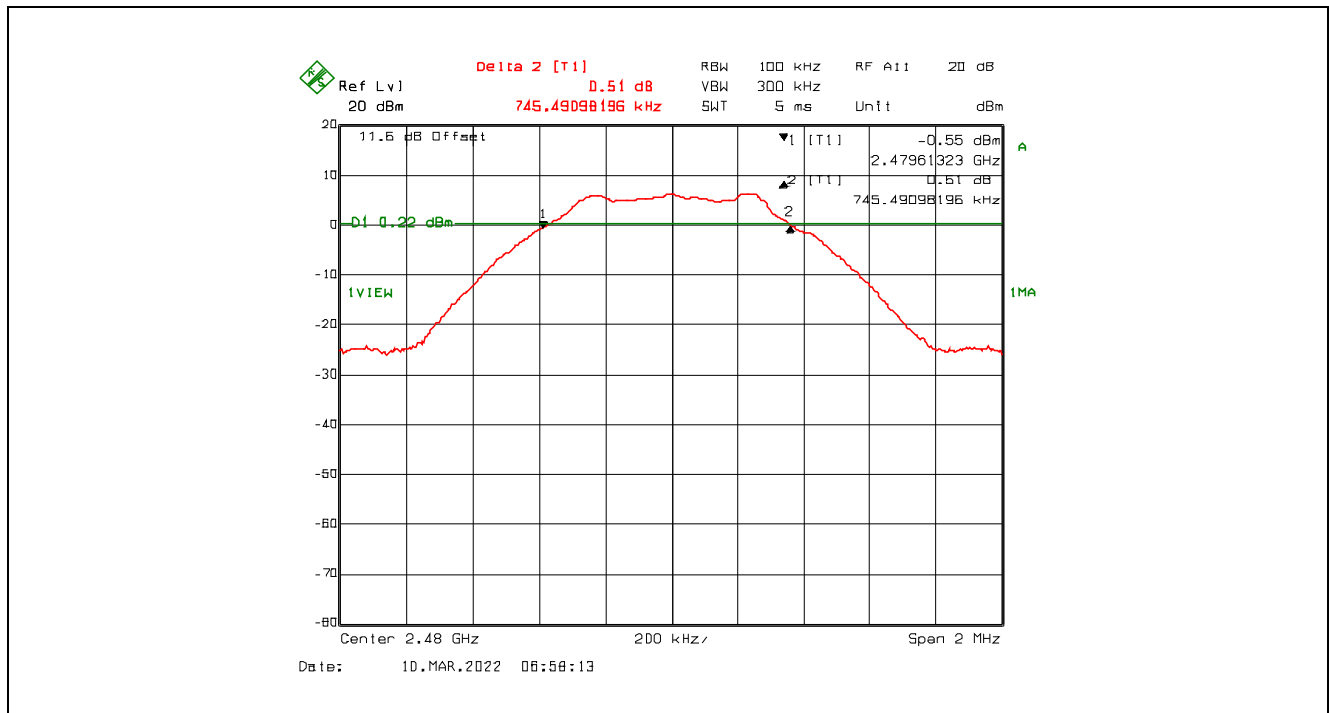
Plot 5.2.4.3. 6 dB Bandwidth, GFSK Modulation, 8 dBm Power Setting, 1 Mbps, 2480 MHz
