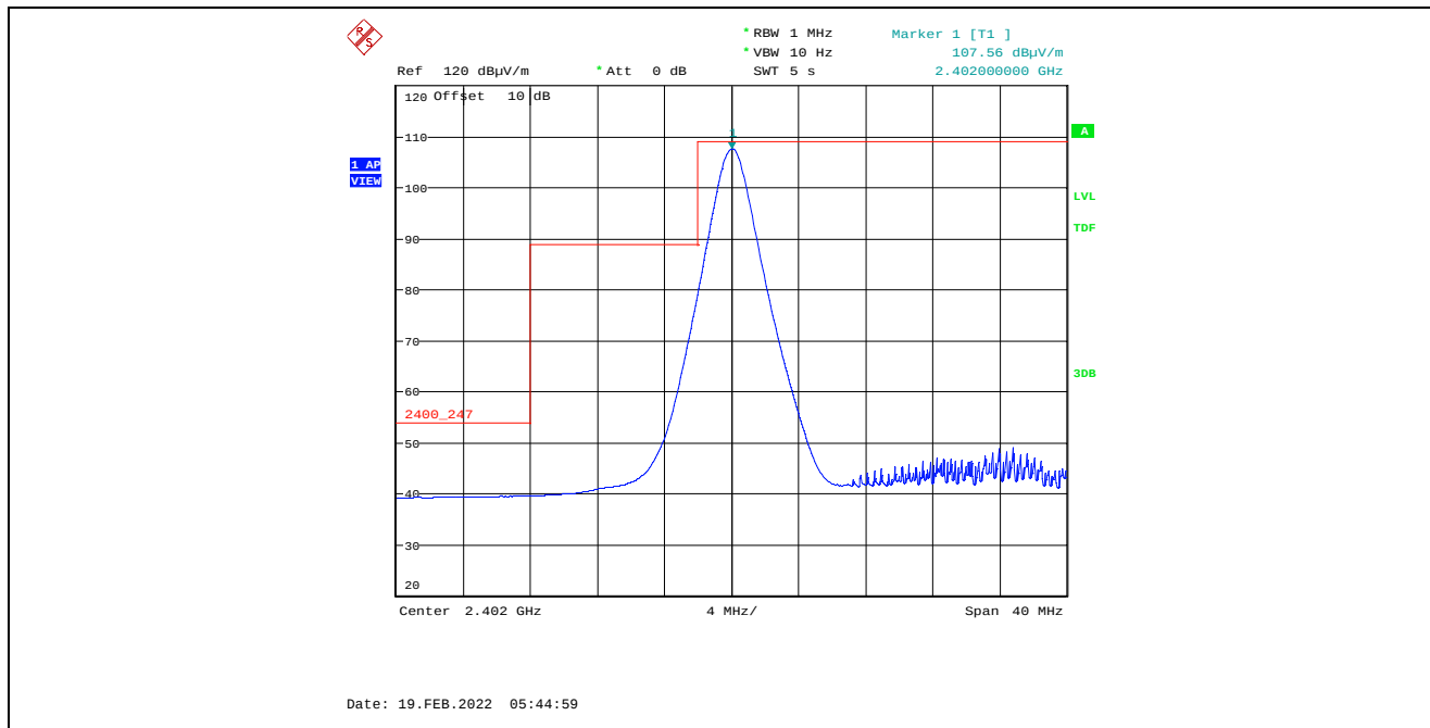
Plot 5.4.4.1.2.2. Band-Edge RF Radiated Emissions at 3 m, Horizontal Polarization, Average Low End of Frequency Band, 2402 MHz, 8 dBm Power Setting, 1 Mbps
