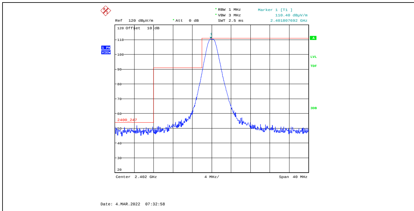
Plot 5.4.4.3.2.1. Band-Edge RF Radiated Emissions at 3 m, Horizontal Polarization, Peak Low End of Frequency Band, 2402 MHz, 8 dBm Power Setting, 1 Mbps
