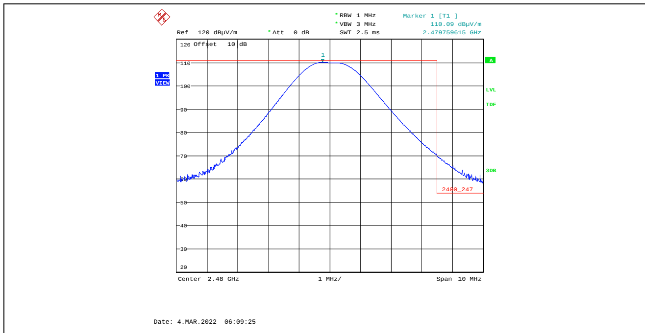
Plot 5.4.4.3.2.7. Band-Edge RF Radiated Emissions at 3 m, Vertical Polarization, Peak High End of Frequency Band, 2480 MHz, 8 dBm Power Setting, 1 Mbps
