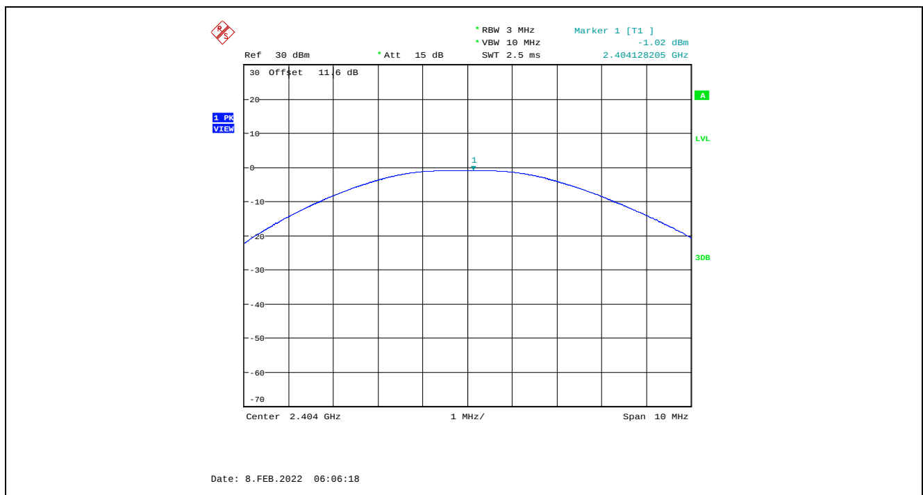
Plot 5.3.4.10. Maximum Peak Conducted Output Power, GFSK Modulation, 2 Mbps, -2 dBm Power Setting, 2404 MHz
