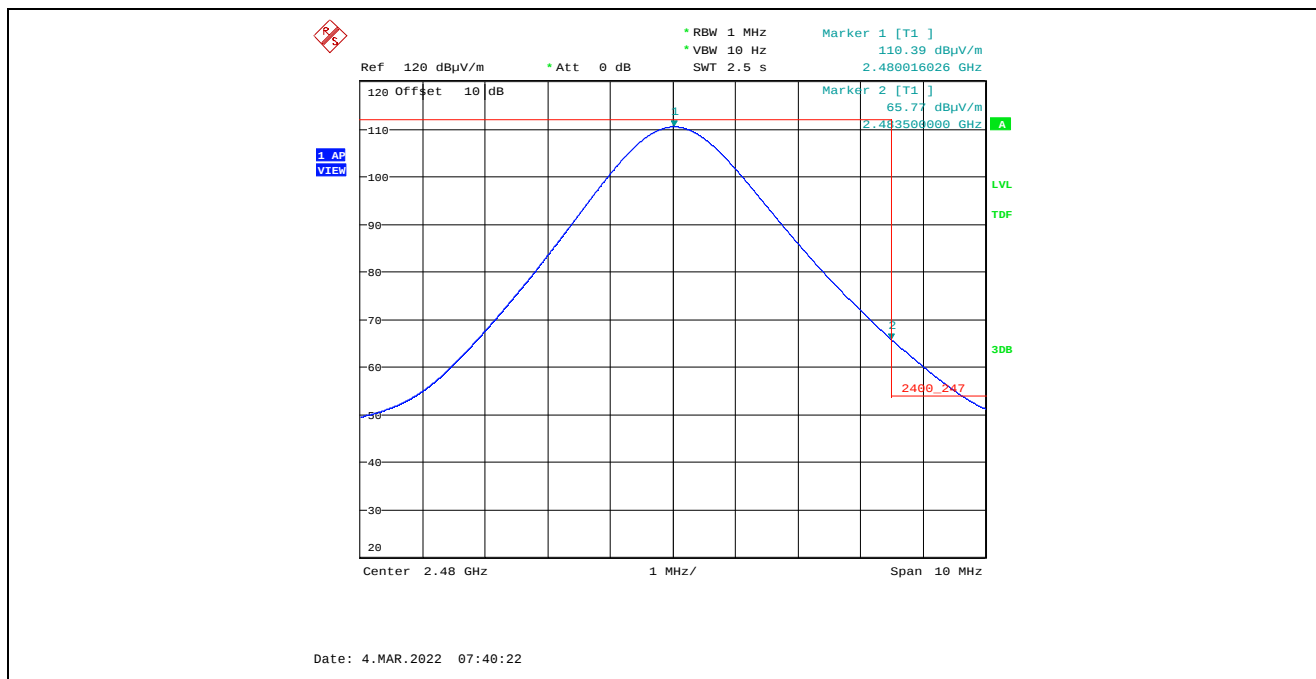
Plot 5.4.4.3.2.6. Band-Edge RF Radiated Emissions at 3 m, Horizontal Polarization, Average High End of Frequency Band, 2480 MHz, 8 dBm Power Setting, 1 Mbps Marker 2: 65.77 dBμV/m – 33.36 dB Duty Cycle Factor = 32.41 dBμV/m (Limit 54 dBμV/m)
