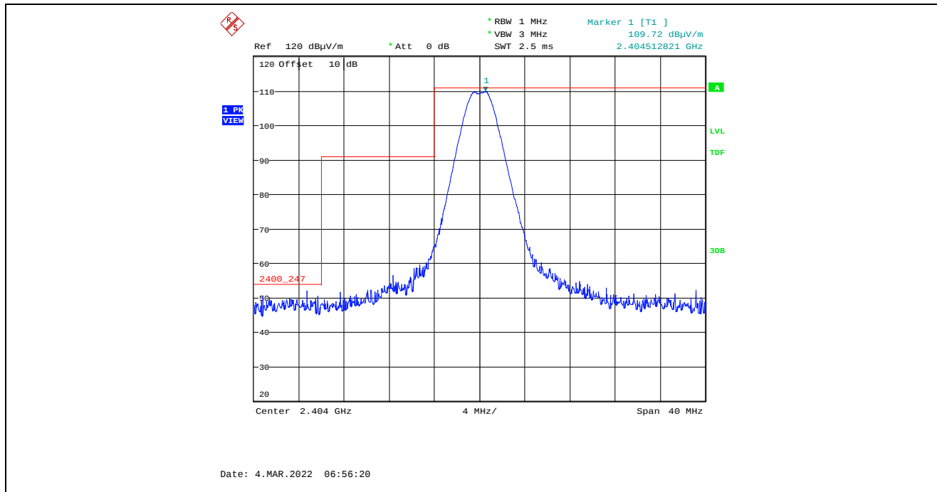
Plot 5.4.4.7.2.3. Band-Edge RF Radiated Emissions at 3 m, Vertical Polarization, Peak Low End of Frequency Band, 2404 MHz, 8 dBm Power Setting, 2 Mbps
