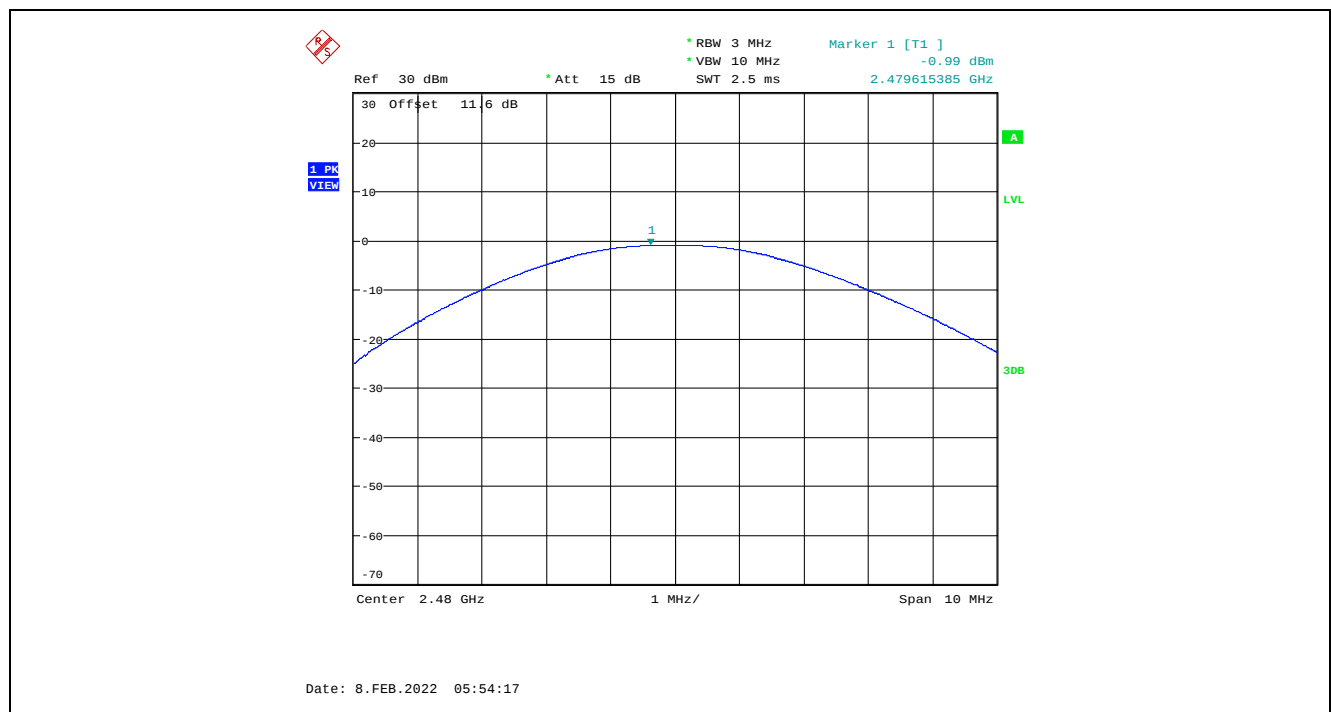
Plot 5.3.4.6. Maximum Peak Conducted Output Power, GFSK Modulation, 1 Mbps, -2 dBm Power Setting, 2480 MHz
