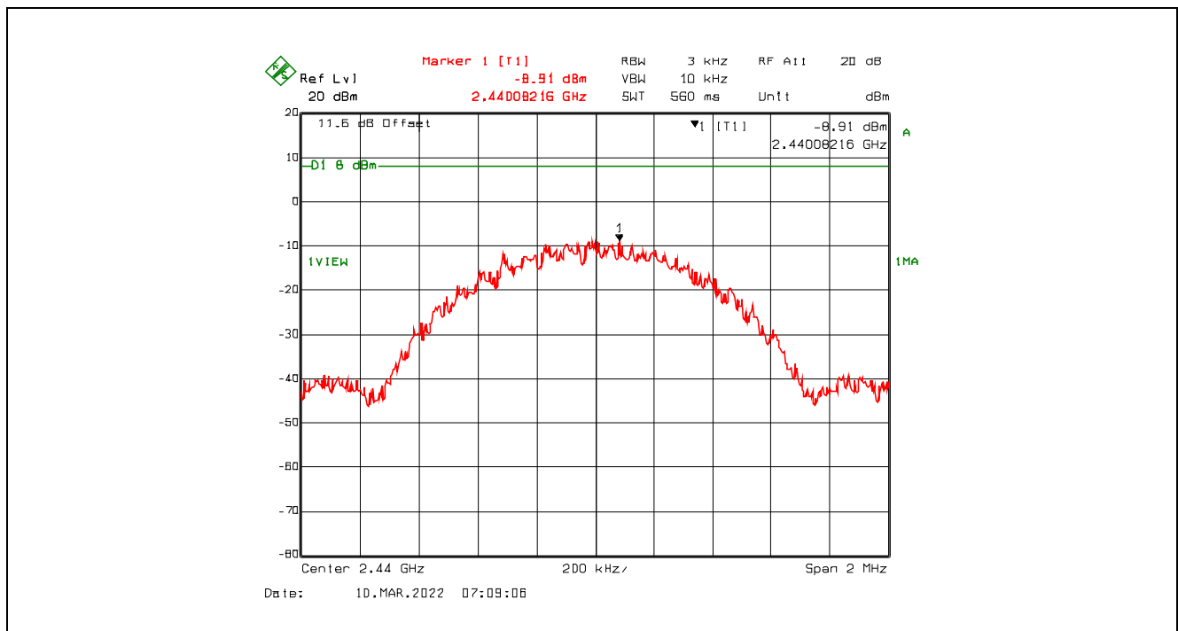
Plot 5.5.4.2. Power Spectral Density, GFSK Modulation, 1 Mbps, 8 dBm Power Setting, 2440 MHz
