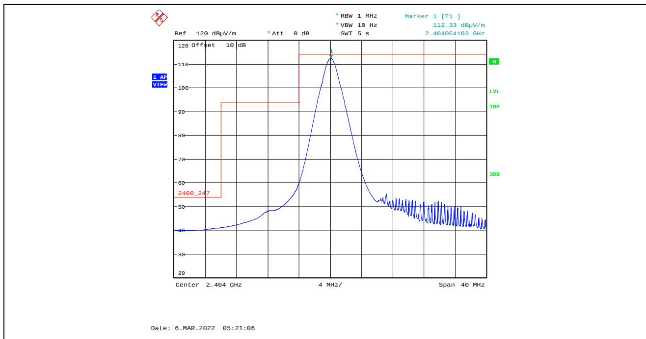
Plot 5.4.4.6.2.4. Band-Edge RF Radiated Emissions at 3 m, Vertical Polarization, Average Low End of Frequency Band, 2404 MHz, 8 dBm Power Setting, 2 Mbps
