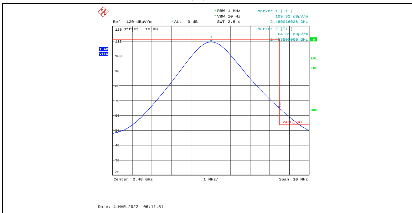
Plot 5.4.4.3.2.8. Band-Edge RF Radiated Emissions at 3 m, Vertical Polarization, Average High End of Frequency Band, 2480 MHz, 8 dBm Power Setting, 1 Mbps Marker 2: 64.83 dBμV/m – 33.36 dB Duty Cycle Factor = 31.47 dBμV/m (Limit 54 dBμV/m)
