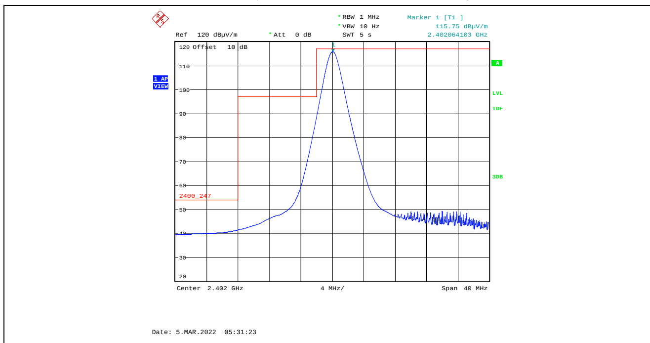
Plot 5.4.4.4.2.4. Band-Edge RF Radiated Emissions at 3 m, Vertical Polarization, Average Low End of Frequency Band, 2402 MHz, 8 dBm Power Setting, 1 Mbps
