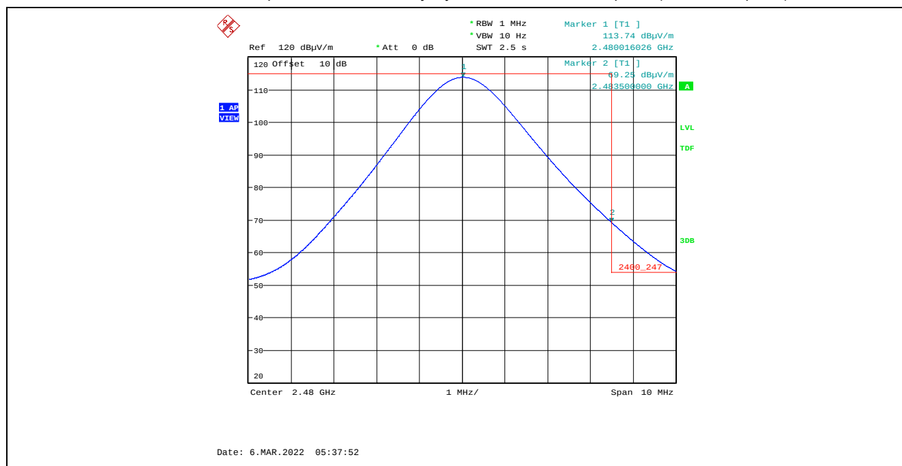
Plot 5.4.4.2.8. Band-Edge RF Radiated Emissions at 3 m, Vertical Polarization, Average High End of Frequency Band, 2480 MHz, 8 dBm Power Setting, 1 Mbps Marker 2: 69.25 dBμV/m – 33.36 dB Duty Cycle Factor = 35.89 dBμV/m (Limit 54 dBμV/m)
