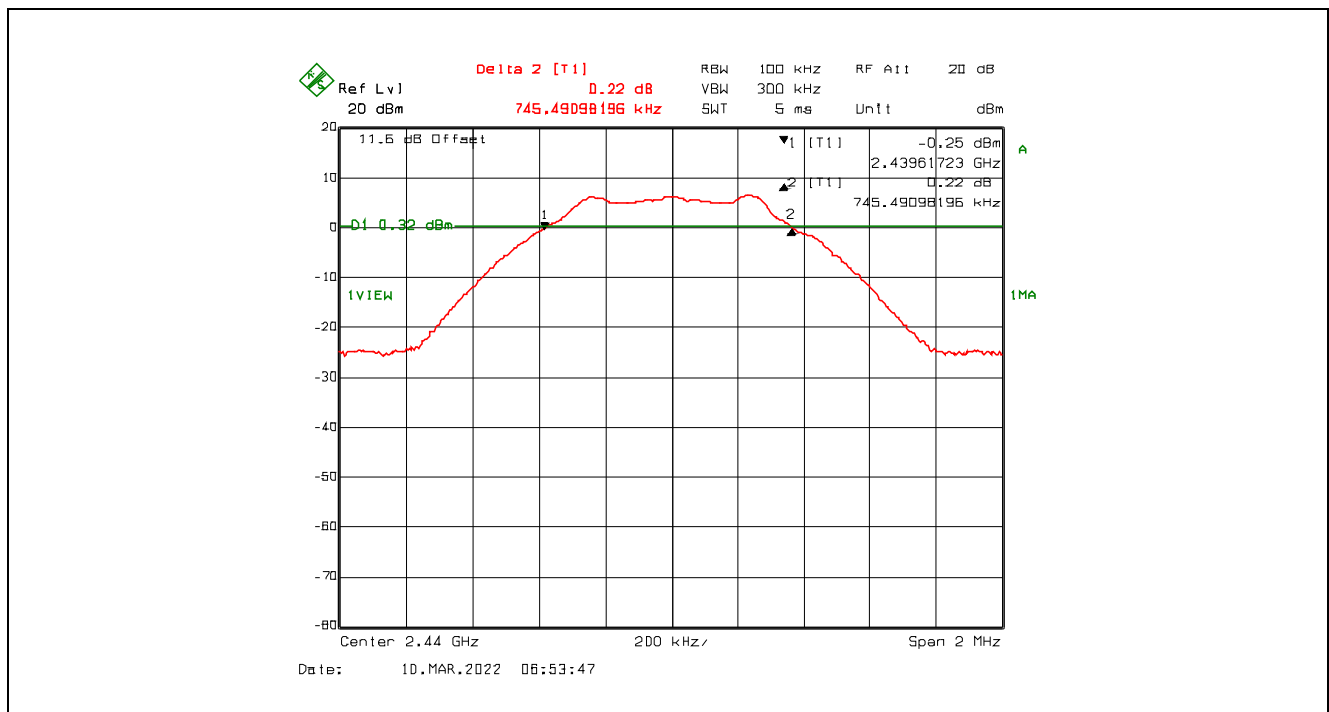
Plot 5.2.4.2. 6 dB Bandwidth, GFSK Modulation, 8 dBm Power Setting, 1 Mbps, 2440 MHz
