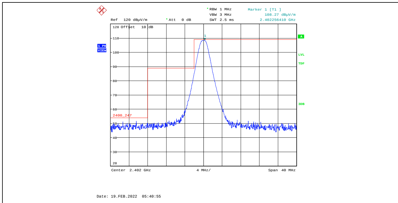
Plot 5.4.4.1.2.1. Band-Edge RF Radiated Emissions at 3 m, Horizontal Polarization, Peak Low End of Frequency Band, 2402 MHz, 8 dBm Power Setting, 1 Mbps
