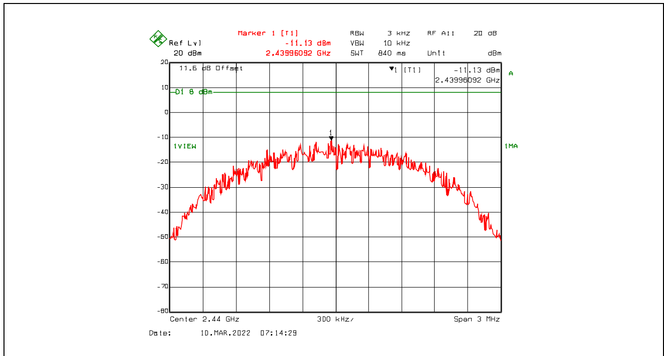
Plot 5.5.4.5. Power Spectral Density, GFSK Modulation, 2 Mbps, 8 dBm Power Setting, 2440 MHz
