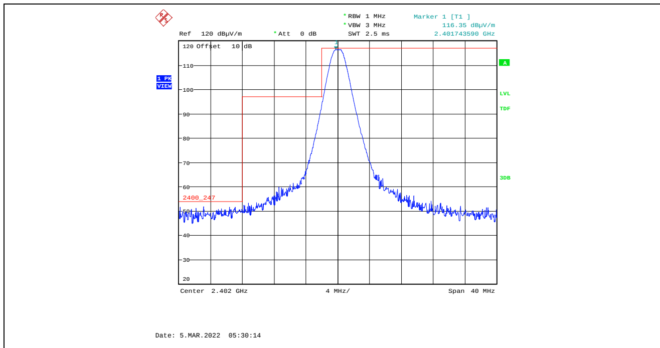
Plot 5.4.4.4.2.3. Band-Edge RF Radiated Emissions at 3 m, Vertical Polarization, Peak Low End of Frequency Band, 2402 MHz, 8 dBm Power Setting, 1 Mbps
