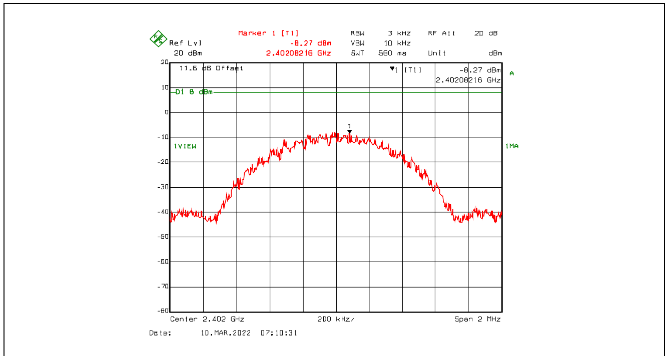
Plot 5.5.4.1. Power Spectral Density, GFSK Modulation, 1 Mbps, 8 dBm Power Setting, 2402 MHz
