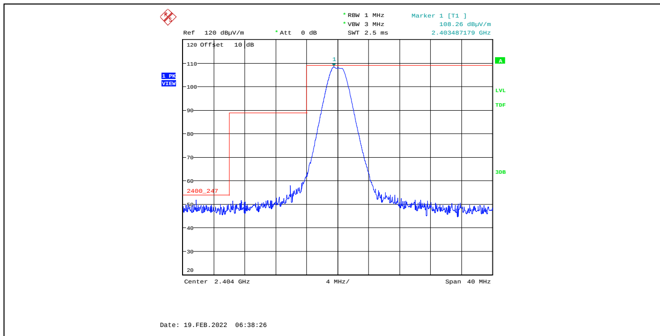
Plot 5.4.4.5.2.1. Band-Edge RF Radiated Emissions at 3 m, Horizontal Polarization, Peak Low End of Frequency Band, 2404 MHz, 8 dBm Power Setting, 2 Mbps
