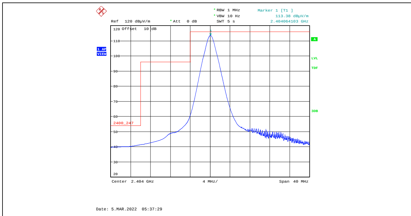
Plot 5.4.4.8.2.4. Band-Edge RF Radiated Emissions at 3 m, Vertical Polarization, Average Low End of Frequency Band, 2404 MHz, 8 dBm Power Setting, 2 Mbps
