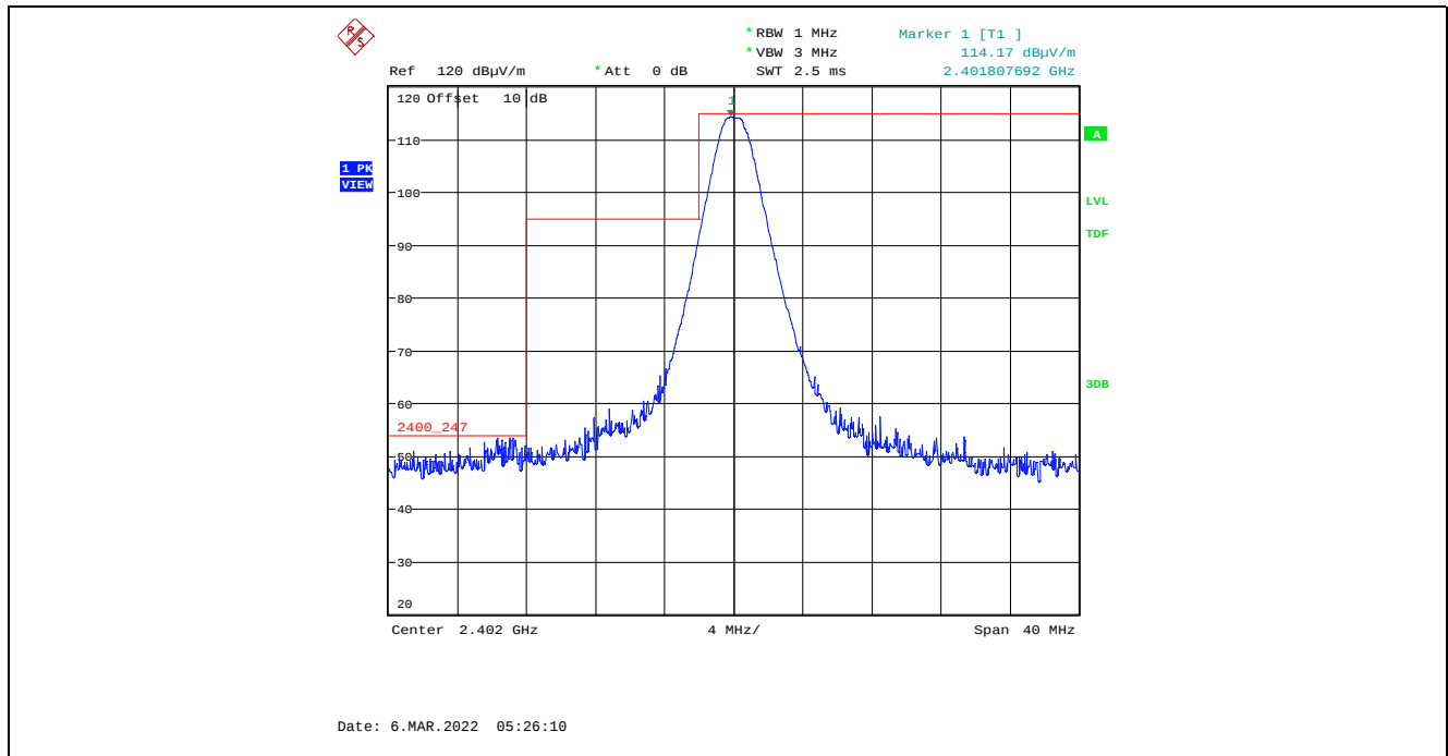
Plot 5.4.4.2.3. Band-Edge RF Radiated Emissions at 3 m, Vertical Polarization, Peak Low End of Frequency Band, 2402 MHz, 8 dBm Power Setting, 1 Mbps
