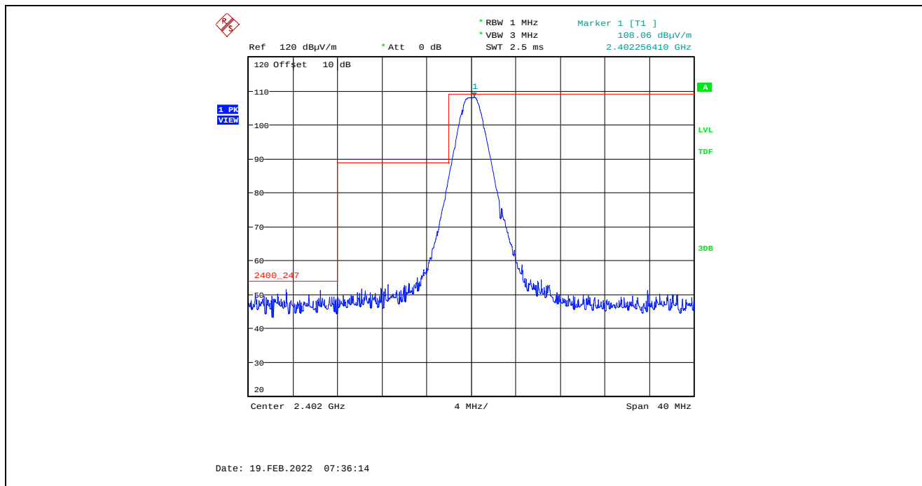
Plot 5.4.4.1.2.3. Band-Edge RF Radiated Emissions at 3 m, Vertical Polarization, Peak Low End of Frequency Band, 2402 MHz, 8 dBm Power Setting, 1 Mbps
