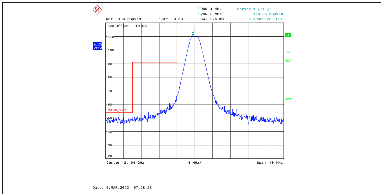
Plot 5.4.4.7.2.1. Band-Edge RF Radiated Emissions at 3 m, Horizontal Polarization, Peak Low End of Frequency Band, 2404 MHz, 8 dBm Power Setting, 2 Mbps
