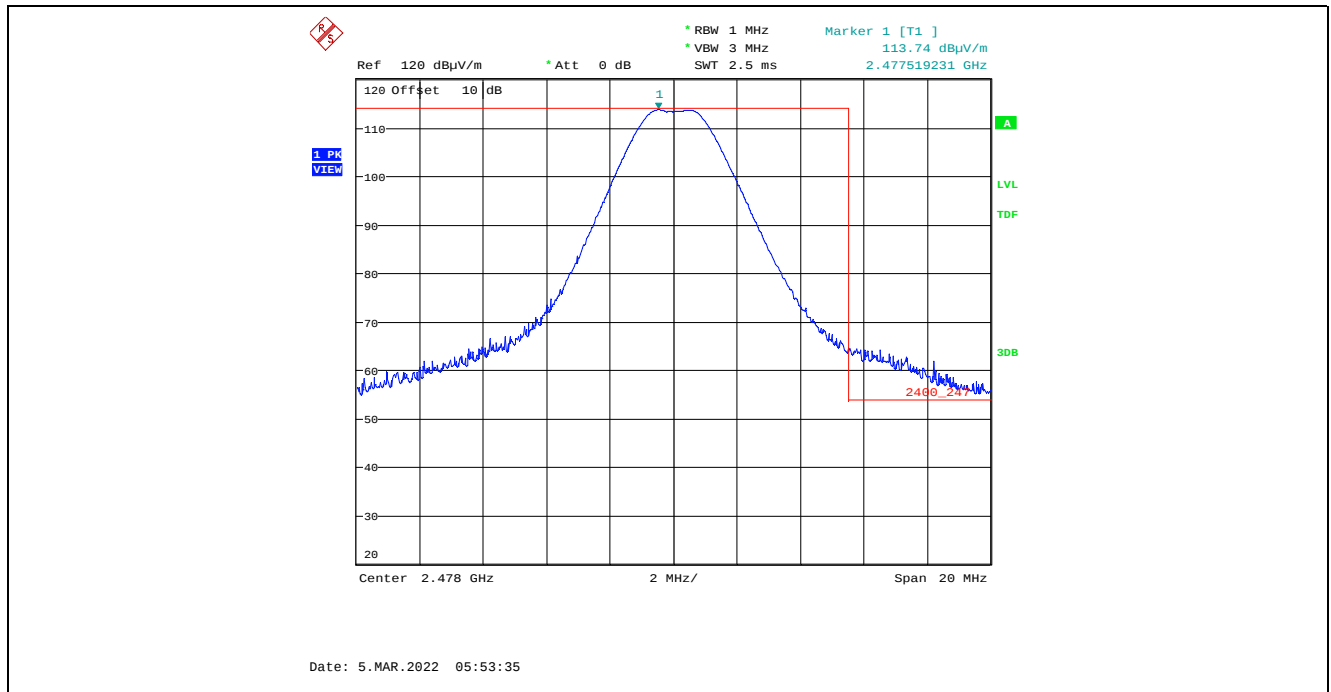
Plot 5.4.4.8.2.5. Band-Edge RF Radiated Emissions at 3 m, Horizontal Polarization, Peak High End of Frequency Band, 2478 MHz, 8 dBm Power Setting, 2 Mbps
