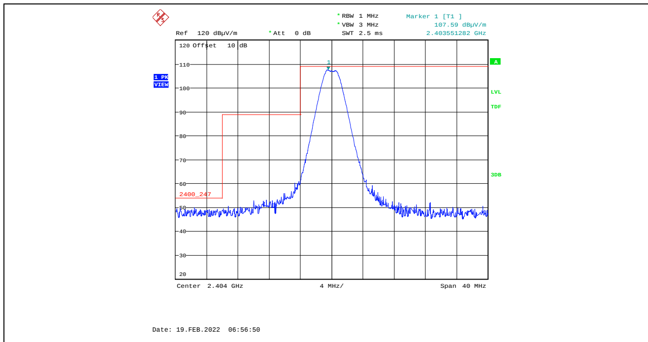
Plot 5.4.4.5.2.3. Band-Edge RF Radiated Emissions at 3 m, Vertical Polarization, Peak Low End of Frequency Band, 2404 MHz, 8 dBm Power Setting, 2 Mbps
