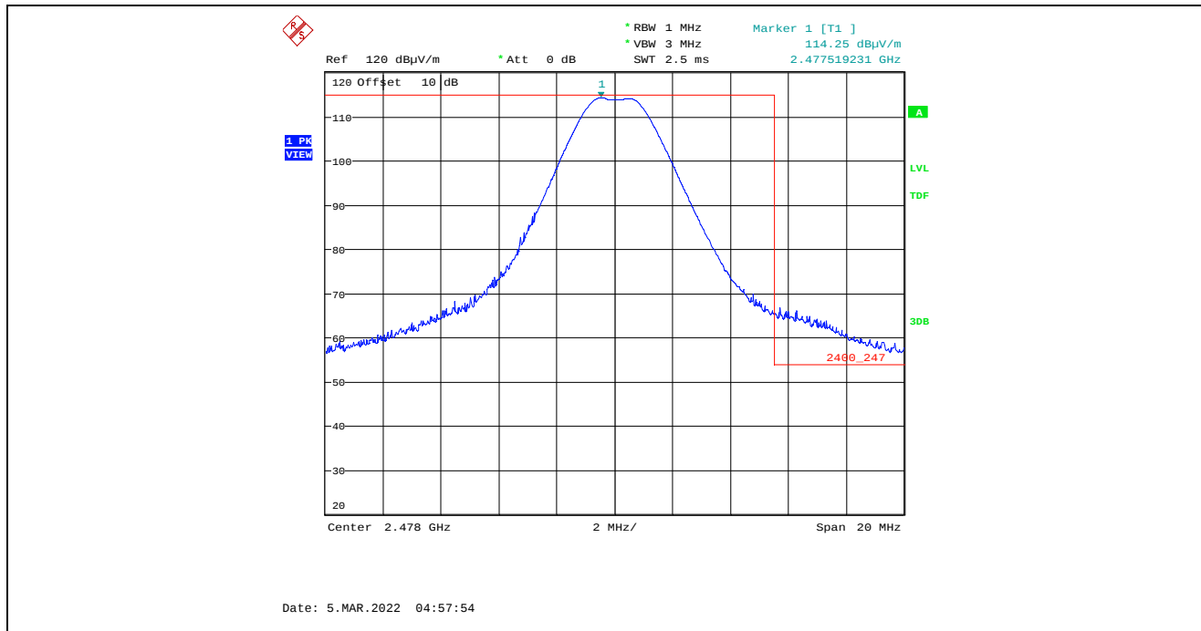
Plot 5.4.4.8.2.7. Band-Edge RF Radiated Emissions at 3 m, Vertical Polarization, Peak High End of Frequency Band, 2478 MHz, 8 dBm Power Setting, 2 Mbps
