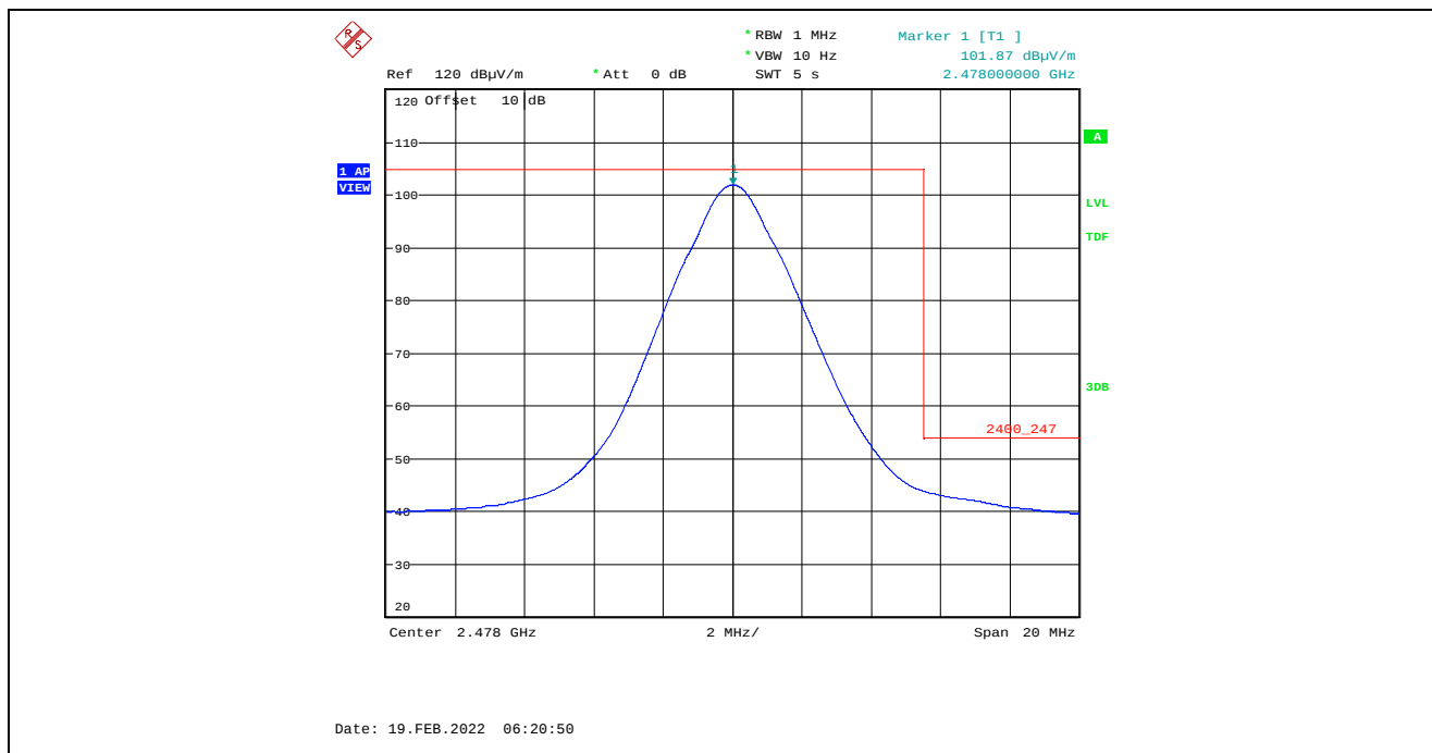
Plot 5.4.4.5.2.6. Band-Edge RF Radiated Emissions at 3 m, Horizontal Polarization, Average High End of Frequency Band, 2478 MHz, 8 dBm Power Setting, 2 Mbps
