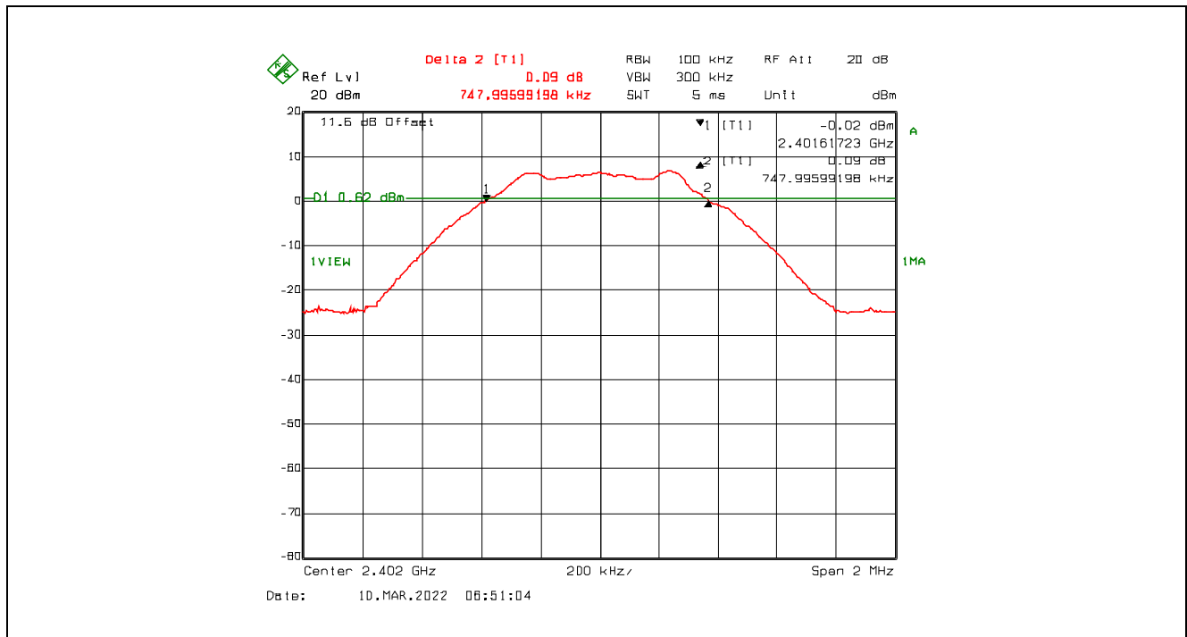
Plot 5.2.4.1. 6 dB Bandwidth, GFSK Modulation, 8 dBm Power Setting, 1 Mbps, 2402 MHz
