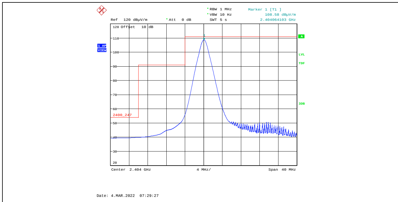
Plot 5.4.4.7.2.2. Band-Edge RF Radiated Emissions at 3 m, Horizontal Polarization, Average Low End of Frequency Band, 2404 MHz, 8 dBm Power Setting, 2 Mbps
