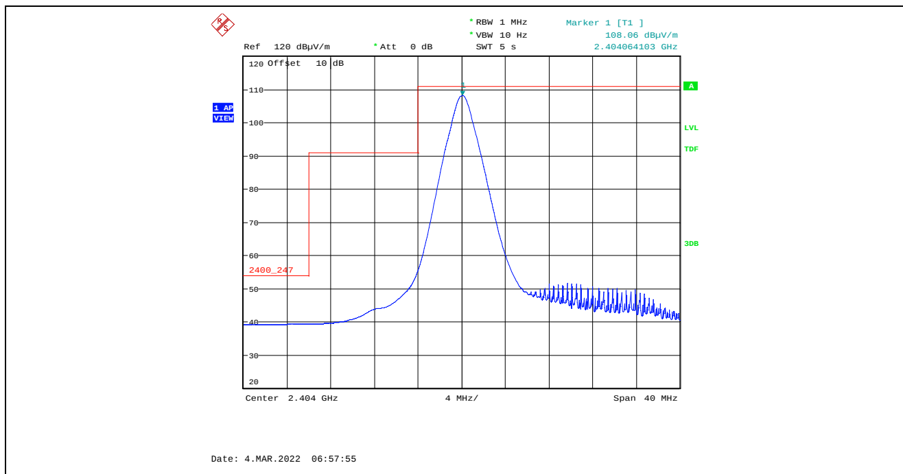
Plot 5.4.4.7.2.4. Band-Edge RF Radiated Emissions at 3 m, Vertical Polarization, Average Low End of Frequency Band, 2404 MHz, 8 dBm Power Setting, 2 Mbps
