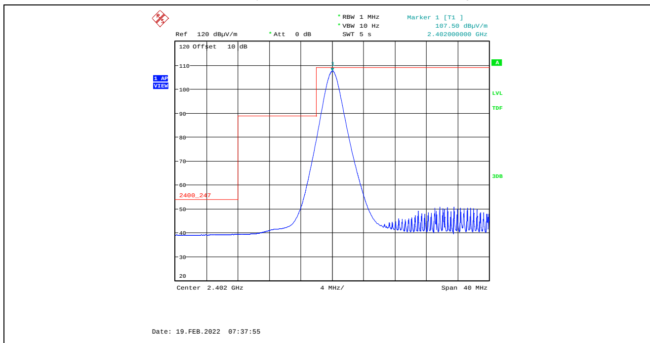
Plot 5.4.4.1.2.4. Band-Edge RF Radiated Emissions at 3 m, Vertical Polarization, Average Low End of Frequency Band, 2402 MHz, 8 dBm Power Setting, 1 Mbps
