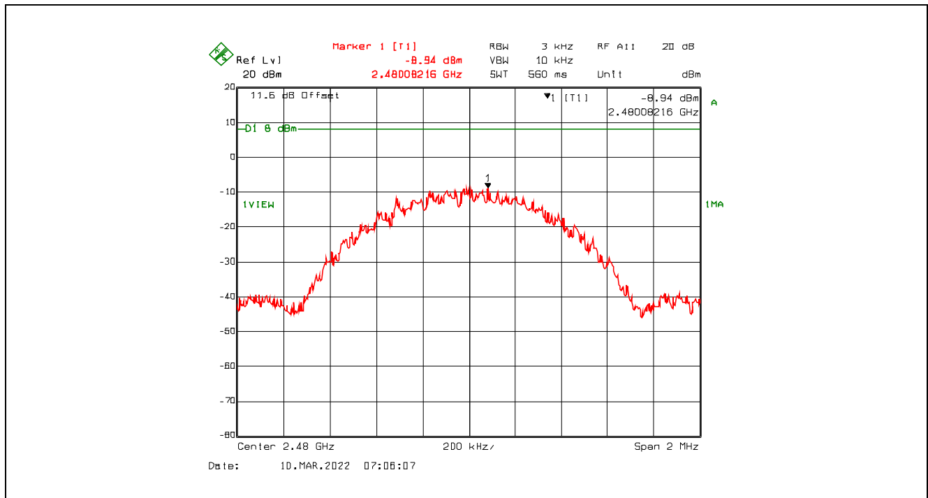
Plot 5.5.4.3. Power Spectral Density, GFSK Modulation, 1 Mbps, 8 dBm Power Setting, 2480 MHz
