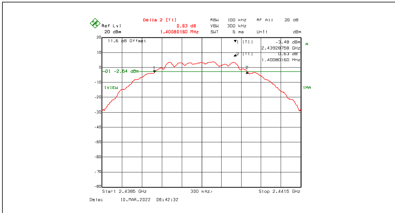
Plot 5.2.4.5. 6 dB Bandwidth, GFSK Modulation, 8 dBm Power Setting, 2 Mbps, 2440 MHz
