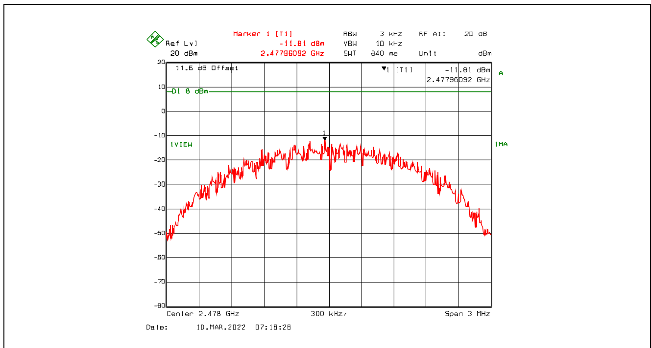
Plot 5.5.4.6. Power Spectral Density, GFSK Modulation, 2 Mbps, 8 dBm Power Setting, 2478 MHz
