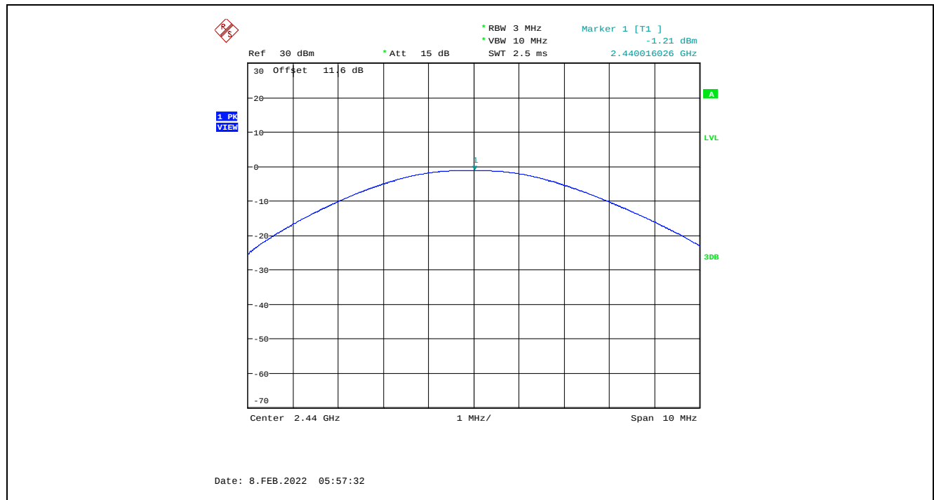
Plot 5.3.4.5. Maximum Peak Conducted Output Power, GFSK Modulation, 1 Mbps, -2 dBm Power Setting, 2440 MHz
