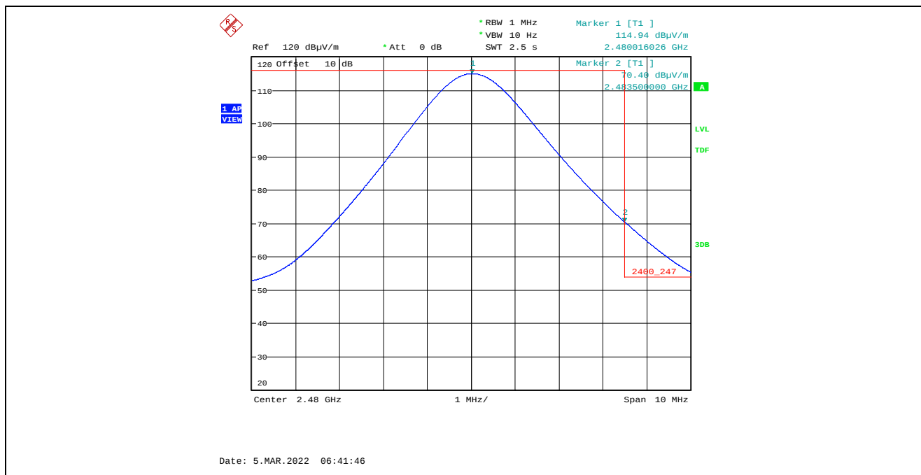
Plot 5.4.4.4.2.6. Band-Edge RF Radiated Emissions at 3 m, Horizontal Polarization, Average High End of Frequency Band, 2480 MHz, 8 dBm Power Setting, 1 Mbps Marker 2: 70.40 dBμV/m – 33.36 dB Duty Cycle Factor = 37.04 dBμV/m (Limit 54 dBμV/m)
