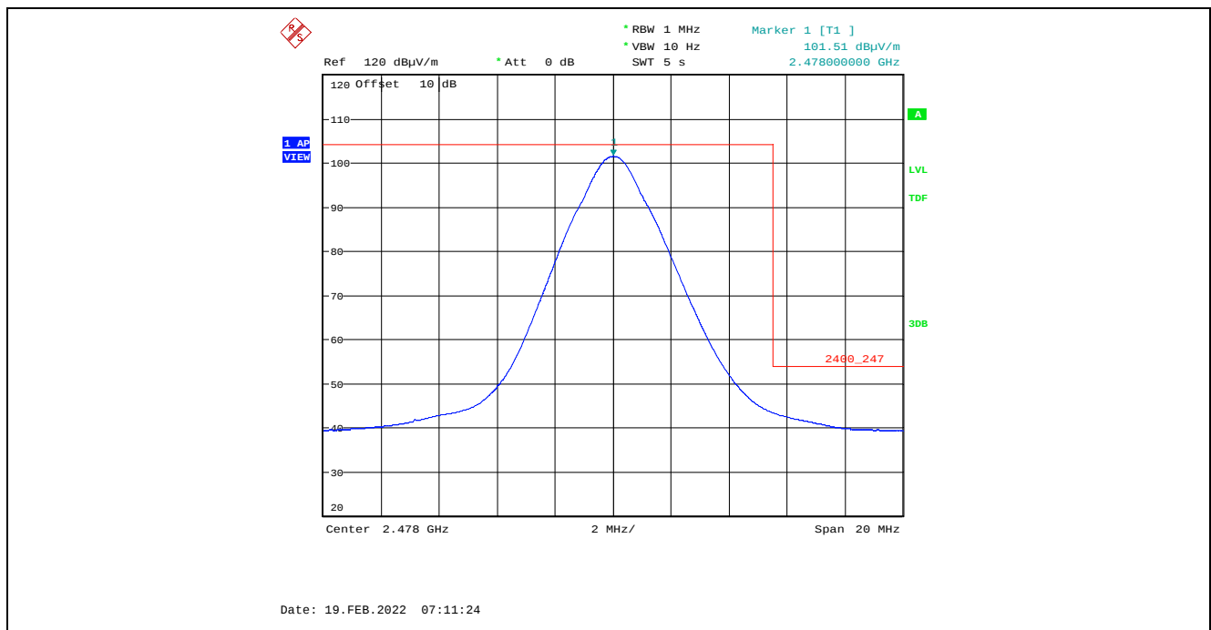
Plot 5.4.4.5.2.8. Band-Edge RF Radiated Emissions at 3 m, Vertical Polarization, Average High End of Frequency Band, 2478 MHz, 8 dBm Power Setting, 2 Mbps
