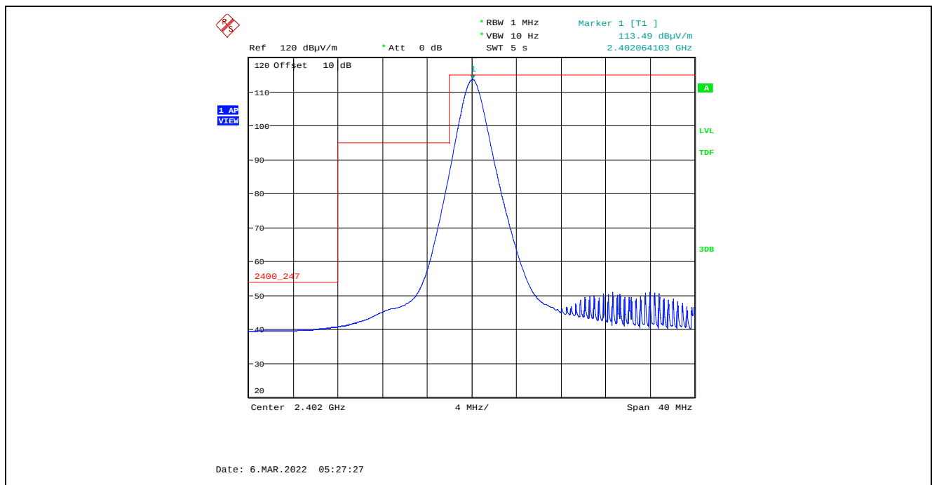
Plot 5.4.4.2.4. Band-Edge RF Radiated Emissions at 3 m, Vertical Polarization, Average Low End of Frequency Band, 2402 MHz, 8 dBm Power Setting, 1 Mbps
