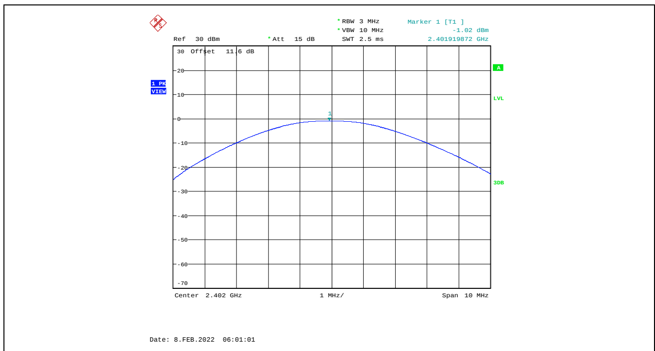
Plot 5.3.4.4. Maximum Peak Conducted Output Power, GFSK Modulation, 1 Mbps, -2 dBm Power Setting, 2402 MHz
