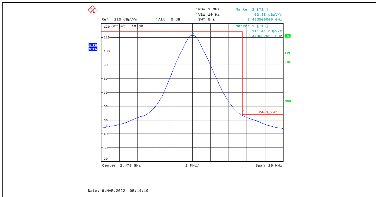
Plot 5.4.4.6.2.8. Band-Edge RF Radiated Emissions at 3 m, Vertical Polarization, Average High End of Frequency Band, 2478 MHz, 8 dBm Power Setting, 2 Mbps
