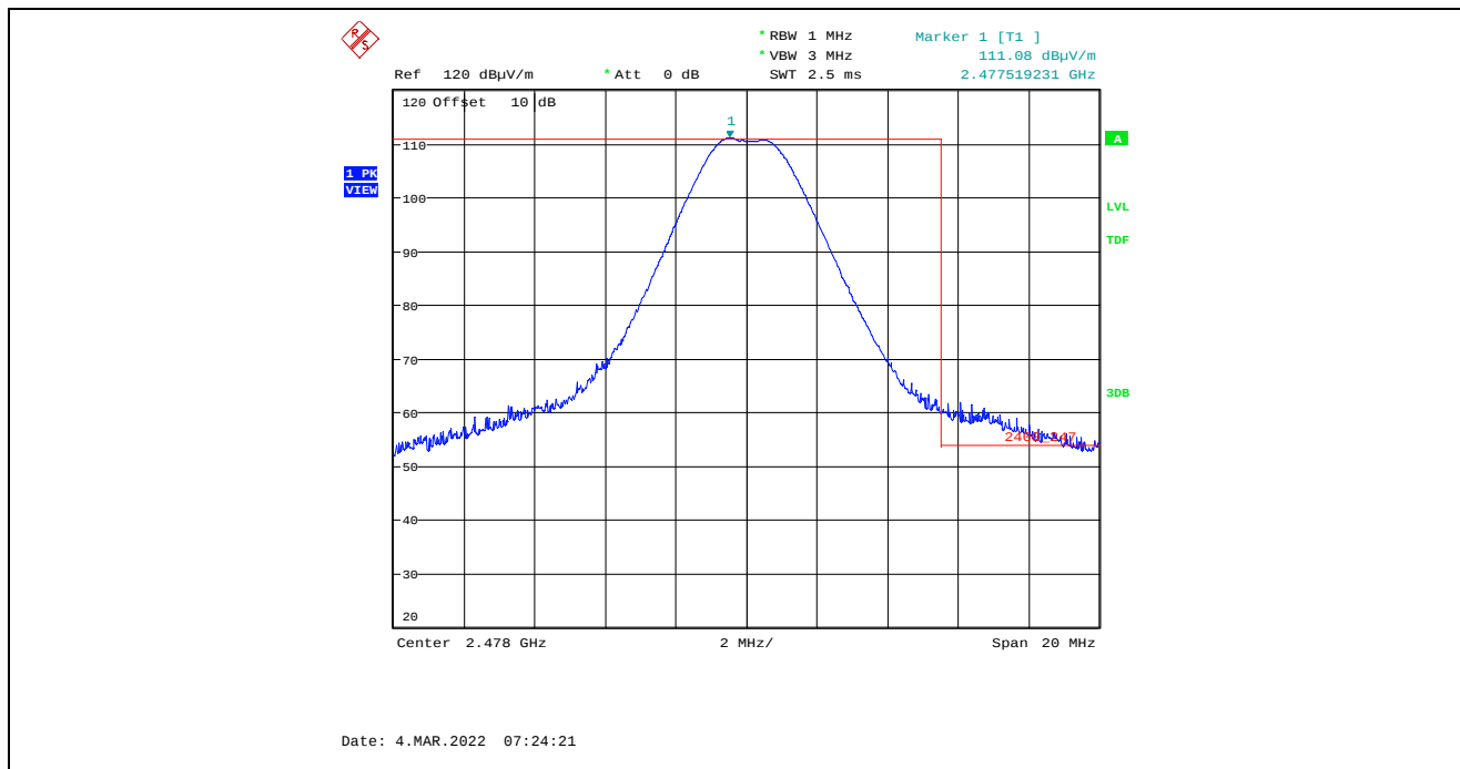
Plot 5.4.4.7.2.5. Band-Edge RF Radiated Emissions at 3 m, Horizontal Polarization, Peak High End of Frequency Band, 2478 MHz, 8 dBm Power Setting, 2 Mbps
