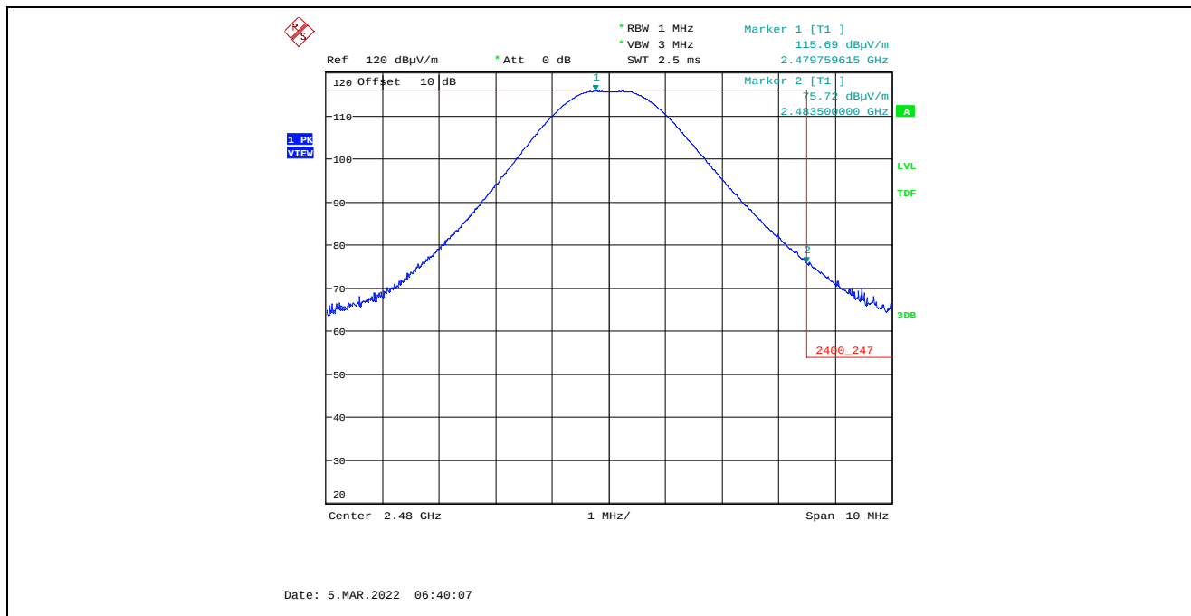
Plot 5.4.4.4.2.5. Band-Edge RF Radiated Emissions at 3 m, Horizontal Polarization, Peak High End of Frequency Band, 2480 MHz, 8 dBm Power Setting, 1 Mbps
