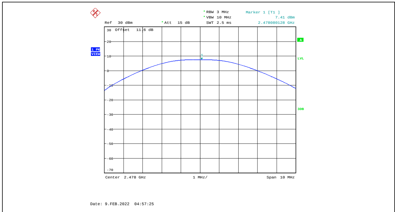
Plot 5.3.4.9. Maximum Peak Conducted Output Power, GFSK Modulation, 2 Mbps, 8 dBm Power Setting, 2478 MHz
