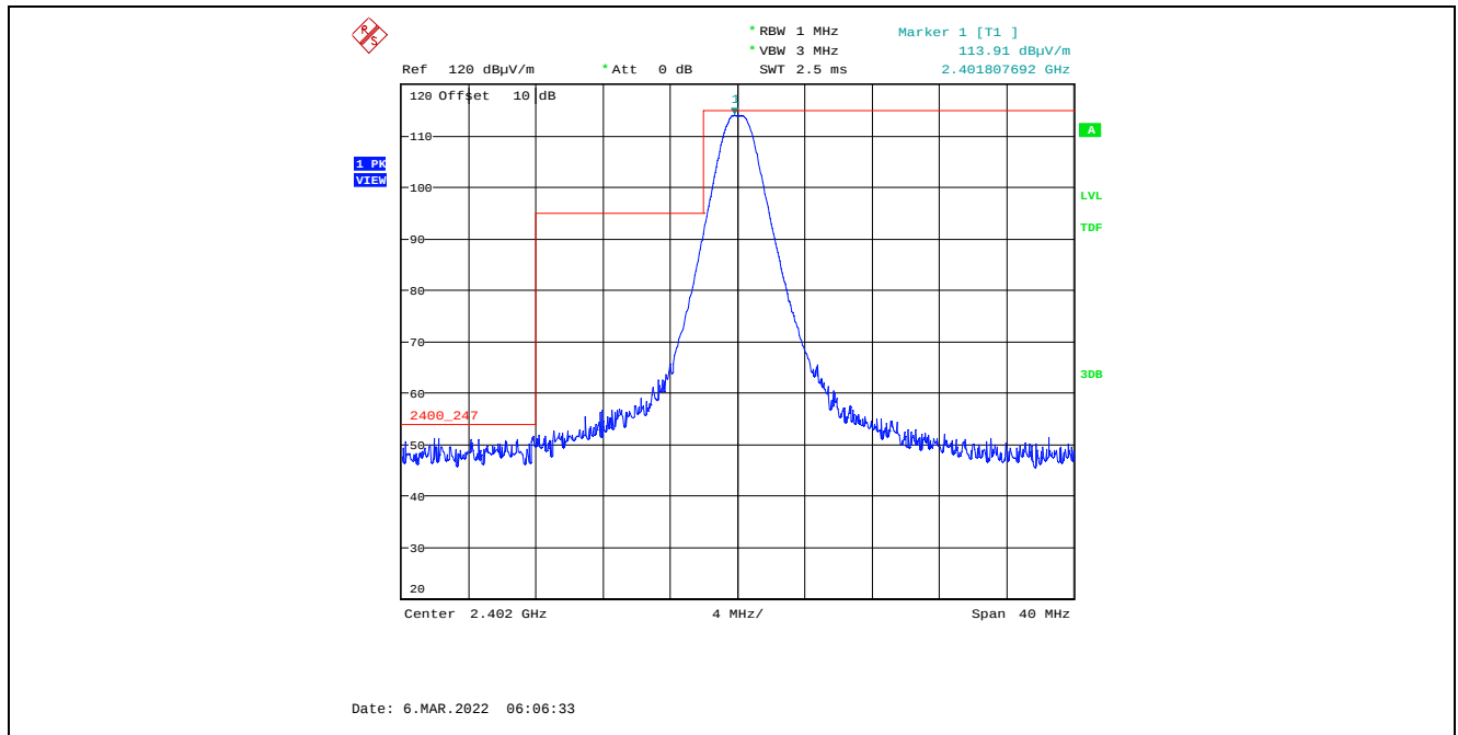
Plot 5.4.4.2.2.1. Band-Edge RF Radiated Emissions at 3 m, Horizontal Polarization, Peak Low End of Frequency Band, 2402 MHz, 8 dBm Power Setting, 1 Mbps
