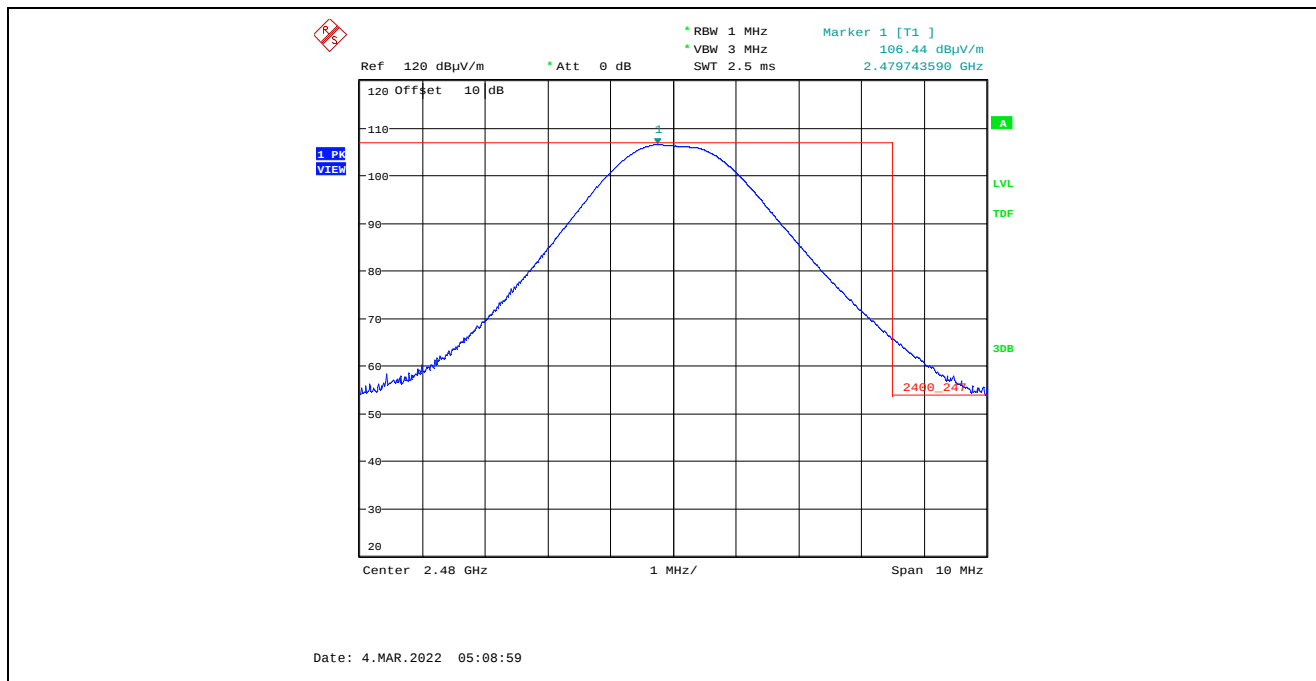
Plot 5.4.4.1.2.7. Band-Edge RF Radiated Emissions at 3 m, Vertical Polarization, Peak High End of Frequency Band, 2480 MHz, 8 dBm Power Setting, 1 Mbps
