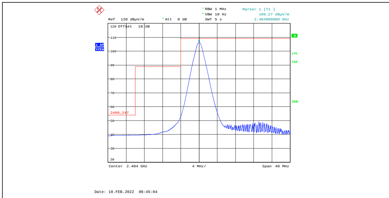
Plot 5.4.4.5.2.2. Band-Edge RF Radiated Emissions at 3 m, Horizontal Polarization, Average Low End of Frequency Band, 2404 MHz, 8 dBm Power Setting, 2 Mbps
