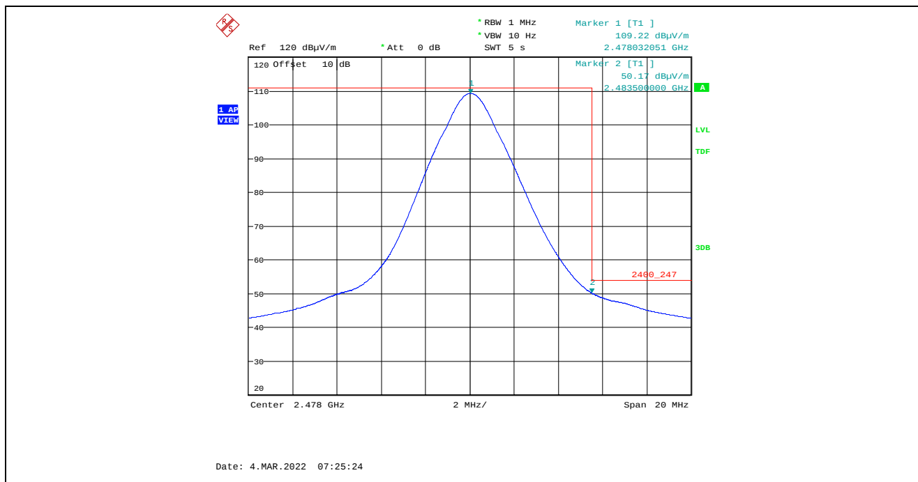
Plot 5.4.4.7.2.6. Band-Edge RF Radiated Emissions at 3 m, Horizontal Polarization, Average High End of Frequency Band, 2478 MHz, 8 dBm Power Setting, 2 Mbps
