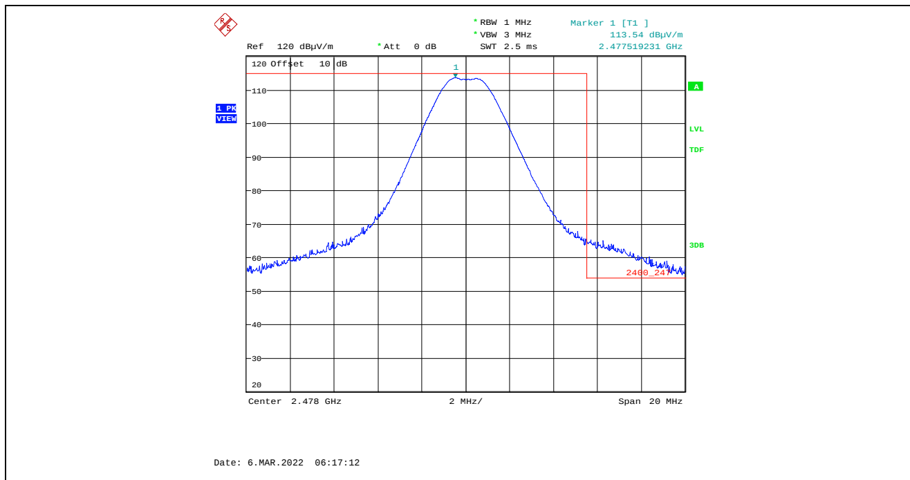
Plot 5.4.4.6.2.5. Band-Edge RF Radiated Emissions at 3 m, Horizontal Polarization, Peak High End of Frequency Band, 2478 MHz, 8 dBm Power Setting, 2 Mbps
