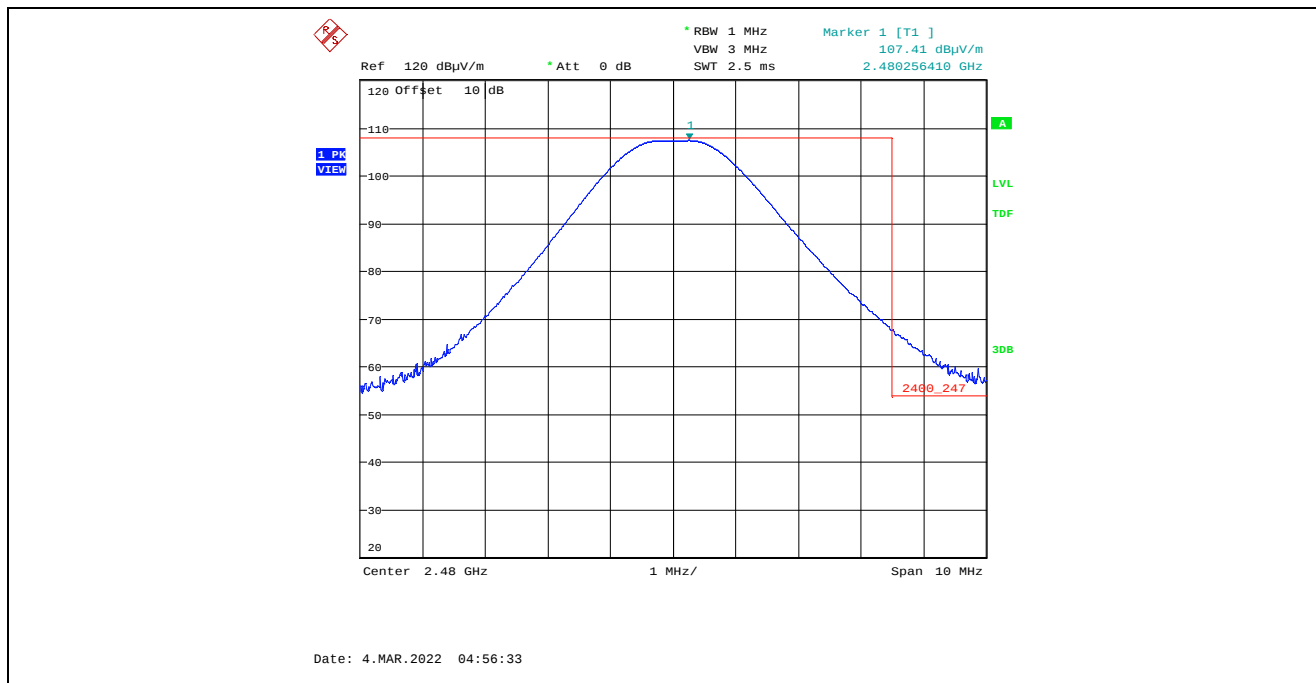
Plot 5.4.4.1.2.5. Band-Edge RF Radiated Emissions at 3 m, Horizontal Polarization, Peak High End of Frequency Band, 2480 MHz, 8 dBm Power Setting, 1 Mbps
