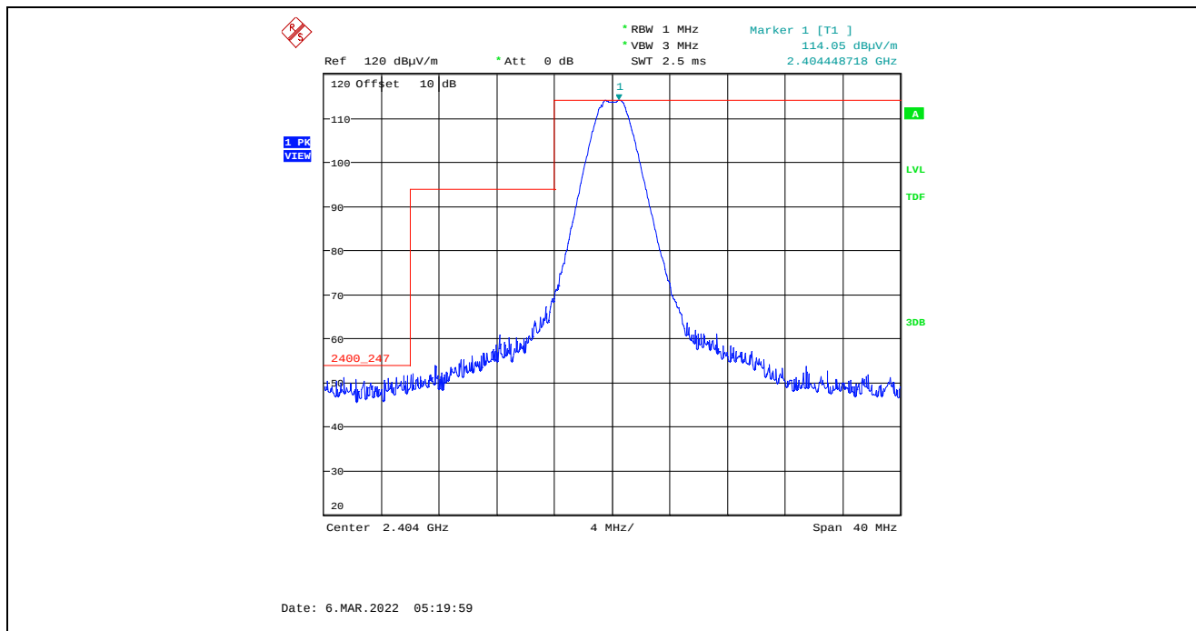
Plot 5.4.4.6.2.3. Band-Edge RF Radiated Emissions at 3 m, Vertical Polarization, Peak Low End of Frequency Band, 2404 MHz, 8 dBm Power Setting, 2 Mbps
