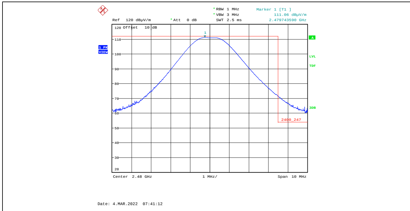
Plot 5.4.4.3.2.5. Band-Edge RF Radiated Emissions at 3 m, Horizontal Polarization, Peak High End of Frequency Band, 2480 MHz, 8 dBm Power Setting, 1 Mbps
