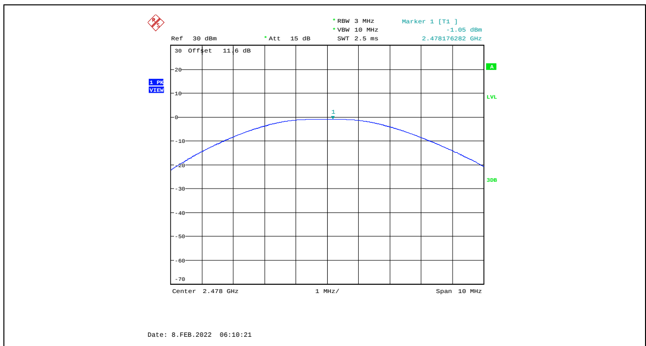
Plot 5.3.4.12. Maximum Peak Conducted Output Power, GFSK Modulation, 2 Mbps, -2 dBm Power Setting, 2478 MHz
