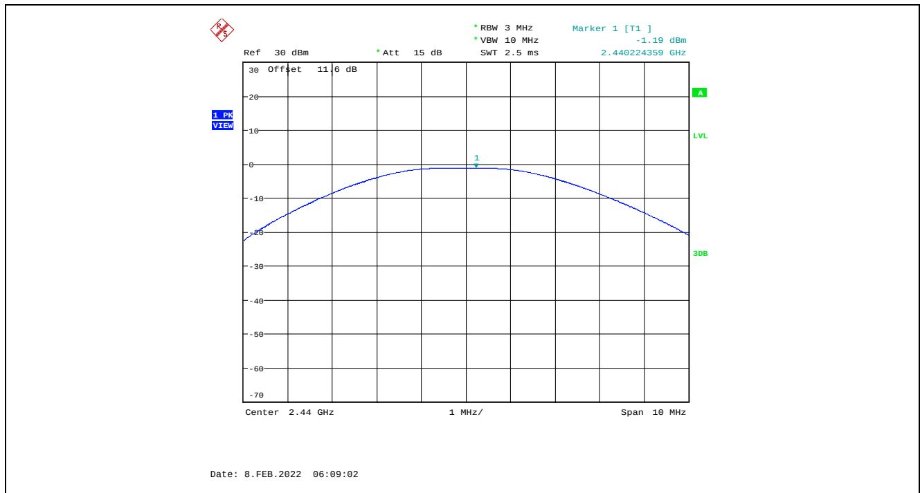
Plot 5.3.4.11. Maximum Peak Conducted Output Power, GFSK Modulation, 2 Mbps, -2 dBm Power Setting, 2440 MHz
