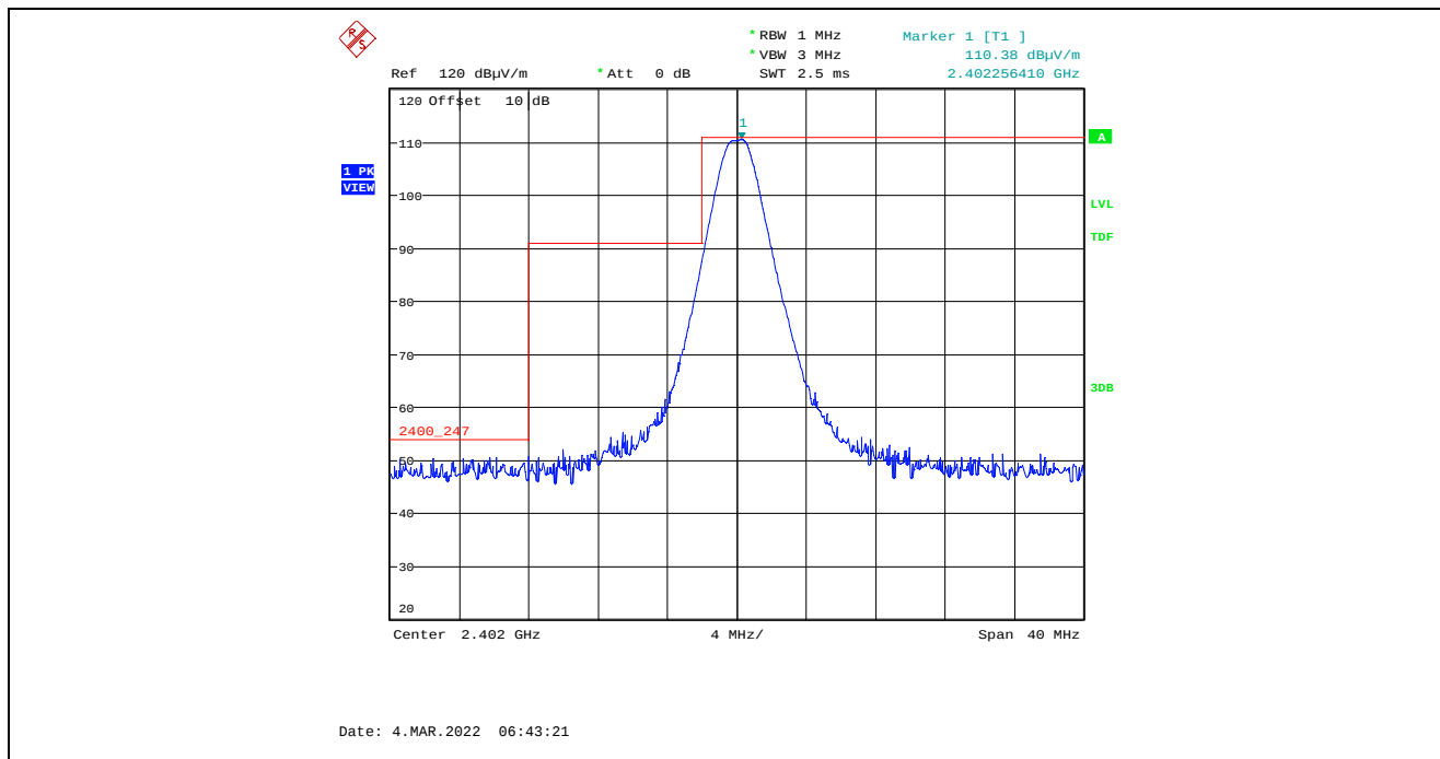
Plot 5.4.4.3.2.3. Band-Edge RF Radiated Emissions at 3 m, Vertical Polarization, Peak Low End of Frequency Band, 2402 MHz, 8 dBm Power Setting, 1 Mbps
