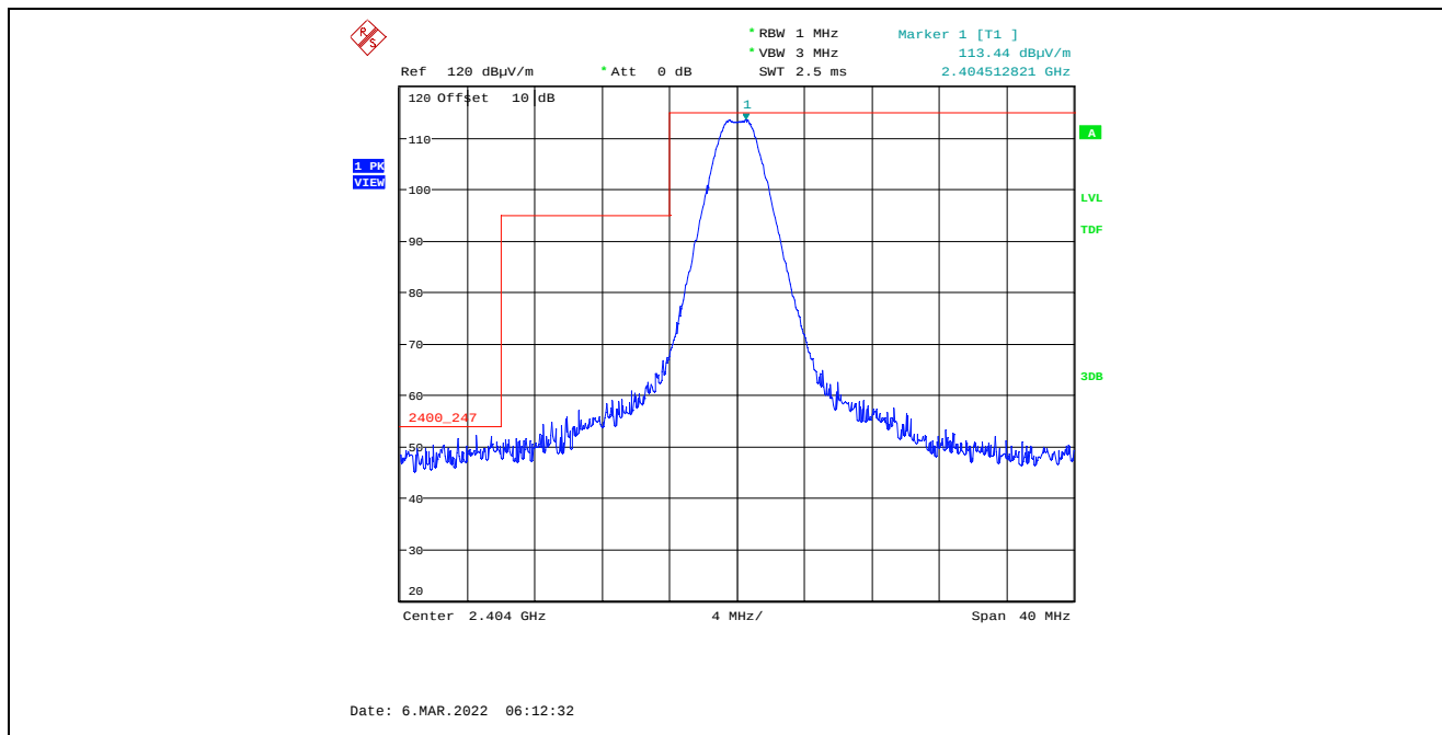
Plot 5.4.4.6.2.1. Band-Edge RF Radiated Emissions at 3 m, Horizontal Polarization, Peak Low End of Frequency Band, 2404 MHz, 8 dBm Power Setting, 2 Mbps
