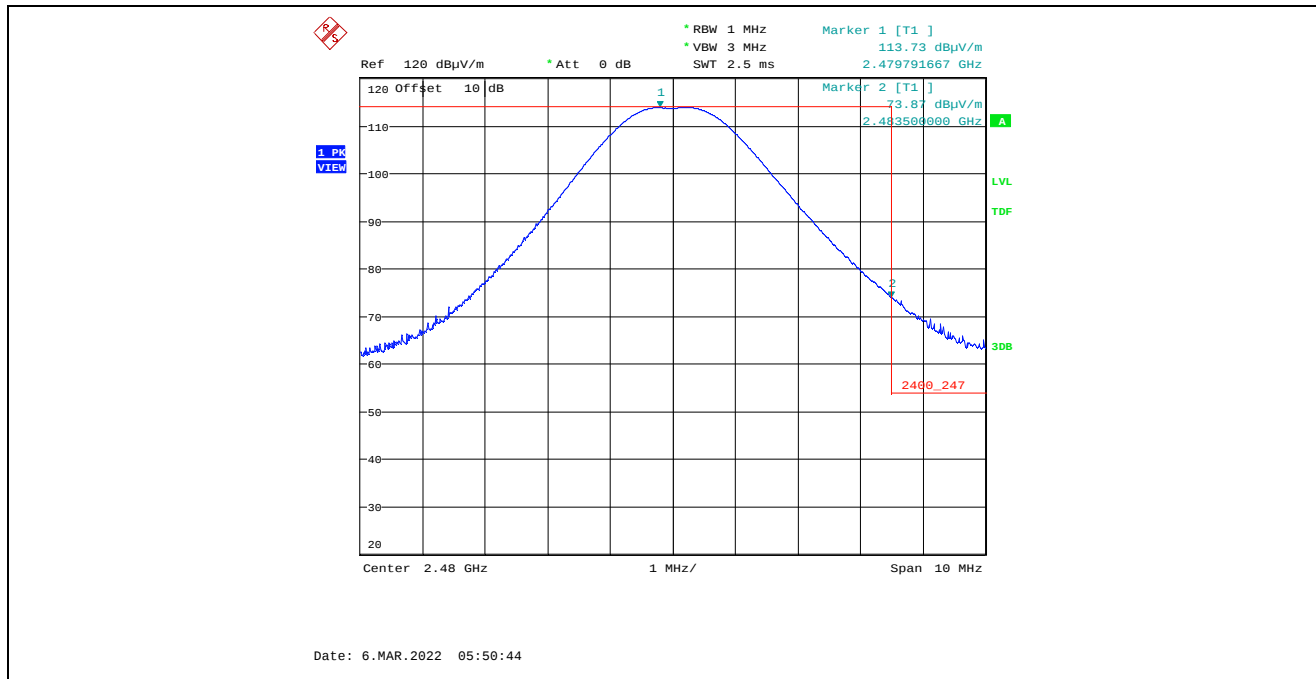
Plot 5.4.4.2.2.5. Band-Edge RF Radiated Emissions at 3 m, Horizontal Polarization, Peak High End of Frequency Band, 2480 MHz, 8 dBm Power Setting, 1 Mbps
