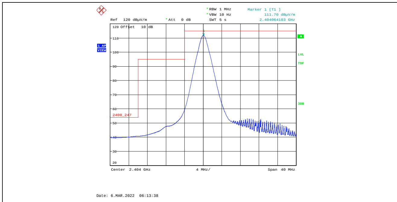
Plot 5.4.4.6.2.2. Band-Edge RF Radiated Emissions at 3 m, Horizontal Polarization, Average Low End of Frequency Band, 2404 MHz, 8 dBm Power Setting, 2 Mbps
