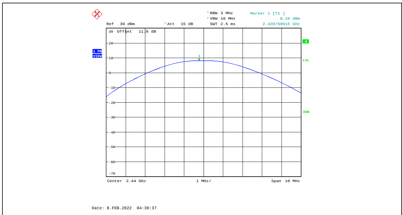
Plot 5.3.4.2. Maximum Peak Conducted Output Power, GFSK Modulation, 1 Mbps, 8 dBm Power Setting, 2440 MHz
