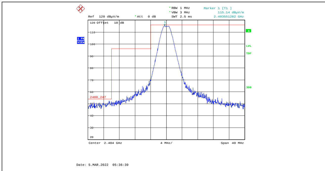
Plot 5.4.4.8.2.3. Band-Edge RF Radiated Emissions at 3 m, Vertical Polarization, Peak Low End of Frequency Band, 2404 MHz, 8 dBm Power Setting, 2 Mbps
