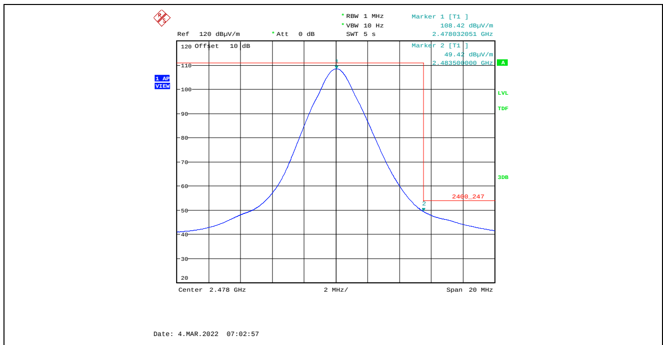
Plot 5.4.4.7.2.8. Band-Edge RF Radiated Emissions at 3 m, Vertical Polarization, Average High End of Frequency Band, 2478 MHz, 8 dBm Power Setting, 2 Mbps
