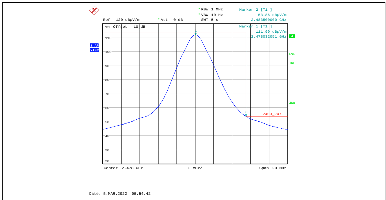
Plot 5.4.4.8.2.6. Band-Edge RF Radiated Emissions at 3 m, Horizontal Polarization, Average High End of Frequency Band, 2478 MHz, 8 dBm Power Setting, 2 Mbps
