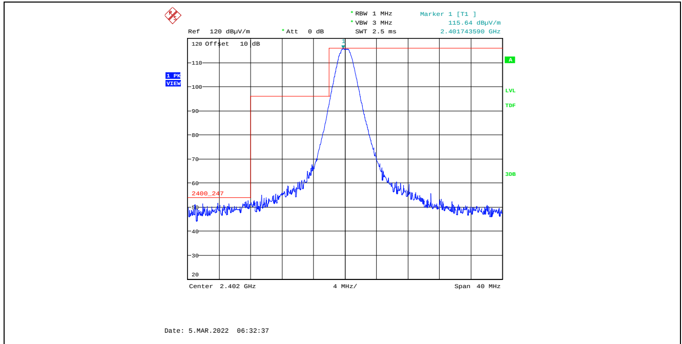
Plot 5.4.4.4.2.1. Band-Edge RF Radiated Emissions at 3 m, Horizontal Polarization, Peak Low End of Frequency Band, 2402 MHz, 8 dBm Power Setting, 1 Mbps
