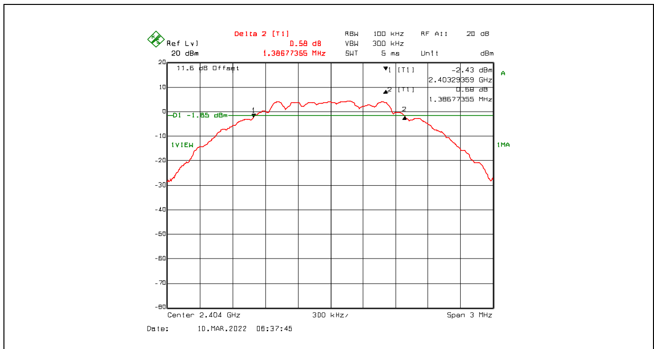
Plot 5.2.4.4. 6 dB Bandwidth, GFSK Modulation, 8 dBm Power Setting, 2 Mbps, 2404 MHz
