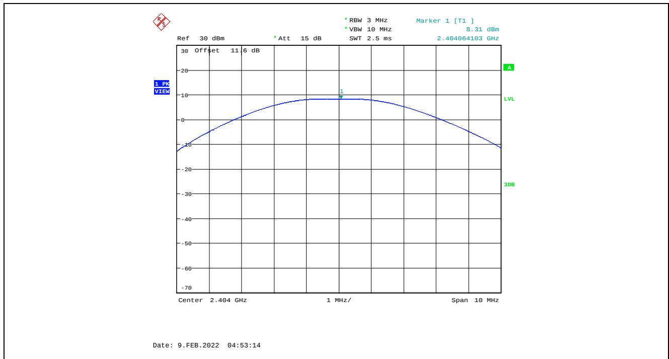
Plot 5.3.4.7. Maximum Peak Conducted Output Power, GFSK Modulation, 2 Mbps, 8 dBm Power Setting, 2404 MHz
