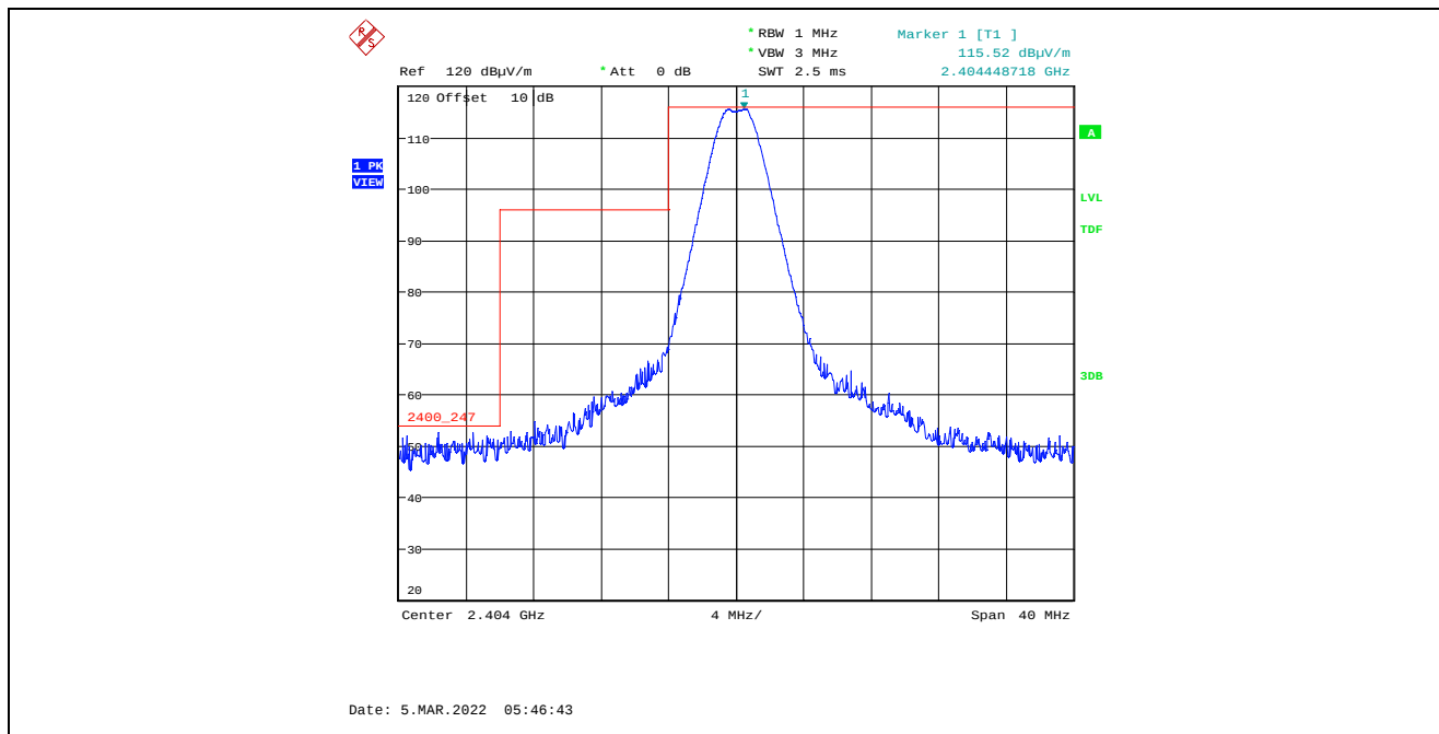
Plot 5.4.4.8.2.1. Band-Edge RF Radiated Emissions at 3 m, Horizontal Polarization, Peak Low End of Frequency Band, 2404 MHz, 8 dBm Power Setting, 2 Mbps
