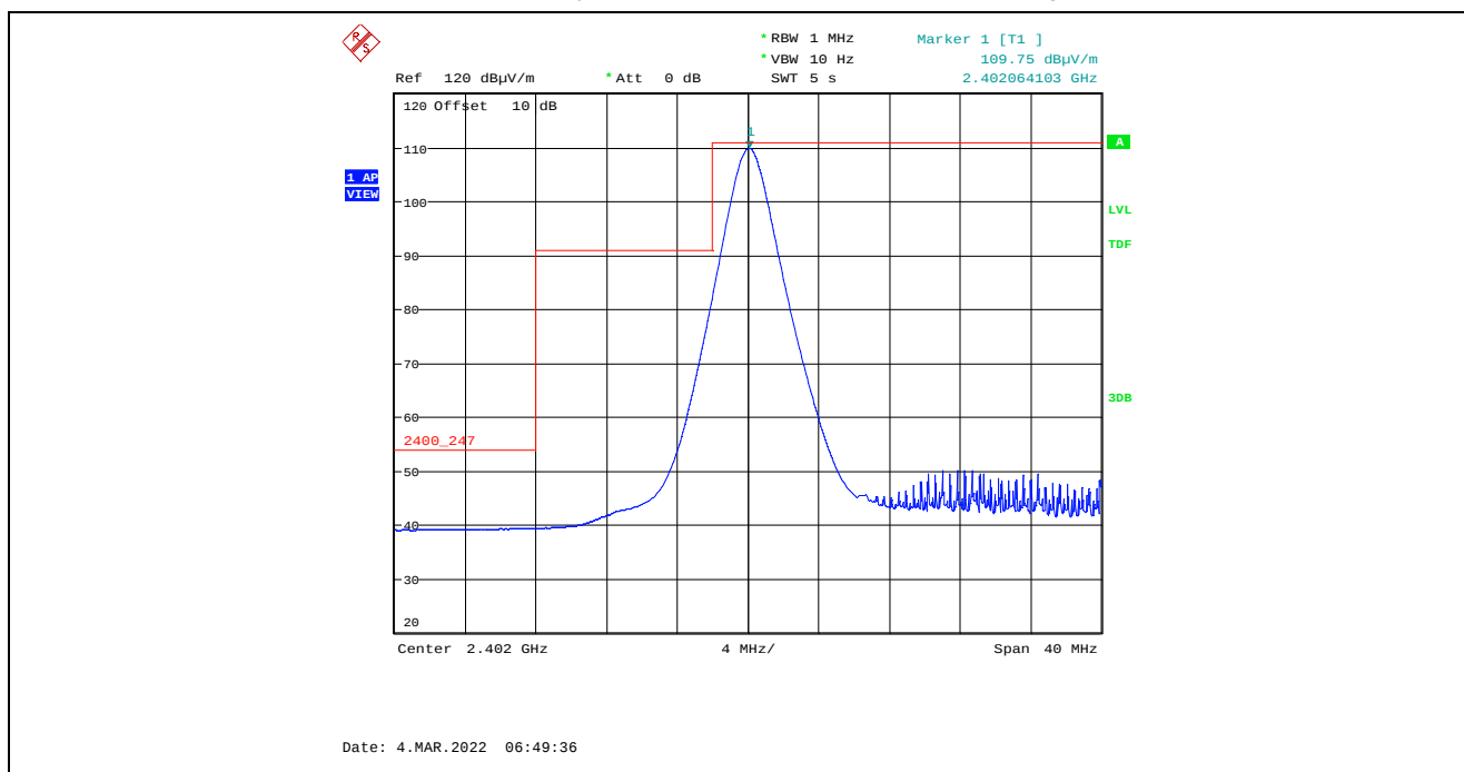
Plot 5.4.4.3.2.4. Band-Edge RF Radiated Emissions at 3 m, Vertical Polarization, Average Low End of Frequency Band, 2402 MHz, 8 dBm Power Setting, 1 Mbps
