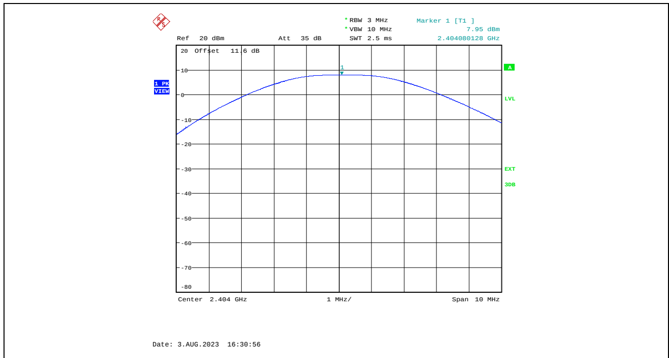
Plot 5.1.4.7. Maximum Peak Conducted Output Power, GFSK Modulation, 2 Mbps, 8 dBm Power Setting, 2404 MHz
