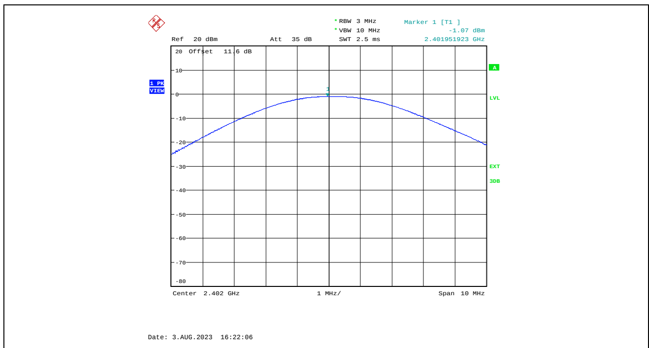
Plot 5.1.4.4. Maximum Peak Conducted Output Power, GFSK Modulation, 1 Mbps, -2 dBm Power Setting, 2402 MHz
