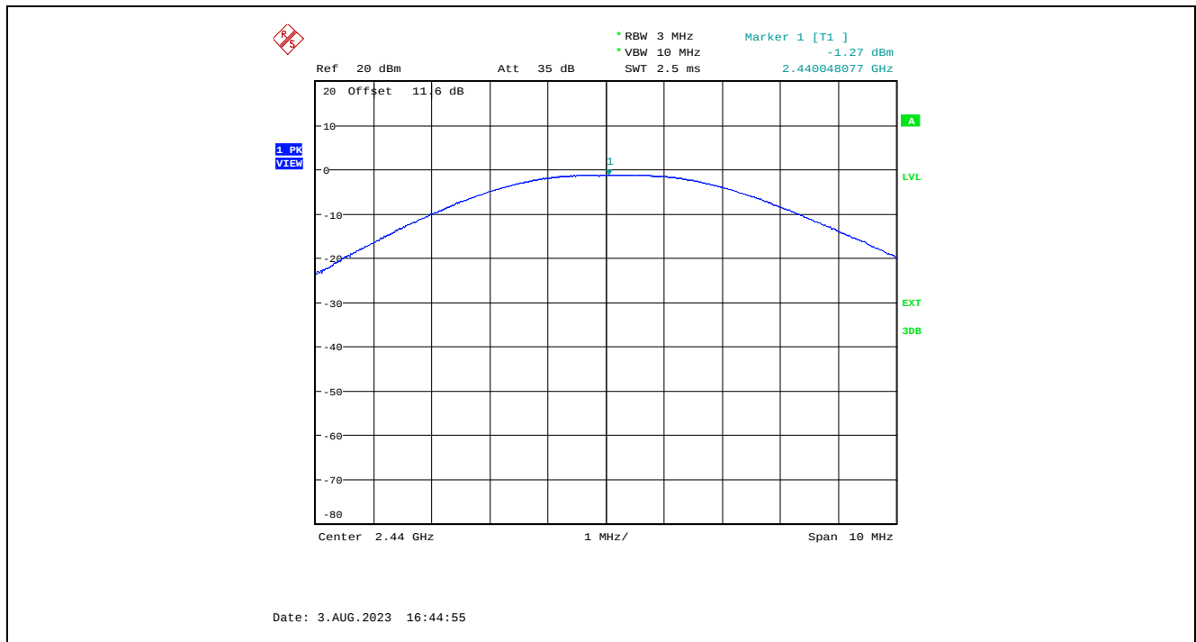
Plot 5.1.4.11. Maximum Peak Conducted Output Power, GFSK Modulation, 2 Mbps, -2 dBm Power Setting, 2440 MHz
