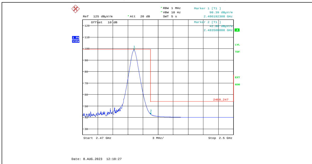
Plot 5.2.4.1.2.6. Band-Edge RF Radiated Emissions at 3 m, Vertical Polarization, Average High End of Frequency Band, 2480 MHz, 8 dBm Power Setting, 1 Mbps
