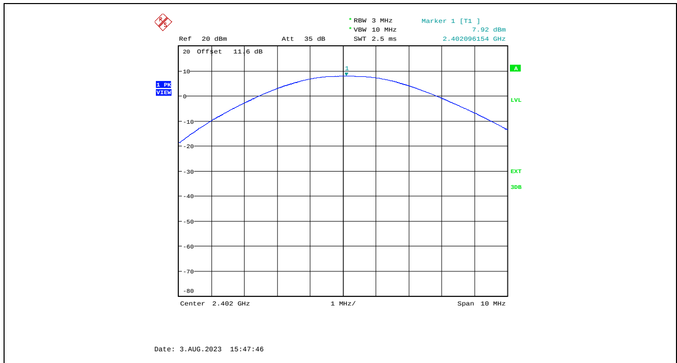
Plot 5.1.4.1. Maximum Peak Conducted Output Power, GFSK Modulation, 1 Mbps, 8 dBm Power Setting, 2402 MHz
