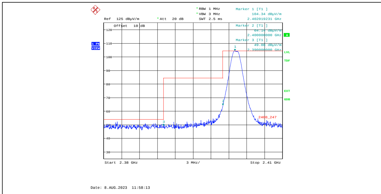
Plot 5.2.4.1.2.1. Band-Edge RF Radiated Emissions at 3 m, Vertical Polarization, Peak Low End of Frequency Band, 2402 MHz, 8 dBm Power Setting, 1 Mbps
