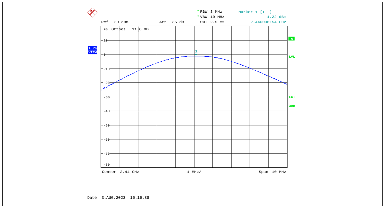
Plot 5.1.4.5. Maximum Peak Conducted Output Power, GFSK Modulation, 1 Mbps, -2 dBm Power Setting, 2440 MHz
