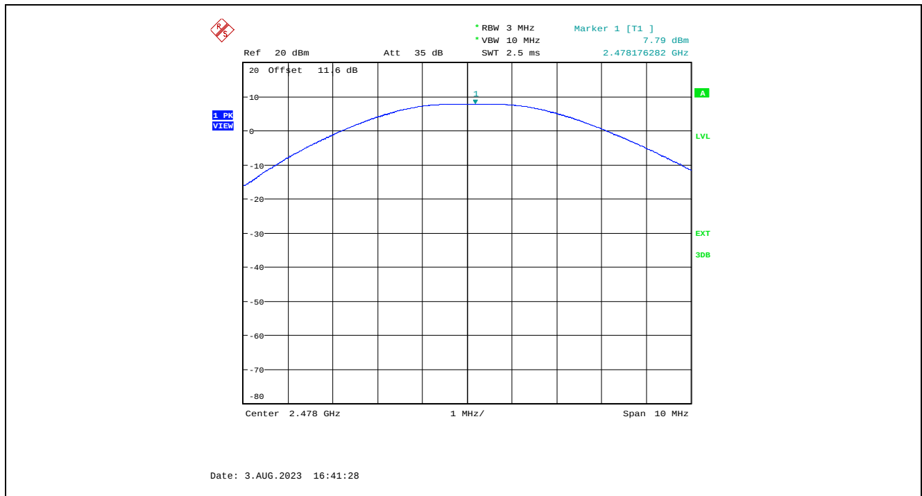
Plot 5.1.4.9. Maximum Peak Conducted Output Power, GFSK Modulation, 2 Mbps, 8 dBm Power Setting, 2478 MHz
