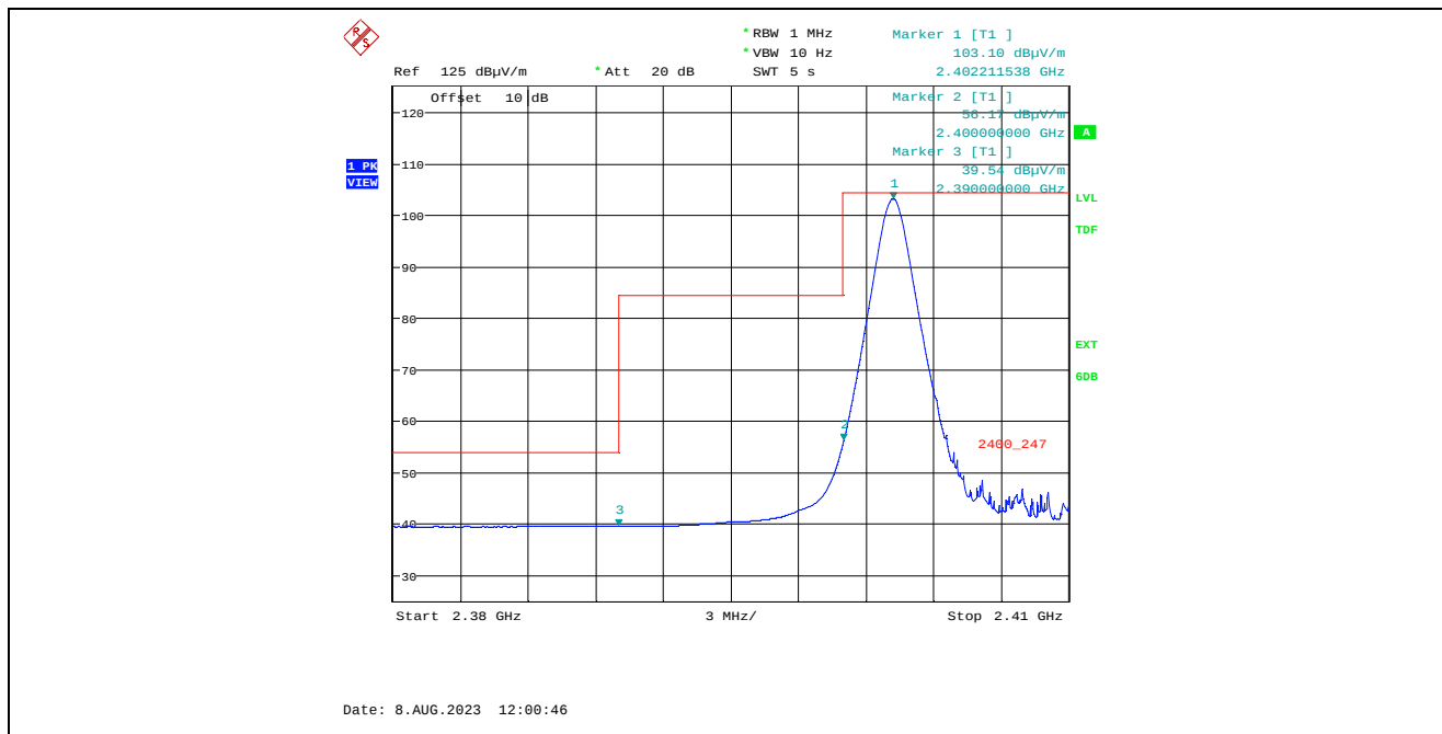
Plot 5.2.4.1.2.2. Band-Edge RF Radiated Emissions at 3 m, Vertical Polarization, Average Low End of Frequency Band, 2402 MHz, 8 dBm Power Setting, 1 Mbps
