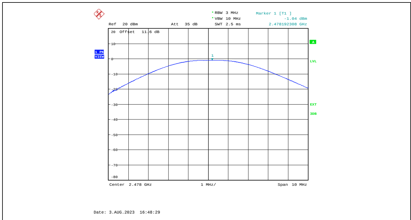
Plot 5.1.4.12. Maximum Peak Conducted Output Power, GFSK Modulation, 2 Mbps, -2 dBm Power Setting, 2478 MHz
