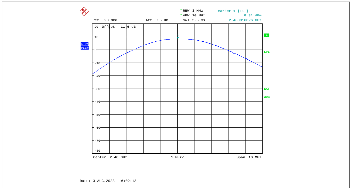
Plot 5.1.4.3. Maximum Peak Conducted Output Power, GFSK Modulation, 1 Mbps, 8 dBm Power Setting, 2480 MHz
