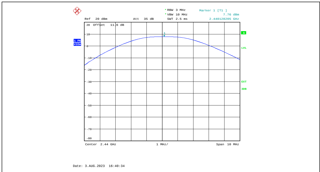
Plot 5.1.4.8. Maximum Peak Conducted Output Power, GFSK Modulation, 2 Mbps, 8 dBm Power Setting, 2440 MHz
