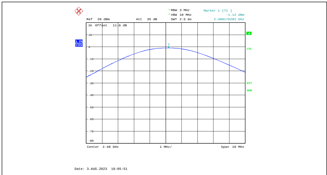
Plot 5.1.4.6. Maximum Peak Conducted Output Power, GFSK Modulation, 1 Mbps, -2 dBm Power Setting, 2480 MHz
