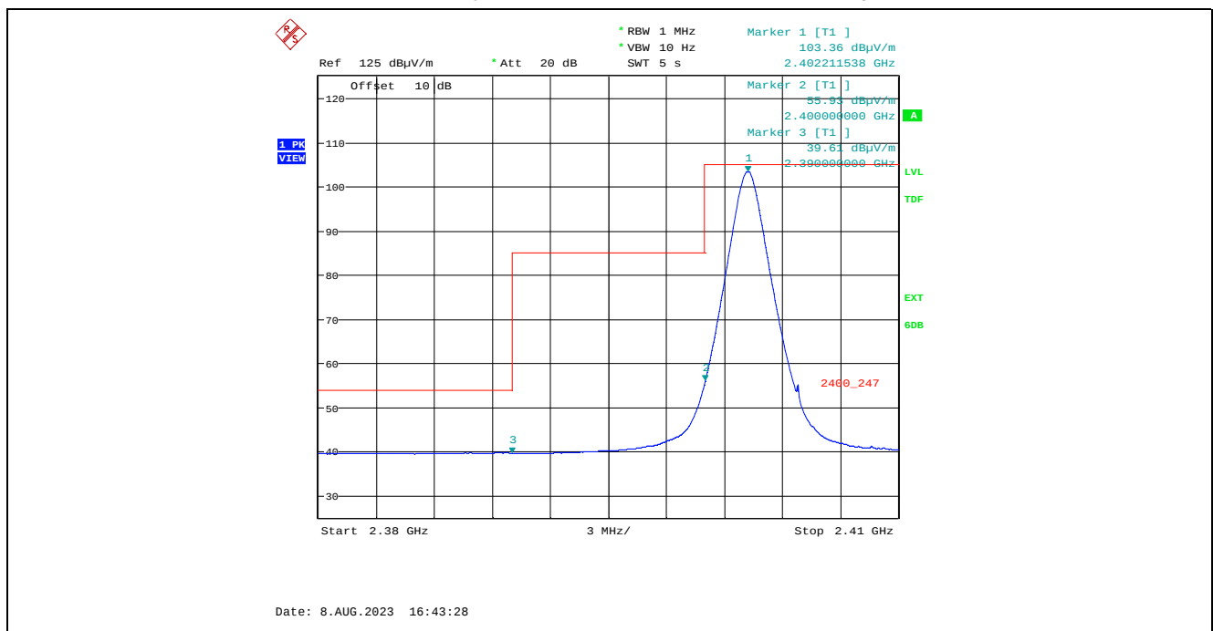
Plot 5.2.4.1.2.4. Band-Edge RF Radiated Emissions at 3 m, Horizontal Polarization, Average Low End of Frequency Band, 2402 MHz, 8 dBm Power Setting, 1 Mbps
