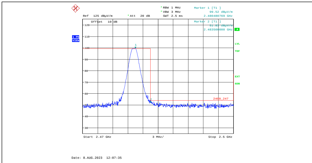
Plot 5.2.4.1.2.5. Band-Edge RF Radiated Emissions at 3 m, Vertical Polarization, Peak High End of Frequency Band, 2480 MHz, 8 dBm Power Setting, 1 Mbps
