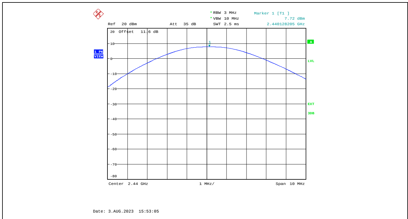
Plot 5.1.4.2. Maximum Peak Conducted Output Power, GFSK Modulation, 1 Mbps, 8 dBm Power Setting, 2440 MHz
