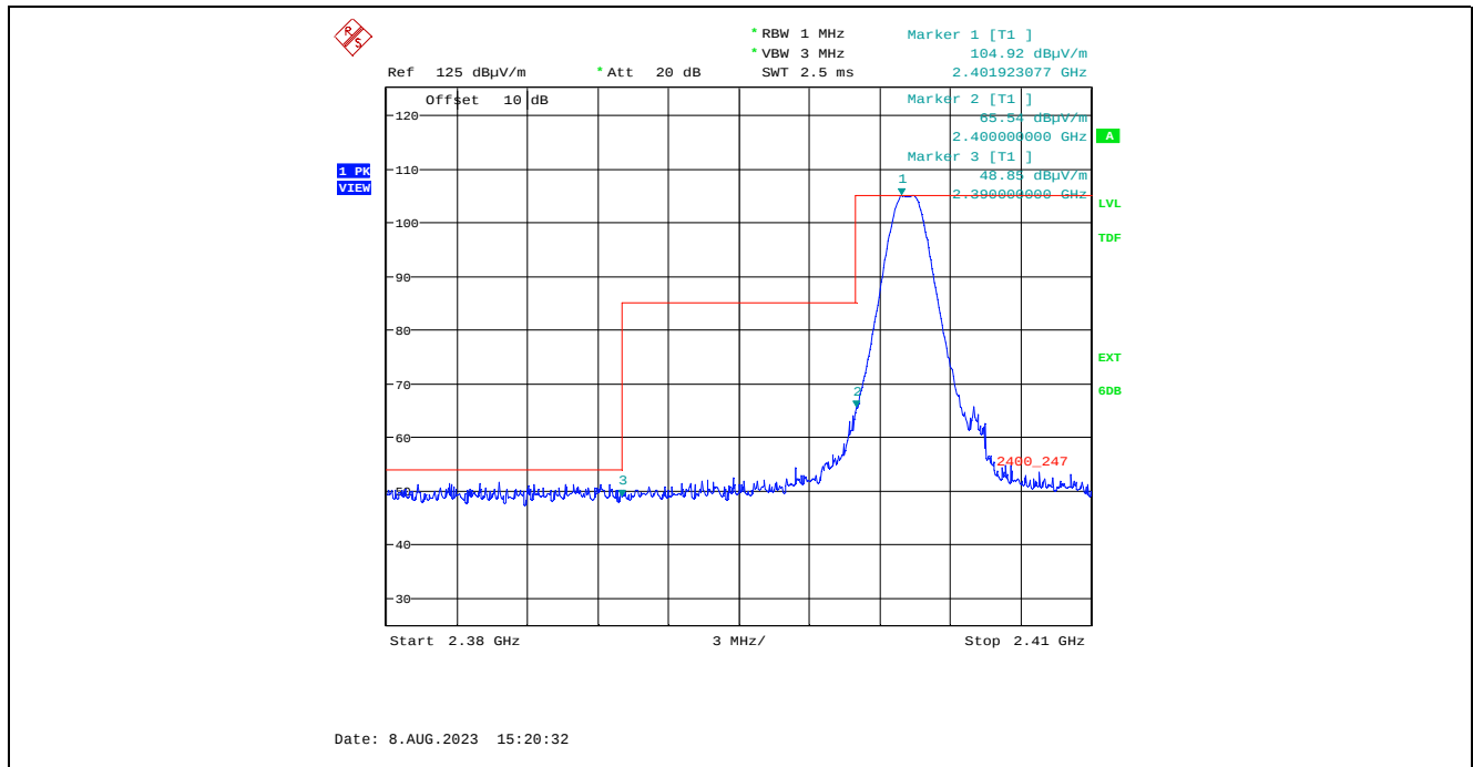
Plot 5.2.4.1.2.3. Band-Edge RF Radiated Emissions at 3 m, Horizontal Polarization, Peak Low End of Frequency Band, 2402 MHz, 8 dBm Power Setting, 1 Mbps
