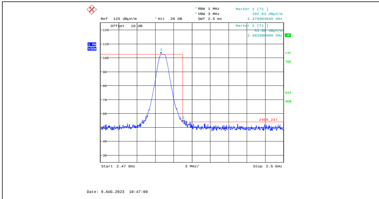
Plot 5.2.4.1.2.7. Band-Edge RF Radiated Emissions at 3 m, Horizontal Polarization, Peak High End of Frequency Band, 2480 MHz, 8 dBm Power Setting, 1 Mbps
