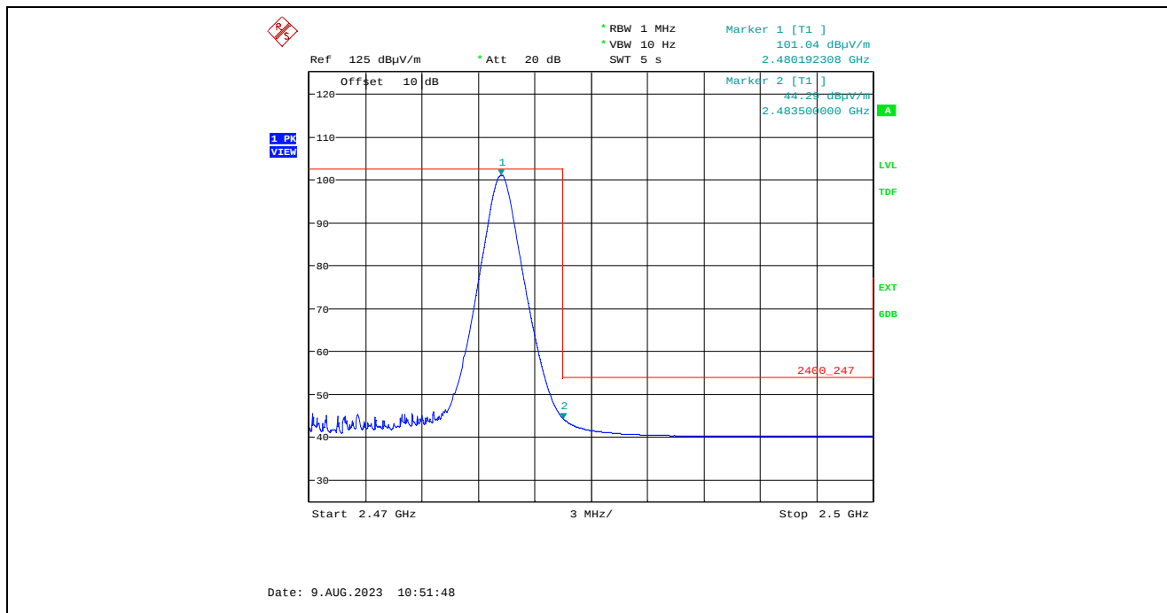
Plot 5.2.4.1.2.8. Band-Edge RF Radiated Emissions at 3 m, Horizontal Polarization, Average High End of Frequency Band, 2480 MHz, 8 dBm Power Setting, 1 Mbps
