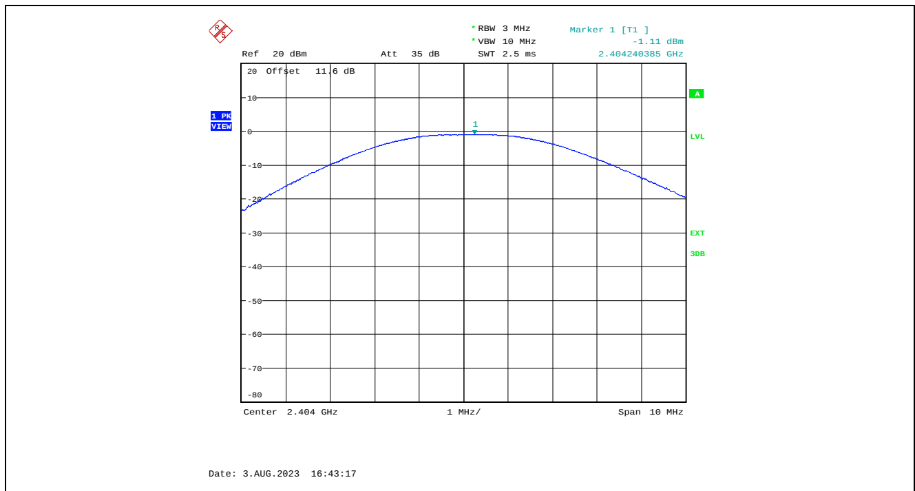
Plot 5.1.4.10. Maximum Peak Conducted Output Power, GFSK Modulation, 2 Mbps, -2 dBm Power Setting, 2404 MHz
