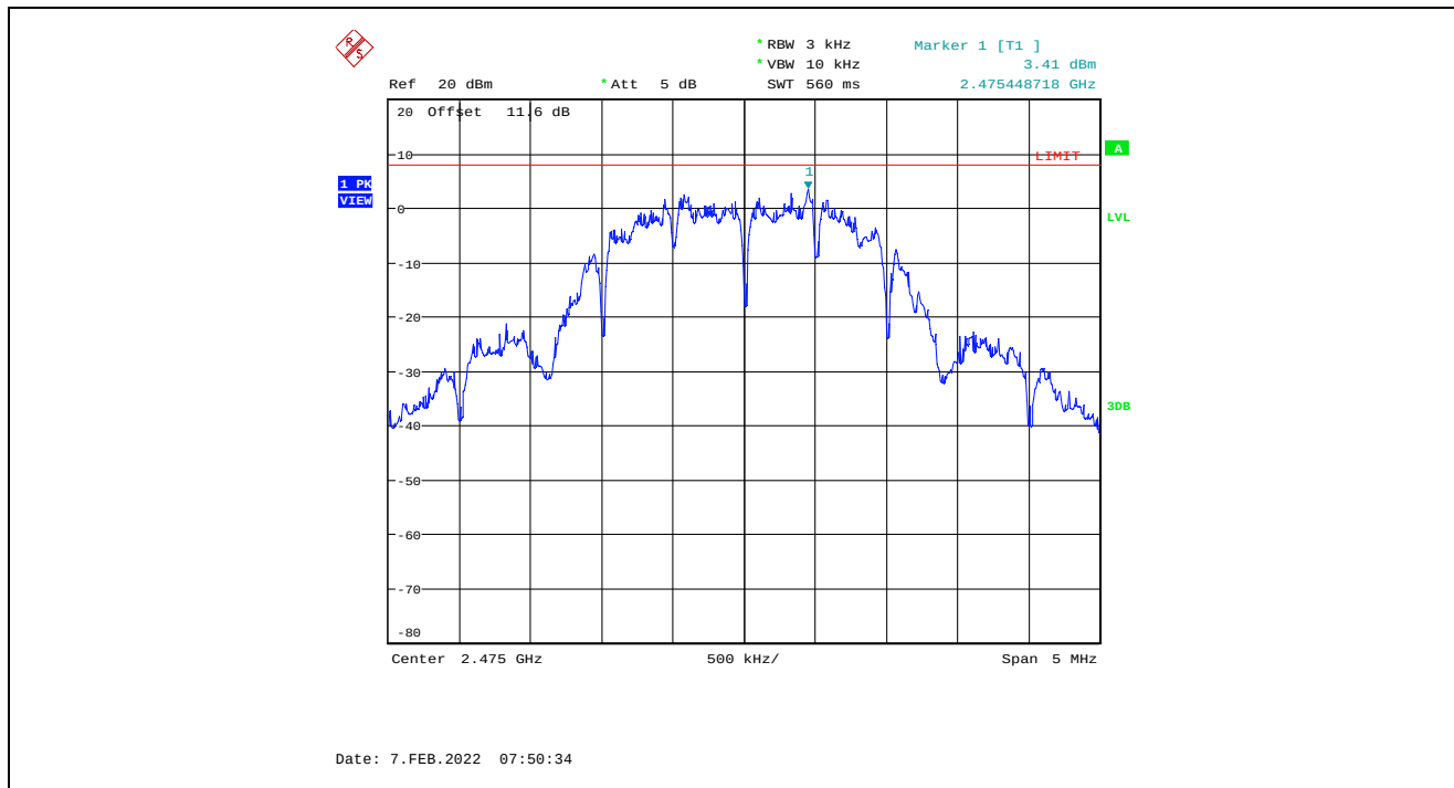
Plot 5.5.4.3. Power Spectral Density, QPSK Modulation, 20 dBm Power Setting, 2475 MHz
