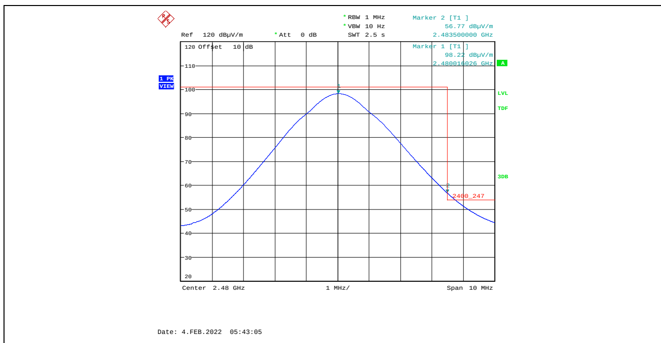
Plot 5.4.4.2.12. Band-Edge RF Radiated Emissions at 3 m, Vertical Polarization, Average High End of Frequency Band, 2480 MHz, 3 dBm Power Setting Marker 2: 56.77 dBμV/m – 3.61 dB = 53.16 dBμV/m (Limit 54 dBμV/m)
