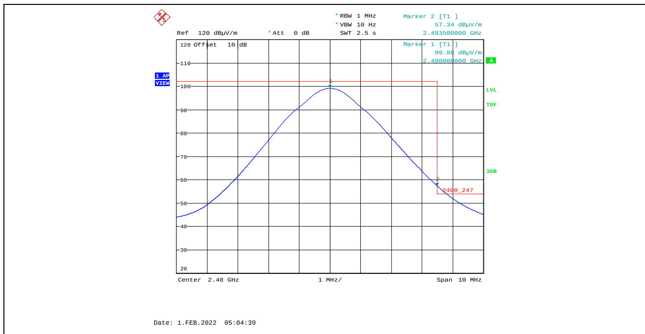
Plot 5.4.4.2.10. Band-Edge RF Radiated Emissions at 3 m, Horizontal Polarization, Average High End of Frequency Band, 2480 MHz, 3 dBm Power Setting Marker 2: 57.34 dBμV/m – 3.61 dB Duty Cycle Factor = 53.73 dBμV/m (Limit 54 dBμV/m)
