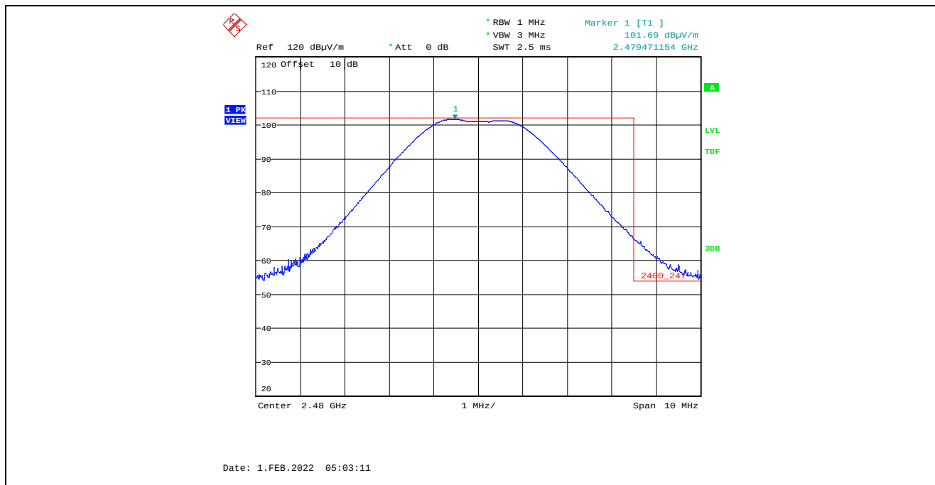
Plot 5.4.4.2.9. Band-Edge RF Radiated Emissions at 3 m, Horizontal Polarization, Peak High End of Frequency Band, 2480 MHz, 3 dBm Power Setting
