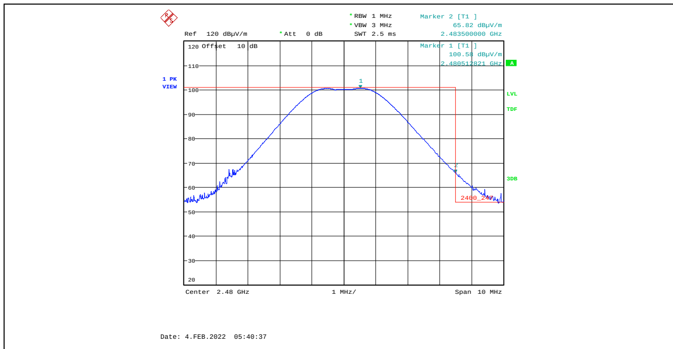
Plot 5.4.4.2.11. Band-Edge RF Radiated Emissions at 3 m, Vertical Polarization, Peak High End of Frequency Band, 2480 MHz, 3 dBm Power Setting
