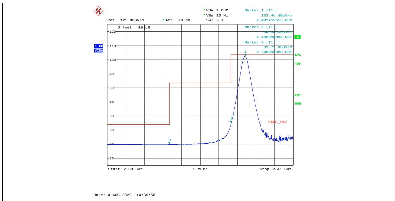
Plot 5.2.4.1.2.2. Band-Edge RF Radiated Emissions at 3 m, Vertical Polarization, Average Low End of Frequency Band, 2402 MHz, 8 dBm Power Setting, 1 Mbps
