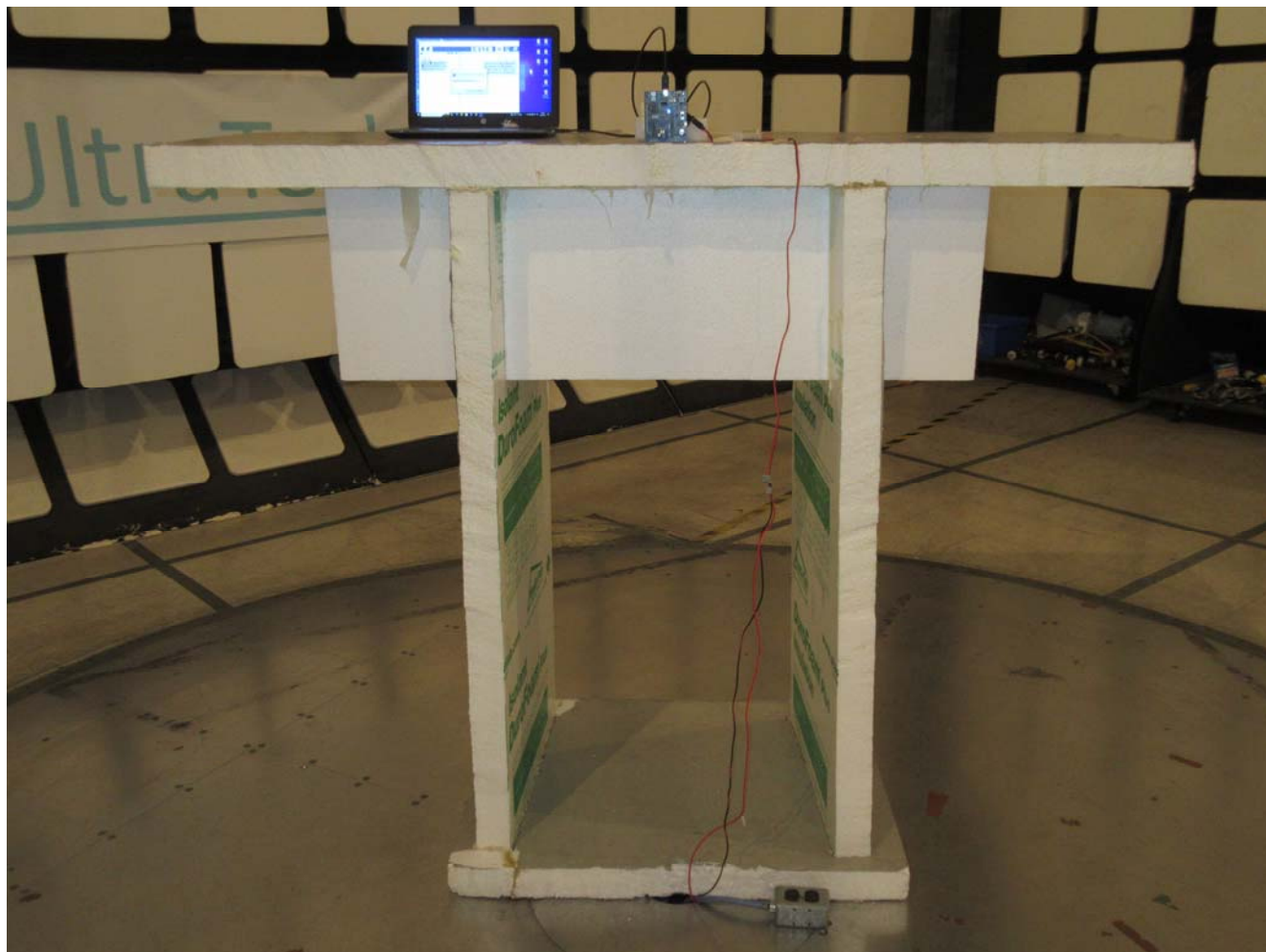
Radiated Emissions at 3 m EUT with -0.5 dBi Embedded F-Style Antenna, Orthogonal Position 3
