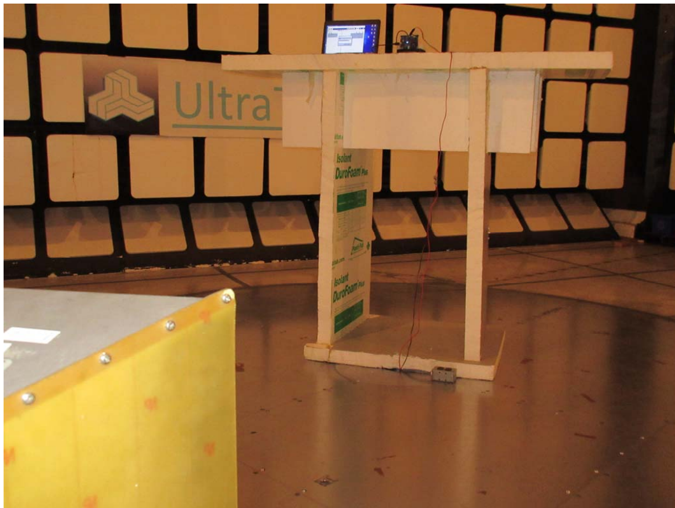
Radiated Emissions at 3 m EUT with -0.5 dBi Embedded F-Style Antenna, Orthogonal Position 2
