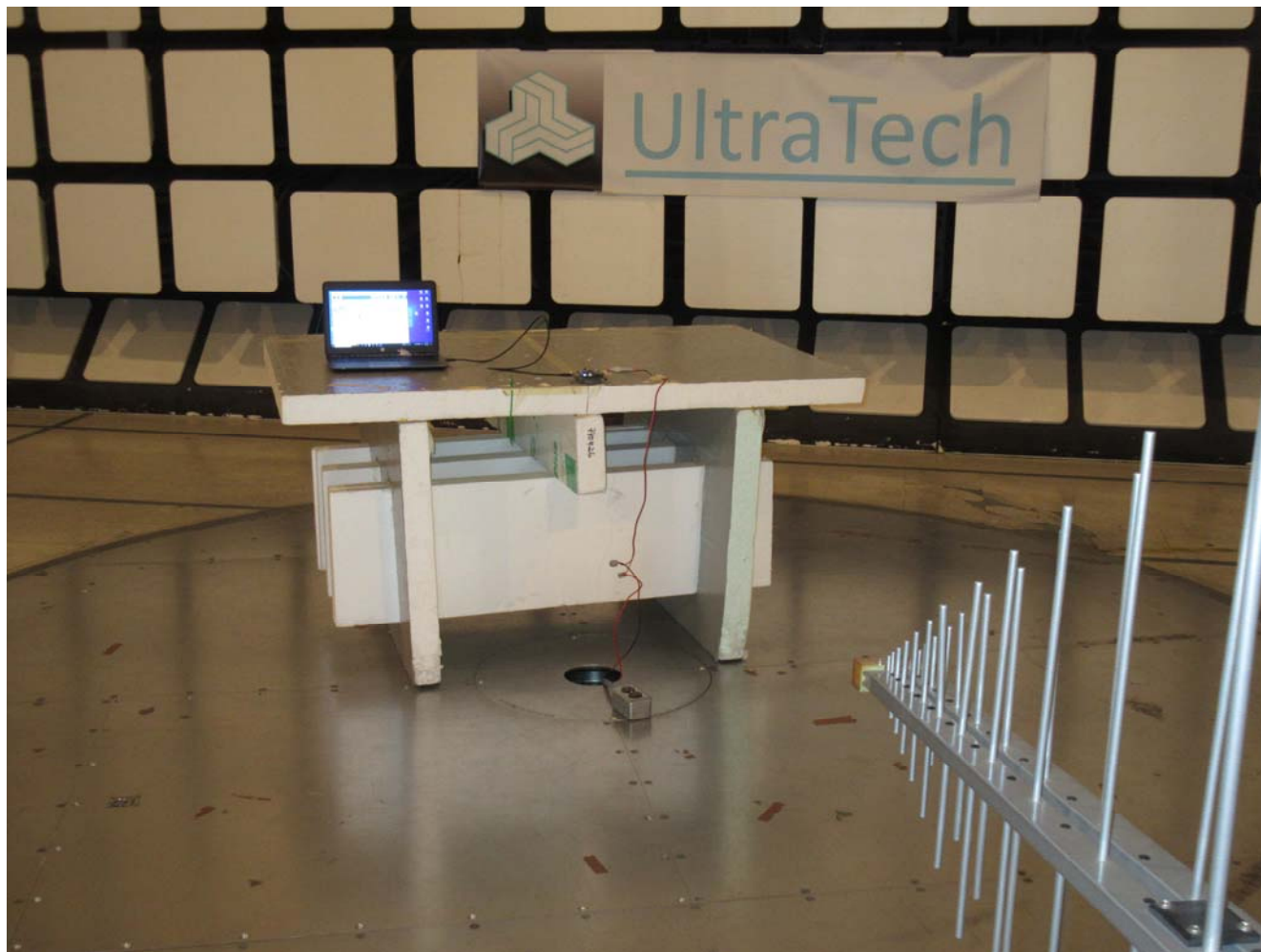
Radiated Emissions at 3 m EUT with -0.5 dBi Embedded F-Style Antenna, Orthogonal Position 1
