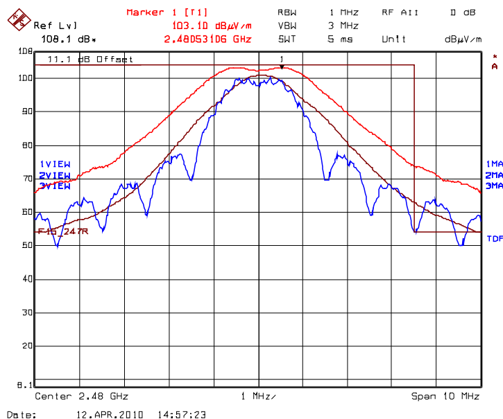
Plot 5.9.4.1.5. Band-Edge RF Radiated Emissions @ 3 m High End of Frequency Band, 2480 MHz, Rx Antenna Orientation: Horizontal
