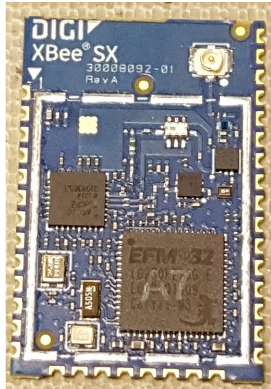
Internal
