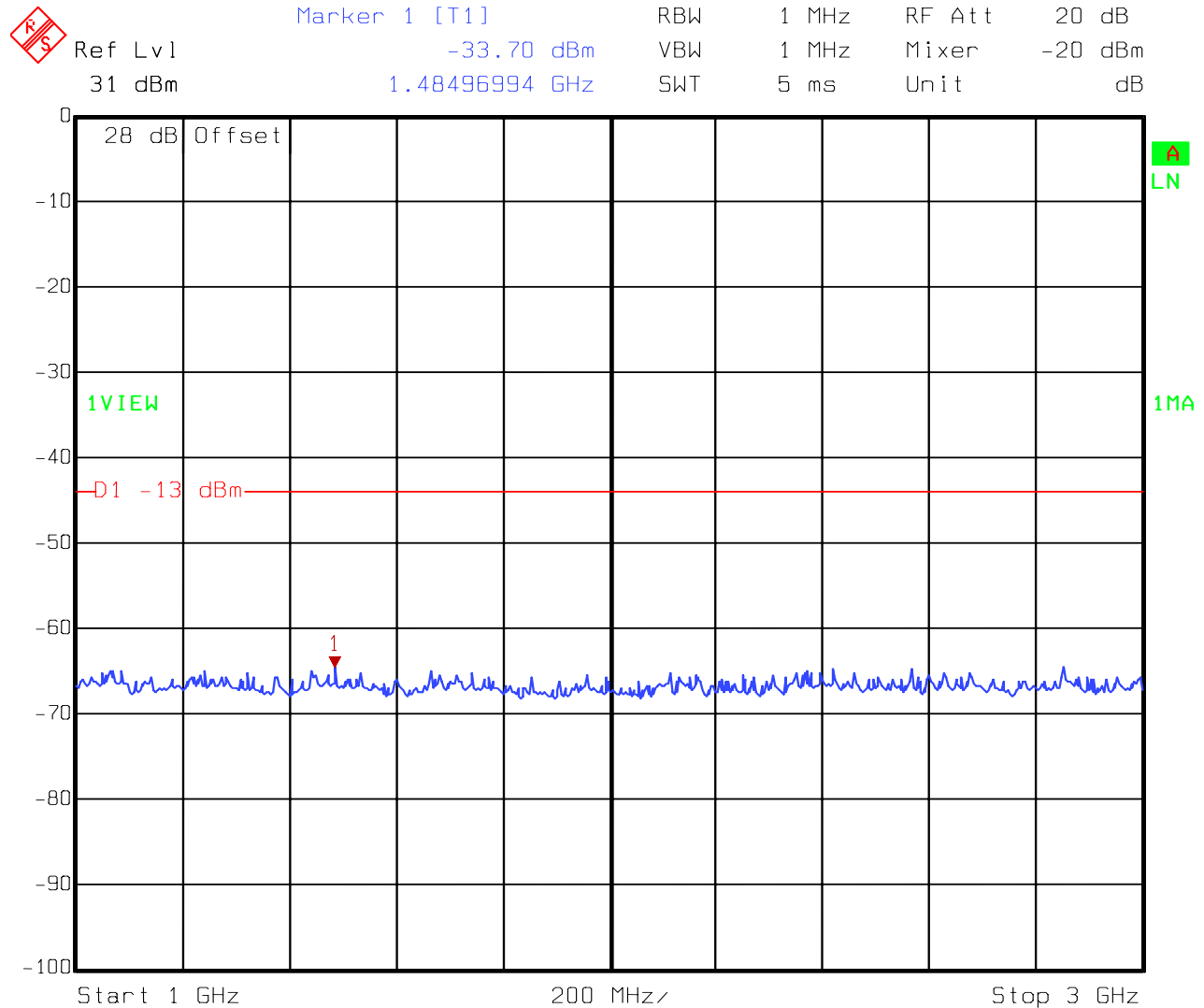
Figure 9 Antenna Conducted Spurious - High Channel – 1 GHz – 3 GHz
