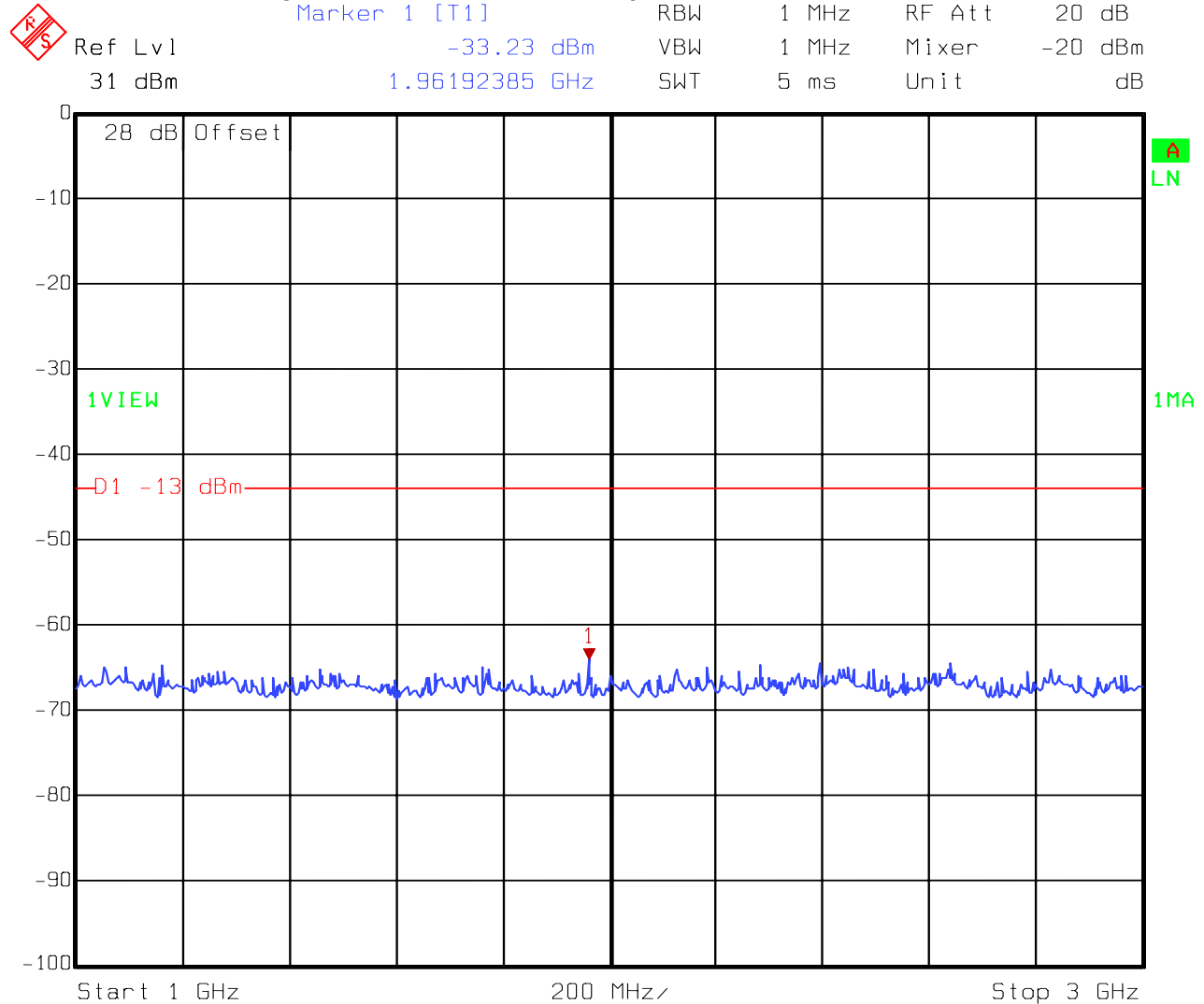
Figure 5 Antenna Conducted Spurious - Low Channel - 1 GHz - 3 GHz
