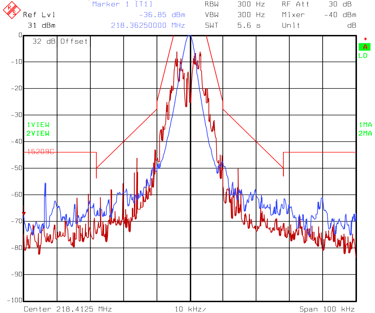
Figure 2 Occupied Bandwidth – Mid Channel
