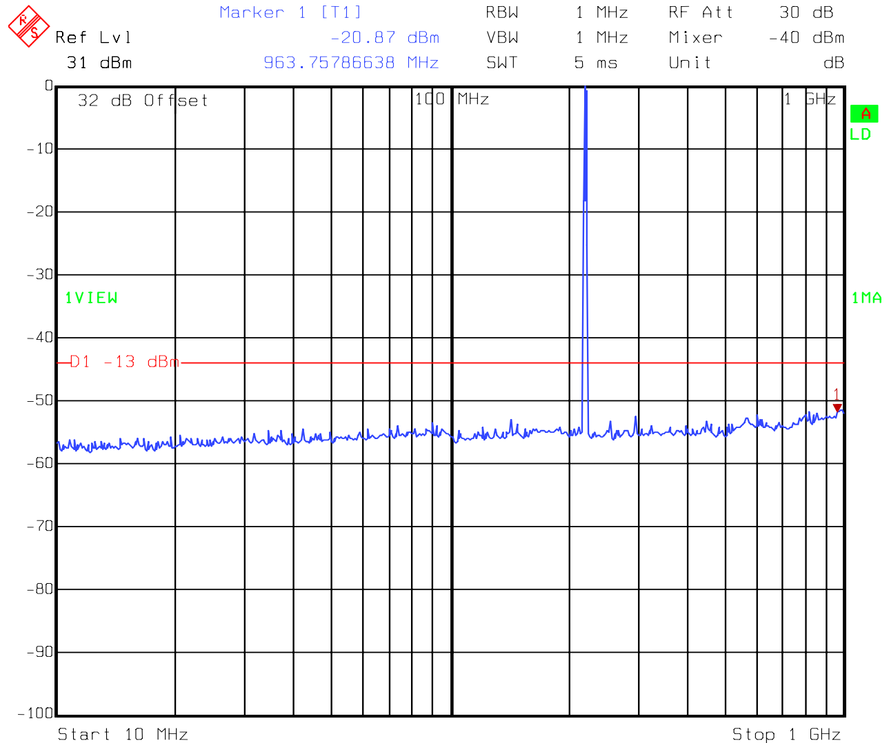
Figure 8 Antenna Conducted Spurious - High Channel – 10 MHz – 1 GHz
