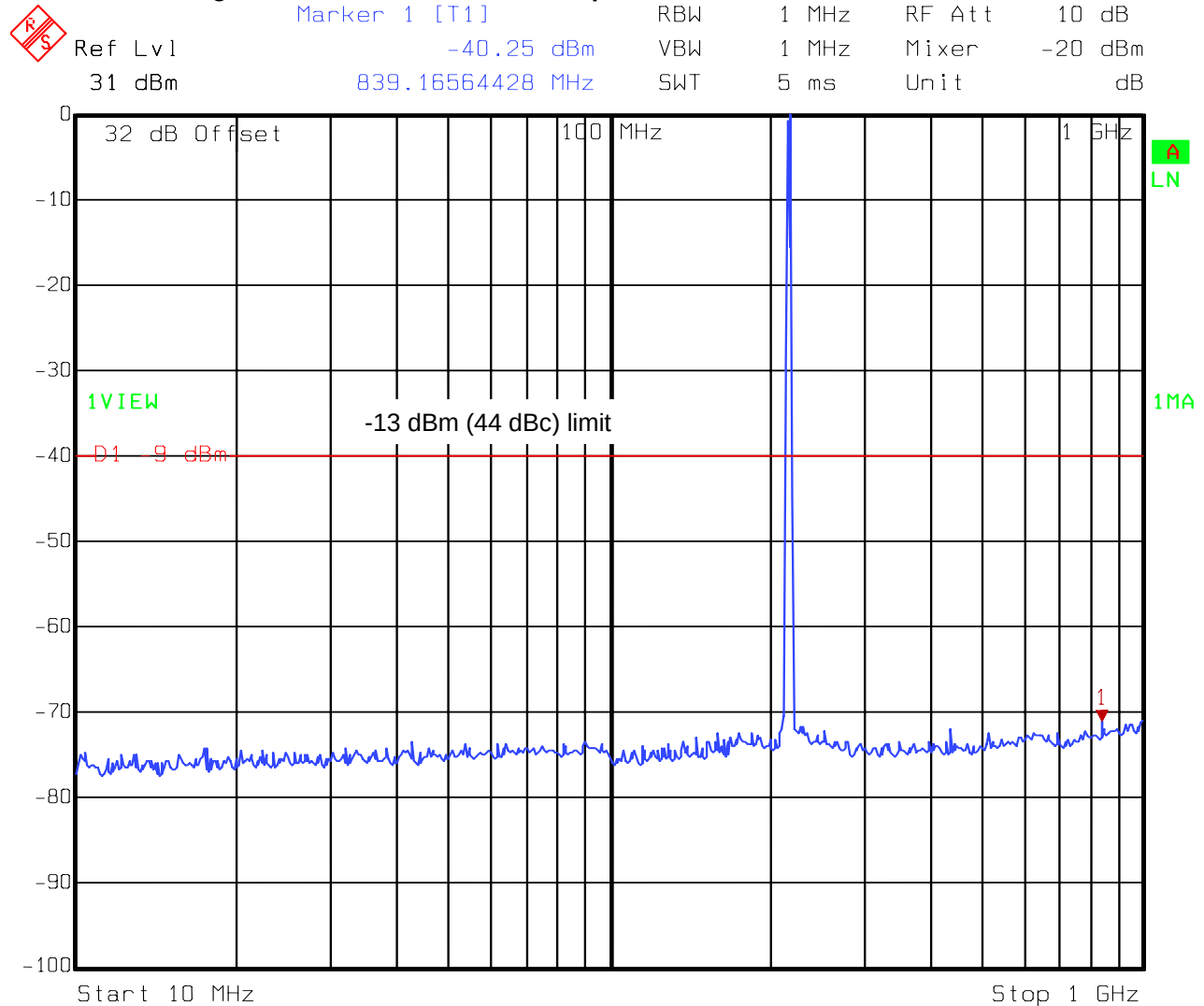
Figure 6 Antenna Conducted Spurious - Mid Channel - 10 MHz - 1 GHz
