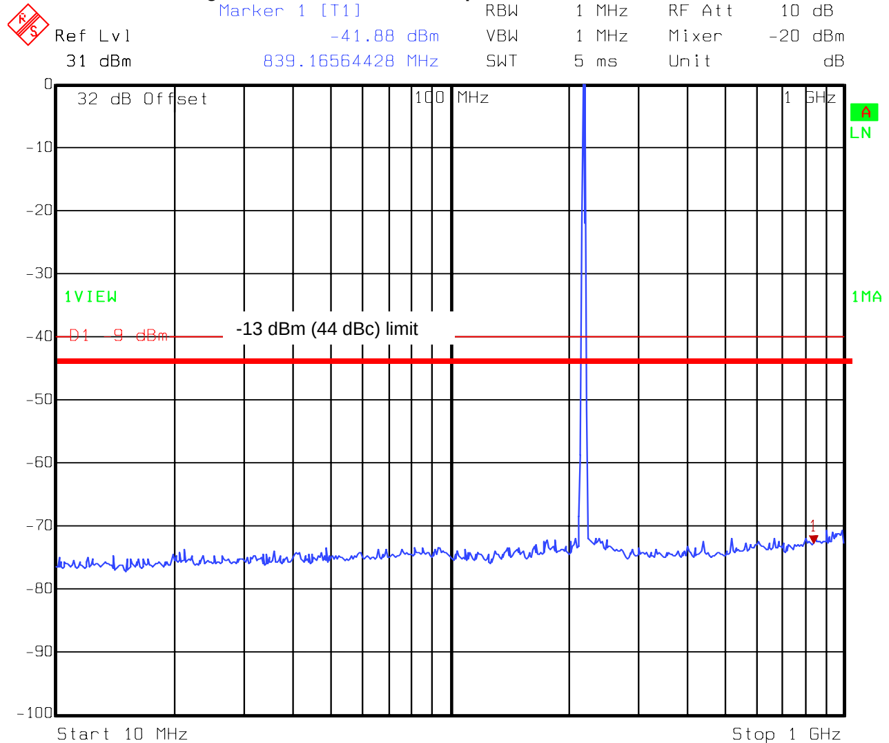
Figure 4 Antenna Conducted Spurious – Low Channel - 10 MHz – 1 GHz
