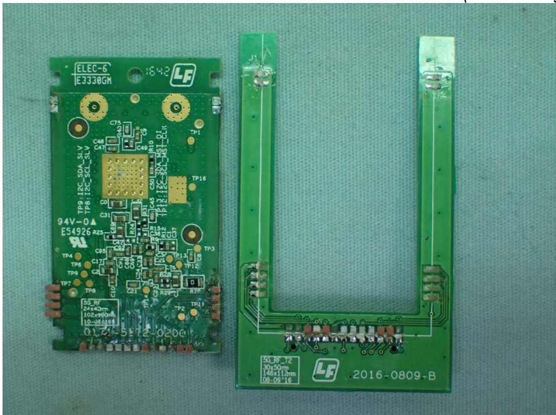
Figure 4 Internal View (Removed Jig Board)
