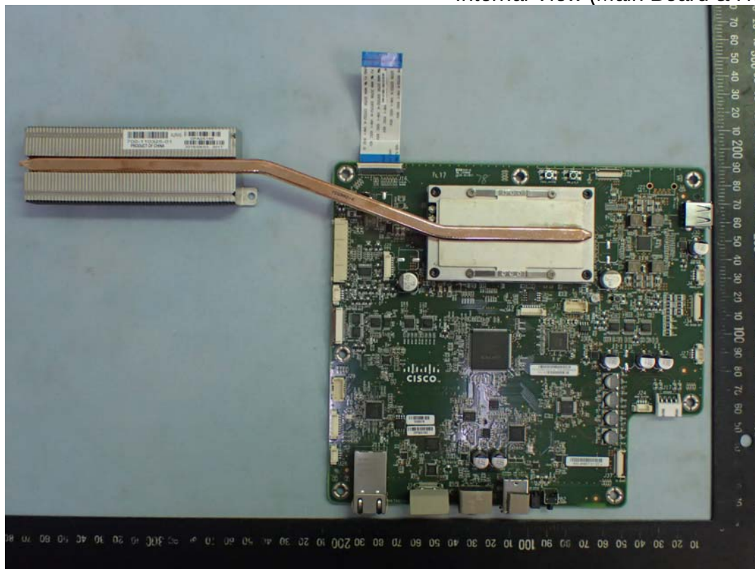
Figure 36 Internal View (Main Board & Heat Sink)
