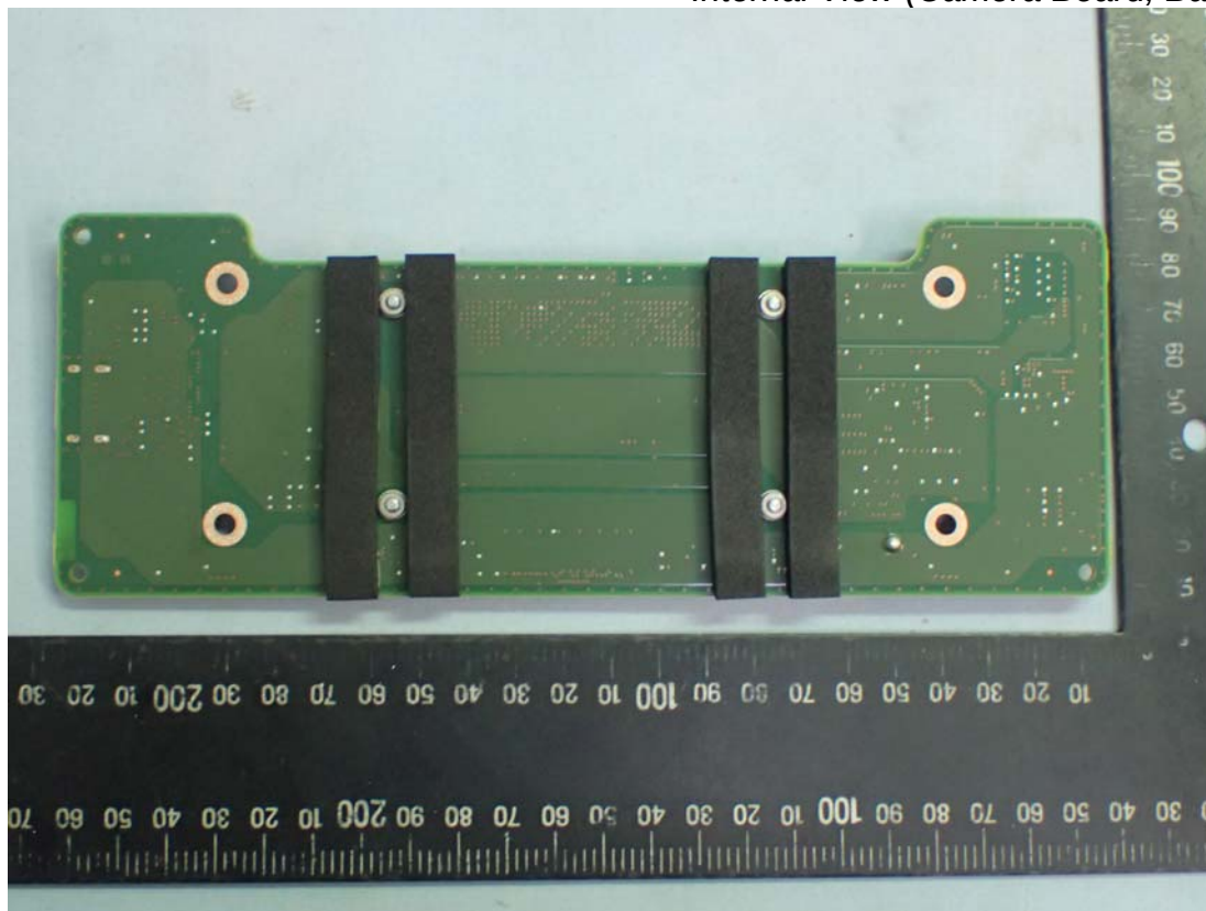
Figure 18 Internal View (Camera Board, Back View)
