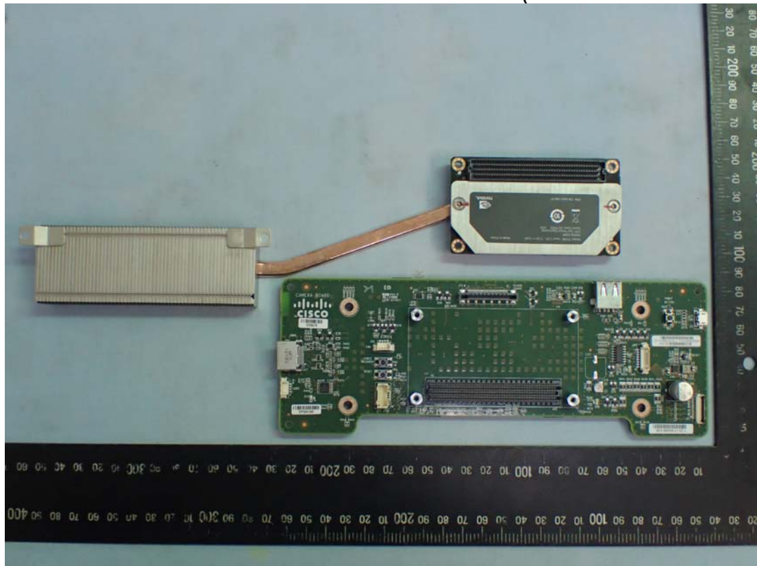
Figure 16 Internal View (RF Module and Camera Board)
