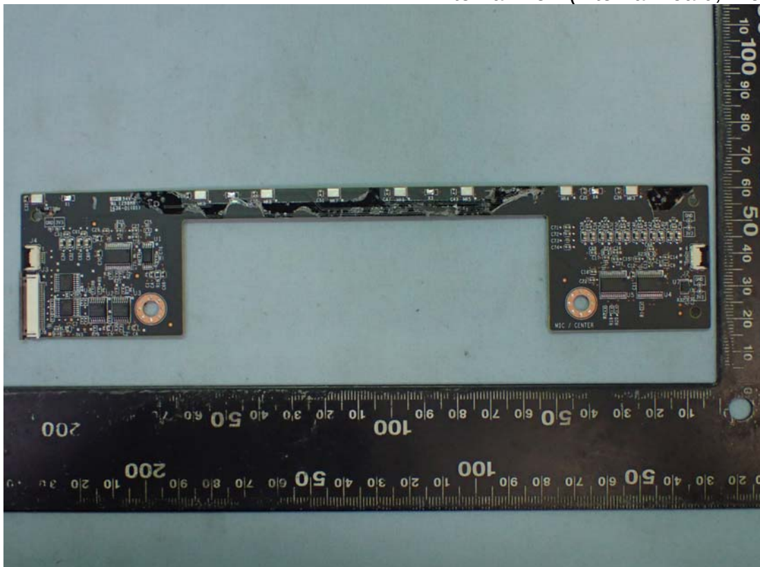
Figure 39 Internal View (Internal Board, Front View)
