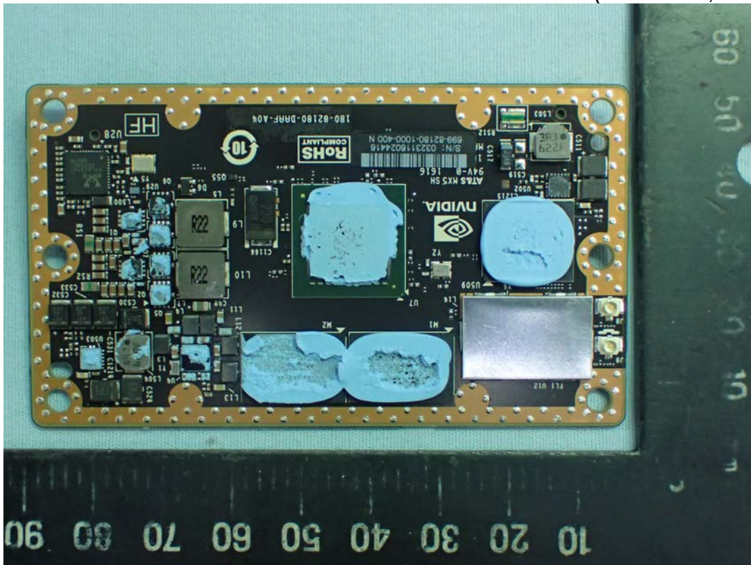
Figure 22 Internal View (RF Module, Front View)
