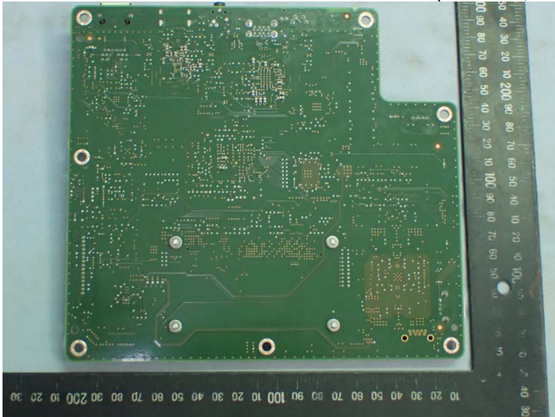
Figure 38 Internal View (Main Board, Back View)
