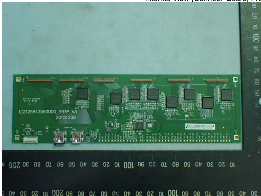
Figure 31 Internal View (Connect Board, Front View)
