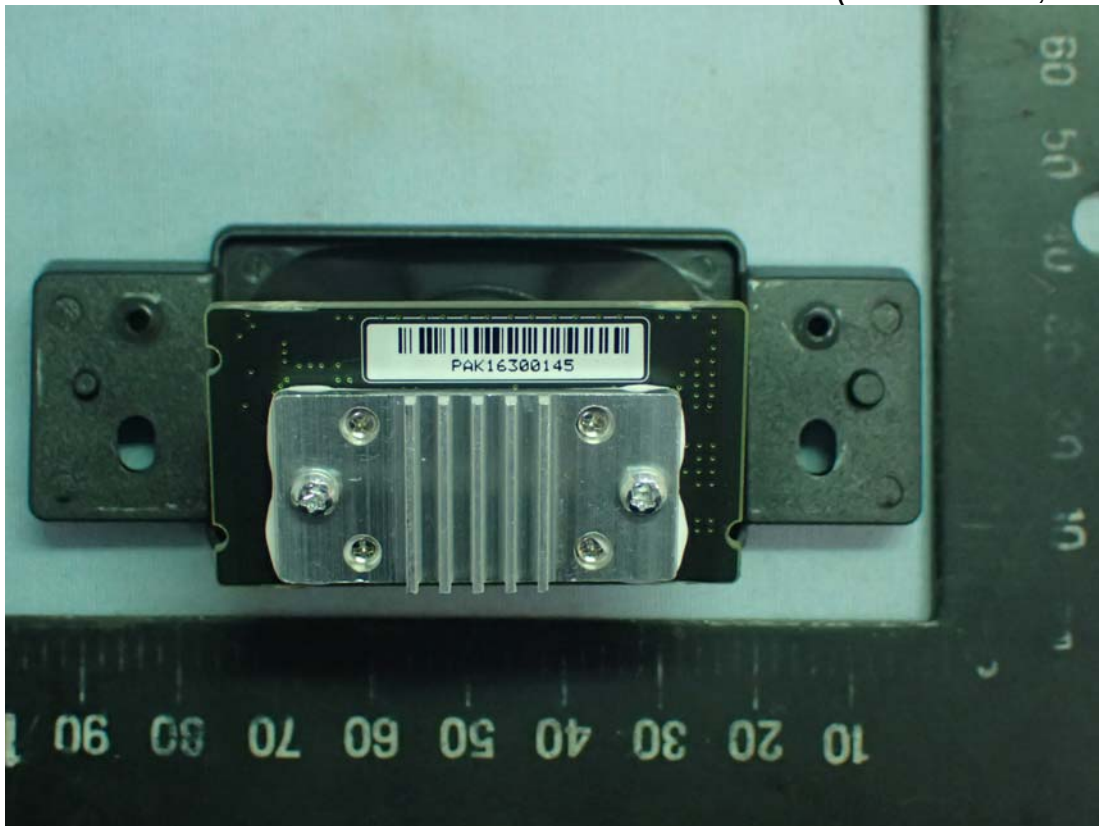
Figure 34 Internal View (Camera View, Back View)
