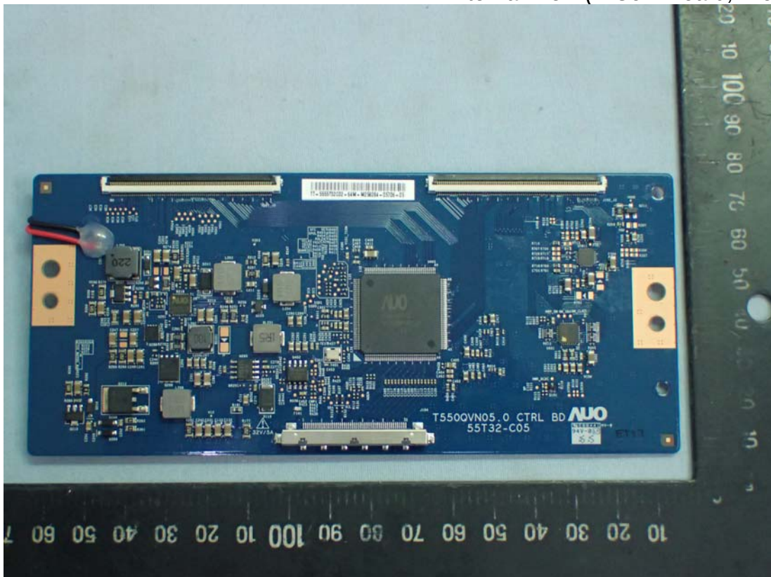
Figure 23 Internal View (T-Com Board, Front View)
