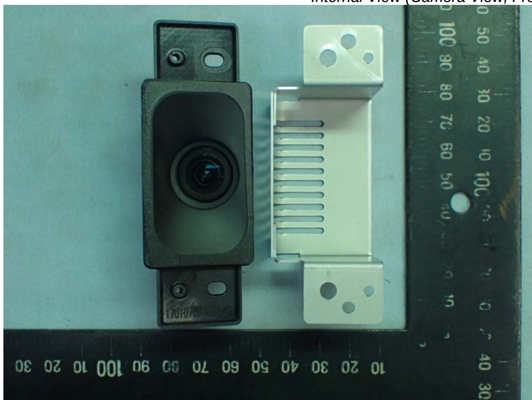
Figure 33 Internal View (Camera View, Front View)
