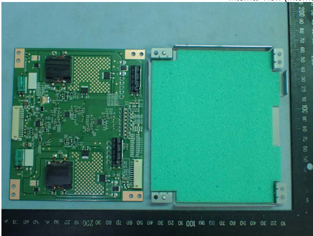
Figure 28 Internal View (Internal Board)
