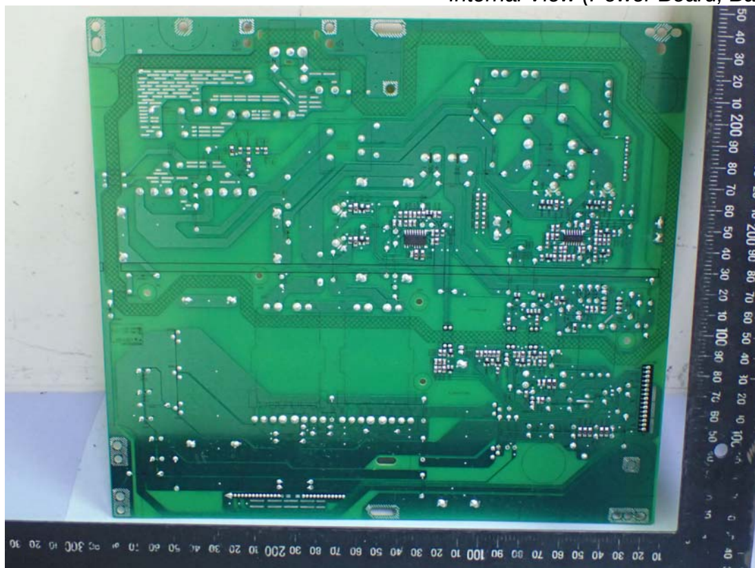
Figure 11 Internal View (Power Board, Back View)
