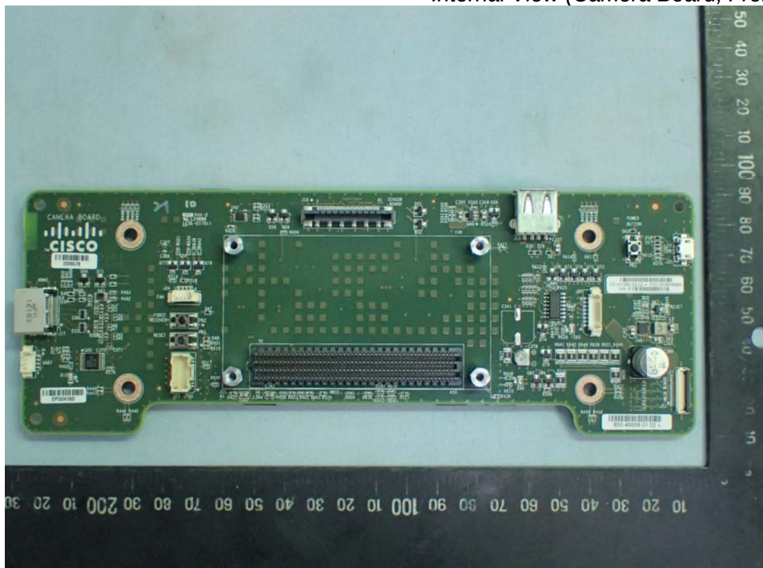
Figure 17 Internal View (Camera Board, Front View)
