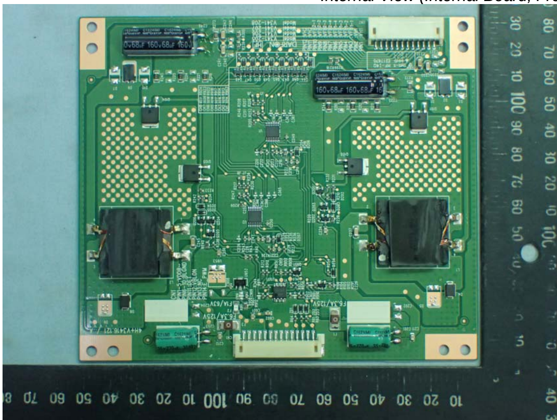
Figure 29 Internal View (Internal Board, Front View)
