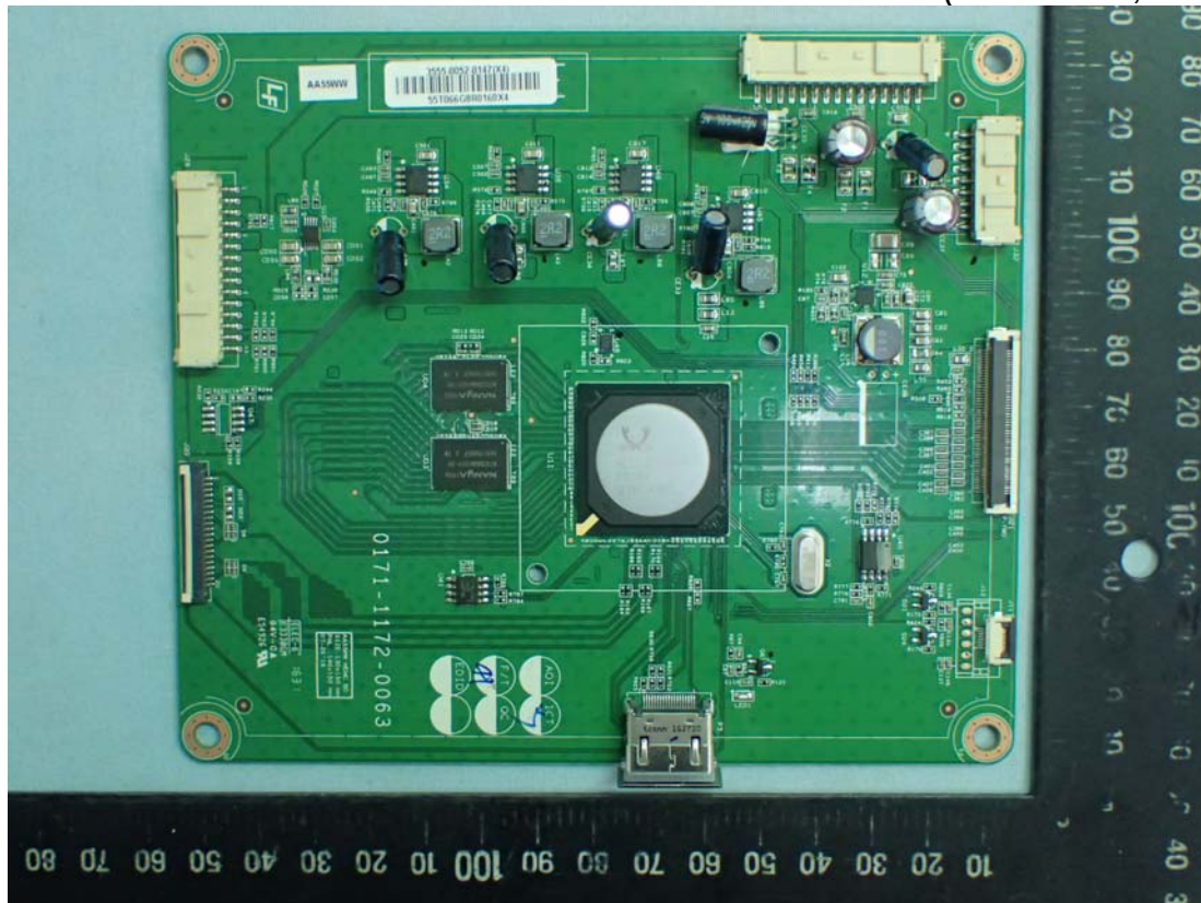
Figure 12 Internal View (Main Board, Front View)
