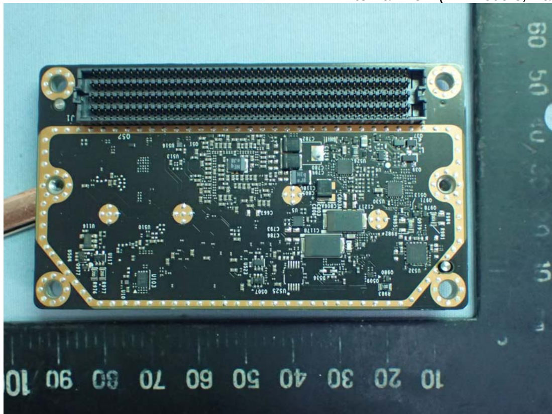
Figure 21 Internal View (RF Module, Back View)
