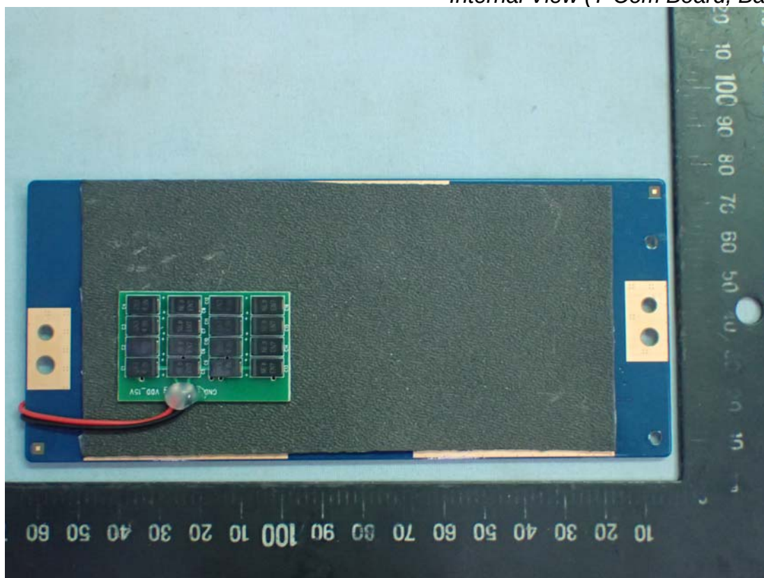
Figure 24 Internal View (T-Com Board, Back View)
