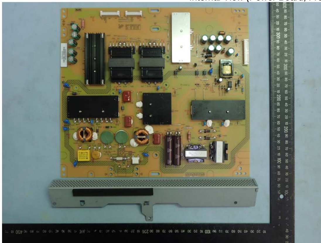
Figure 10 Internal View (Power Board, Front View)
