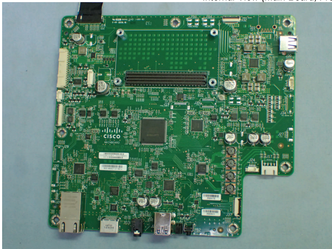
Figure 28 Internal View (Main Board, Front View)
