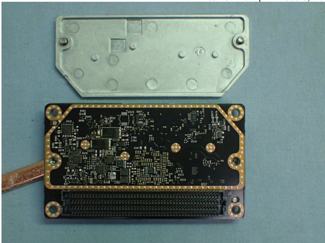
Figure 31 Internal View (RF Module, Back View)
