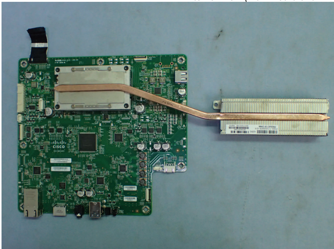
Figure 27 Internal View (Main Board and RF Module)
