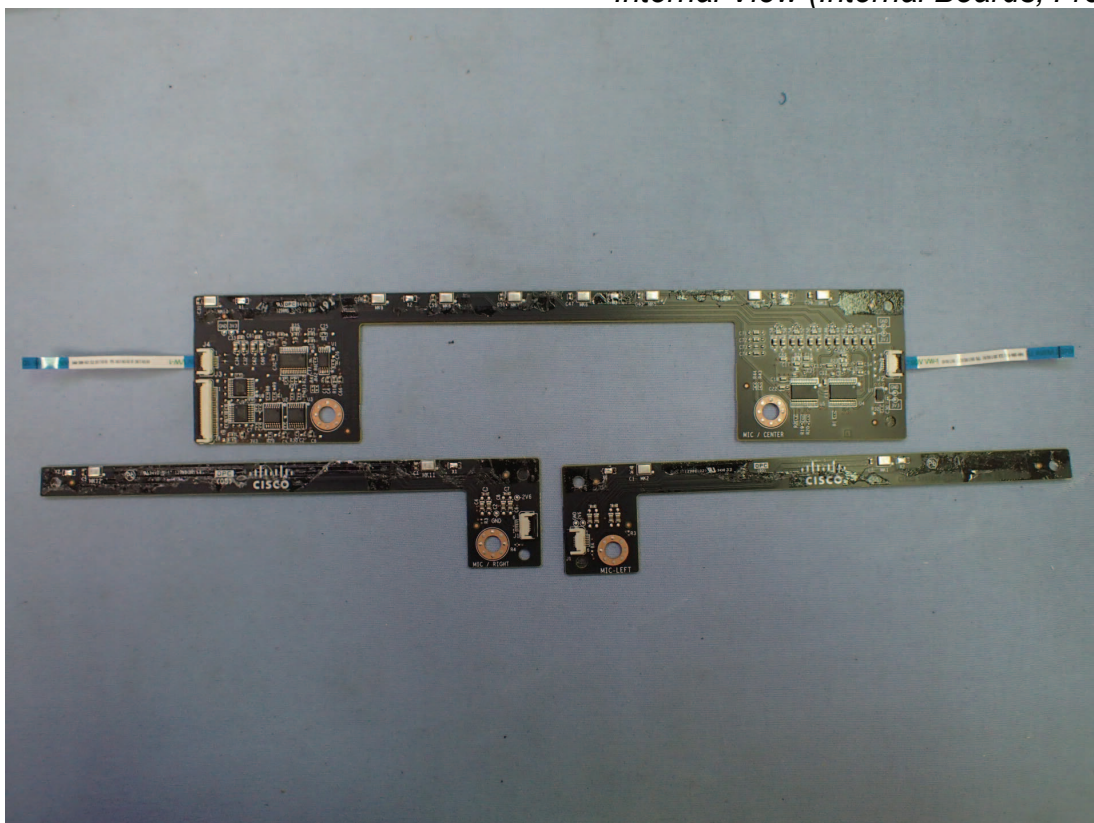
Figure 37 Internal View (Internal Boards, Front View)
