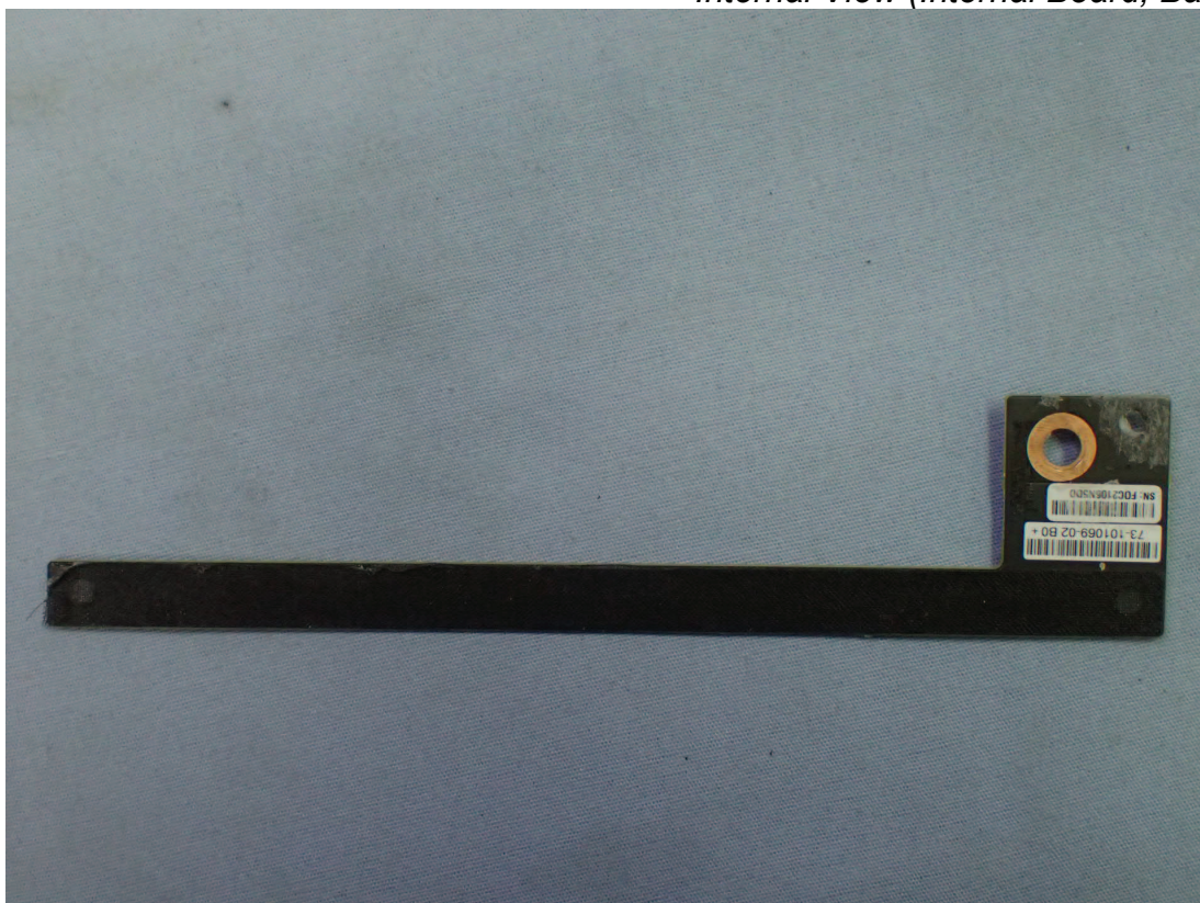
Figure 39 Internal View (Internal Board, Back View)
