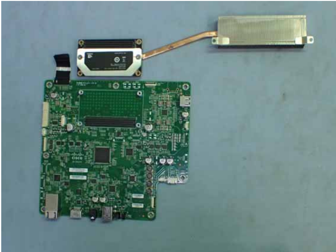
Figure 23 Internal View (Main Board)
