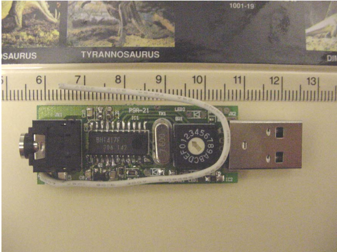
Interior top of PCB showing antenna.
