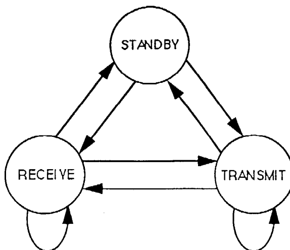
Figure 7 - Radio Modes
