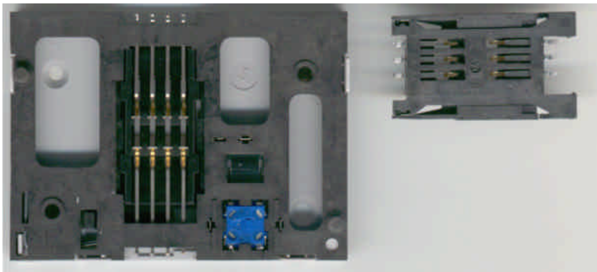
Bottom view of Smart and Sam card connectors
