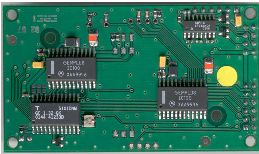
Bottom view (without Sam card connector) Components side.
