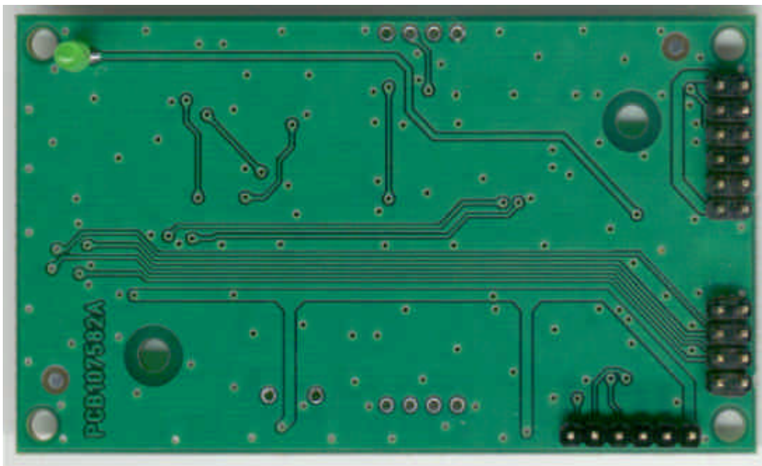
Top view (without smart card connector)
