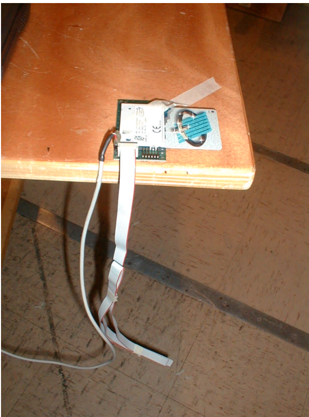
Detailed view of EUT with its cables
