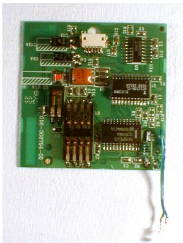
Internal board, Component side
