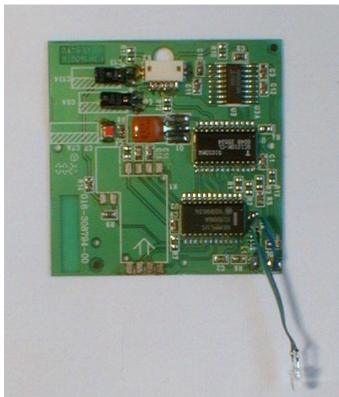
Internal board, Component side, smart card connector removed
