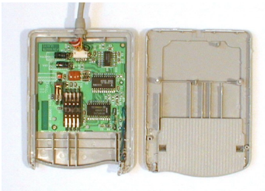
Internal view, Box opened
