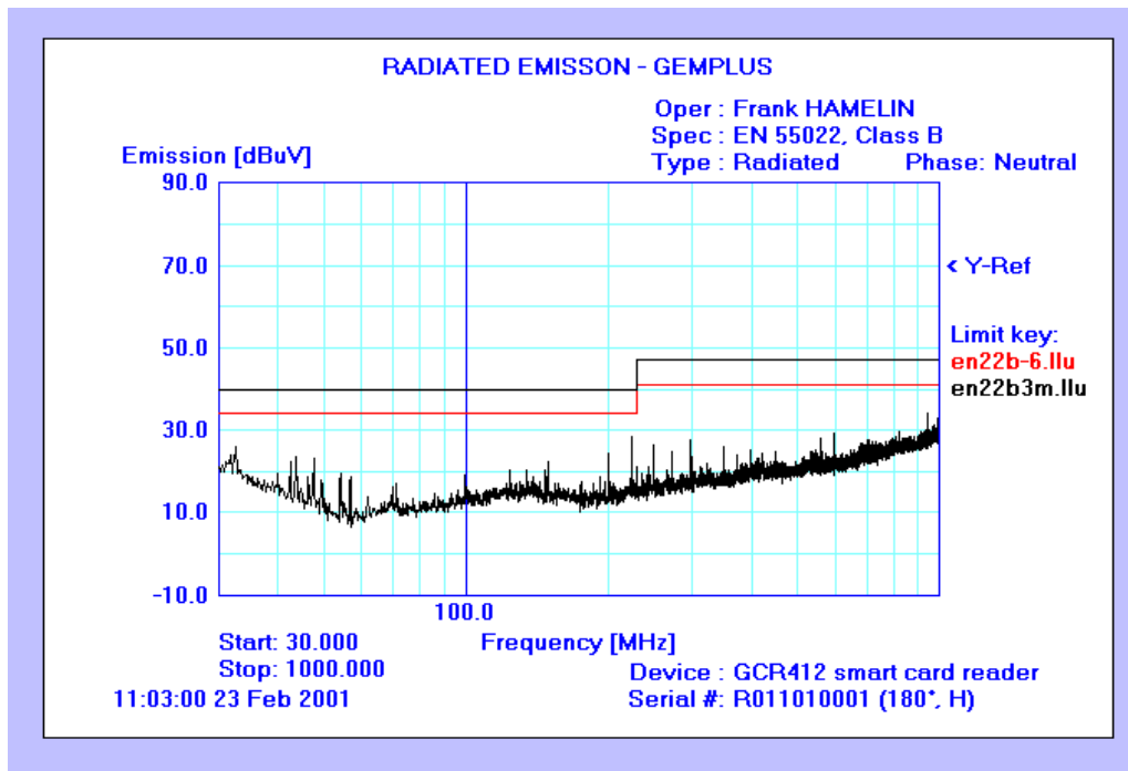
Graph abstract - 30-1000MHz
