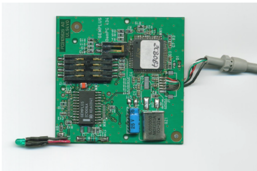
Internal board, Component side
