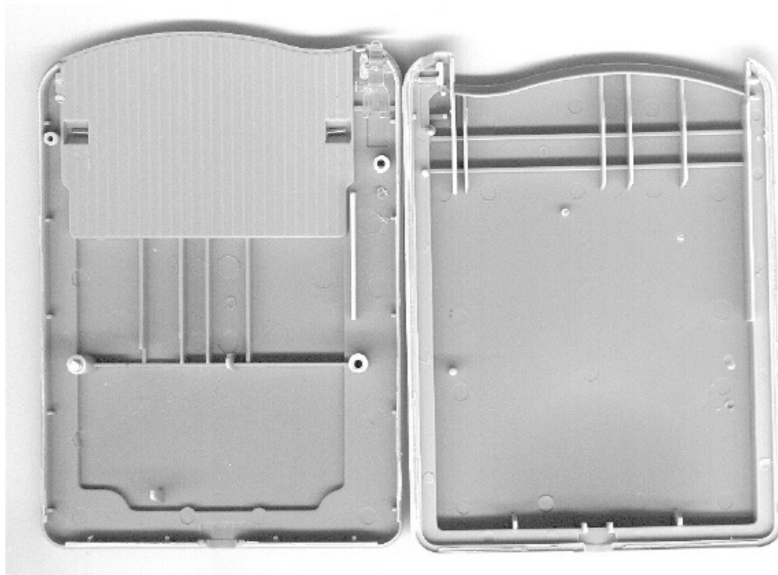
Internal view, Box opened Without internal board
