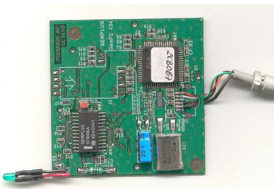
Internal board, Component side, smart card connector removed
