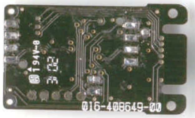
Internal board, smart card connector removed
