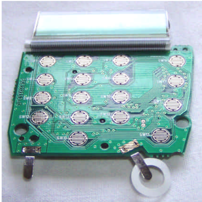
keypad side
